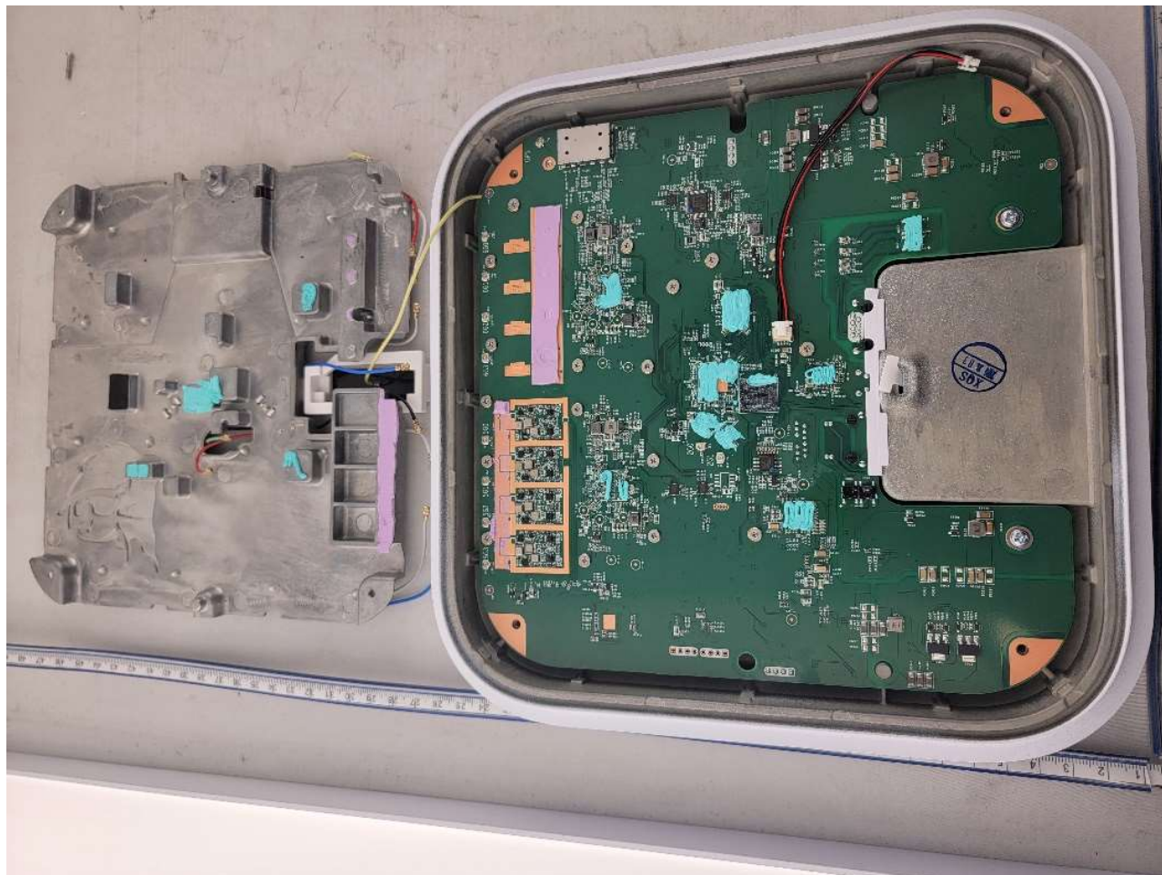
Photograph 2: Antenna Board Removed Showing PCB Placement
