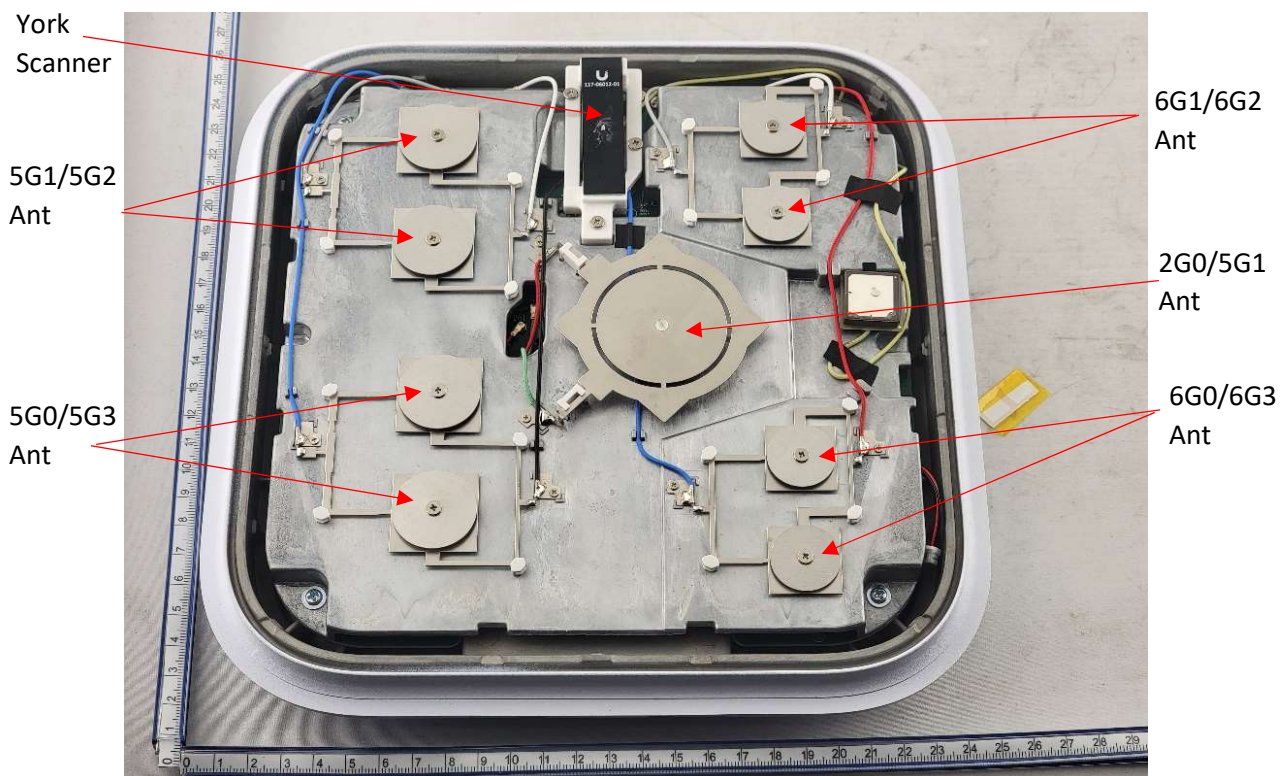
Photograph 1: Front Cover Off Showing Front of Antenna Board
