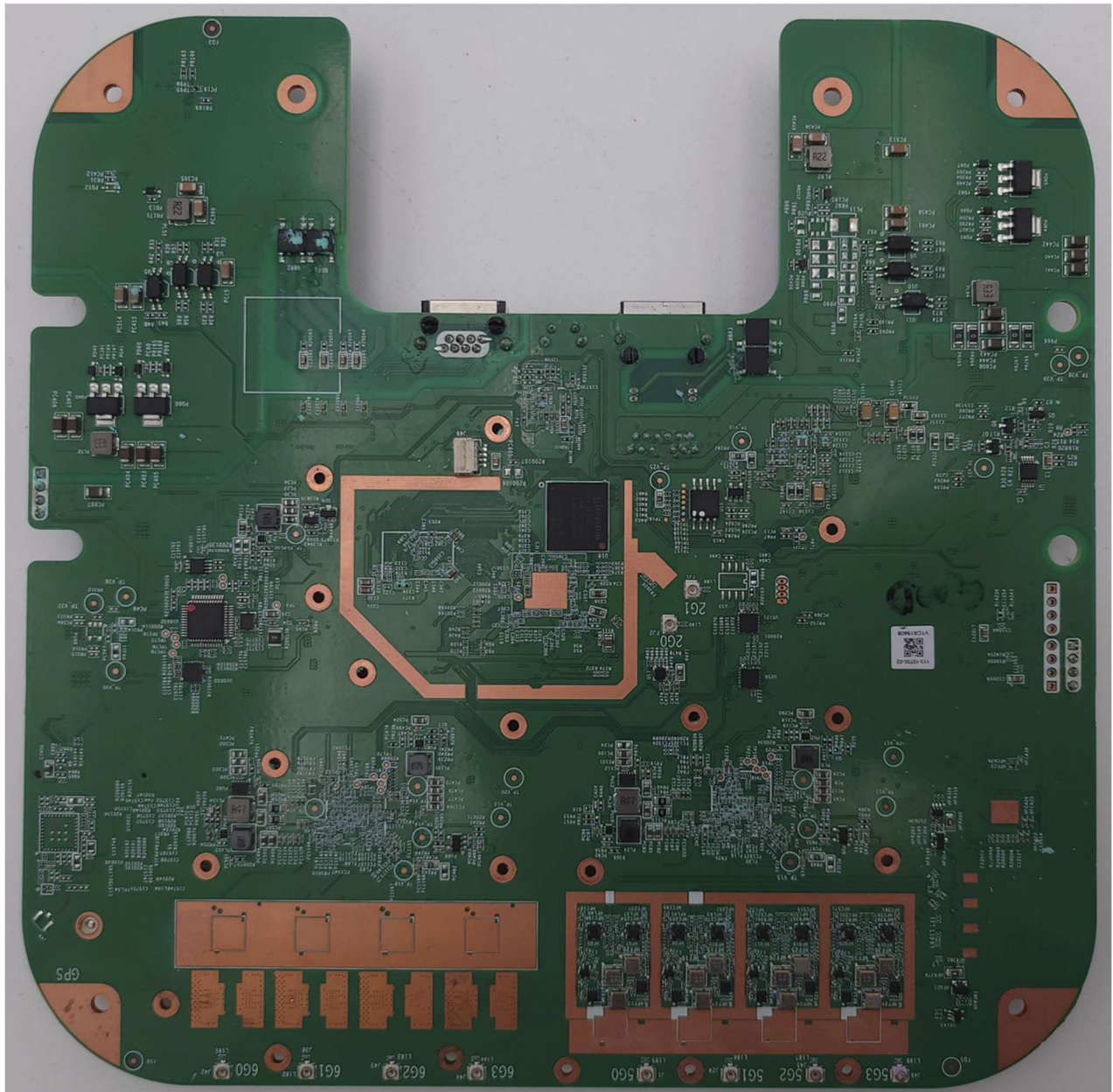
Photograph 2: Bottom Side Of PCB
