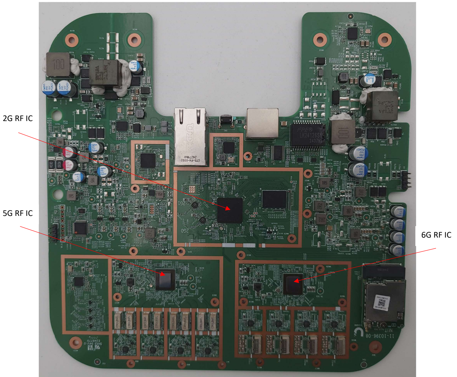
Photograph 1: Top Side Of PCB
