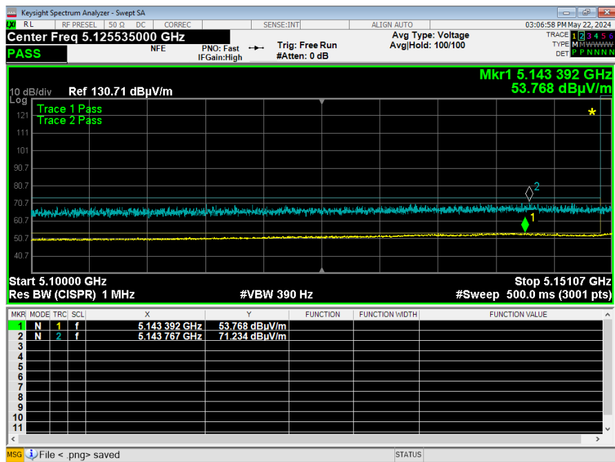
Graph 3: Band Edge Low ax Mode 20 MHz
