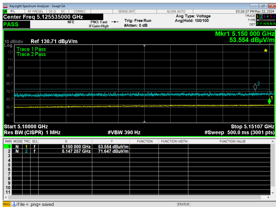
Graph 6: Band Edge High ax Mode 40 MHz
