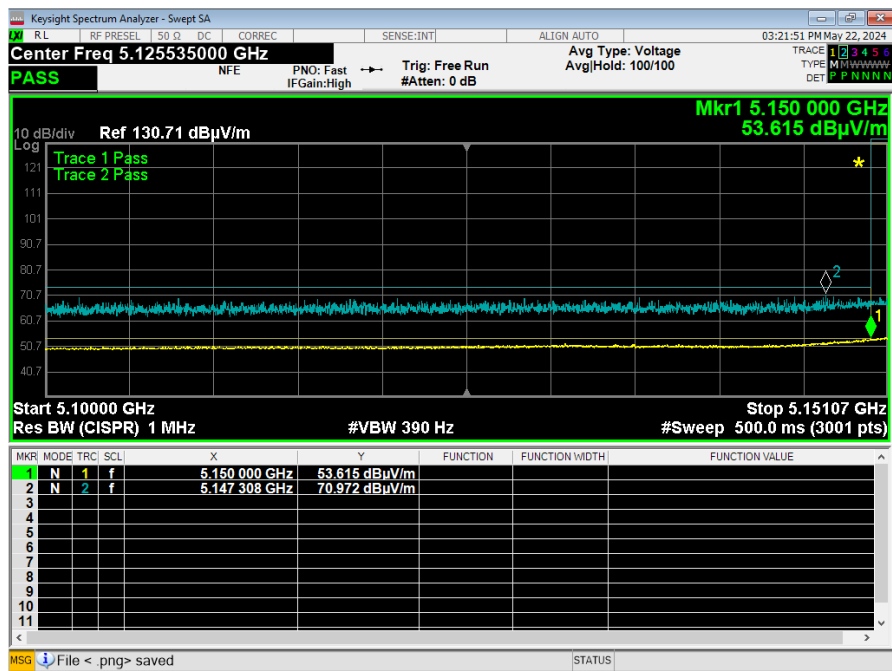
Graph 5: Band Edge Low ax Mode 40 MHz
