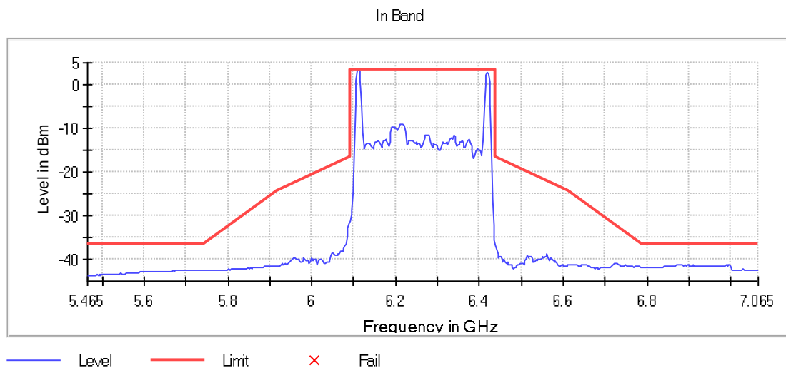
Figure 14: 3265 320MHz RU Vérification - Edge
