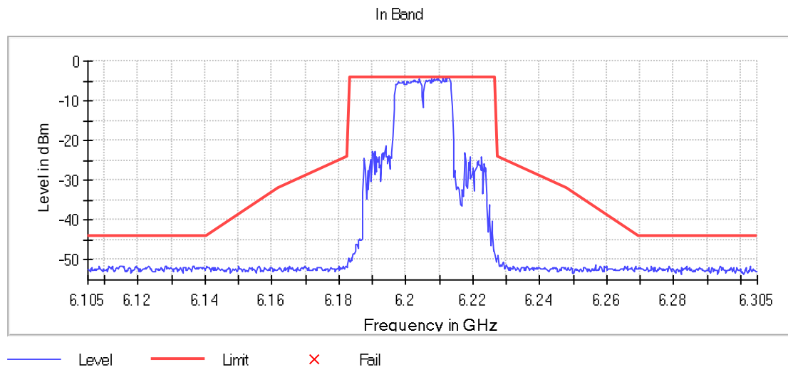
Figure 7: 6205 40MHz RU Vérification - Center
