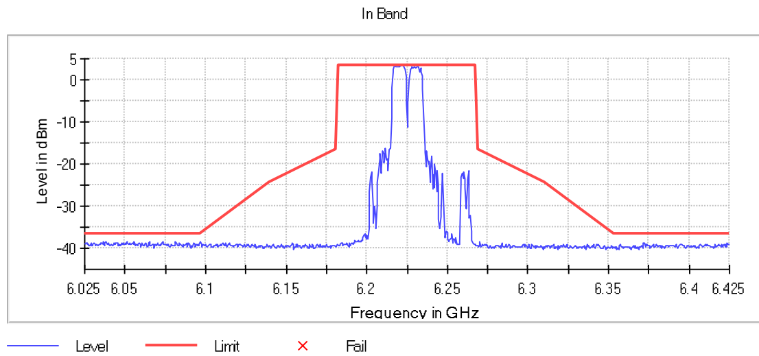
Figure 9: 6225 80MHz RU Vérification - Center
