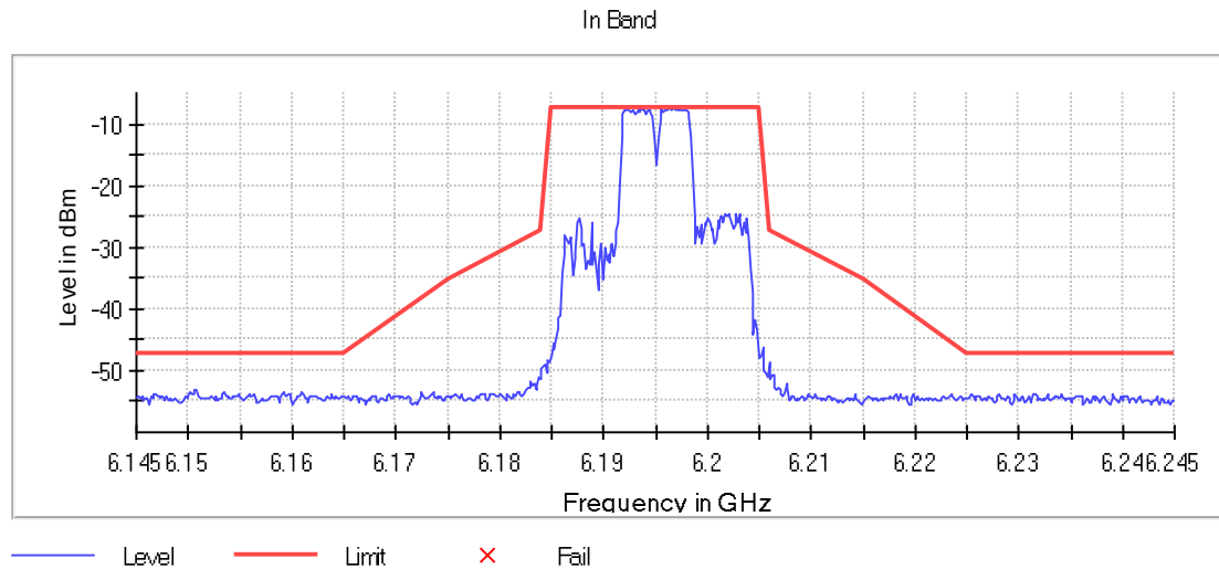
Figure 5: 6195 20MHz RU Vérification - Center
