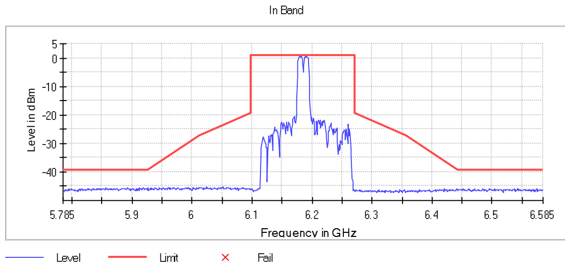
Figure 11: 6185 160MHz RU Vérification - Center
