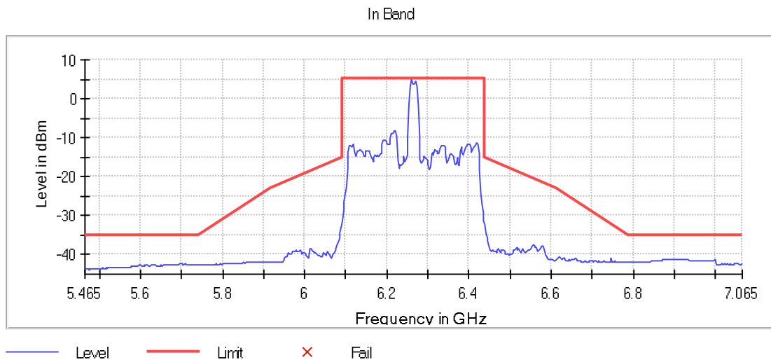
Figure 13: 6265 320MHz RU Vérification - Center
