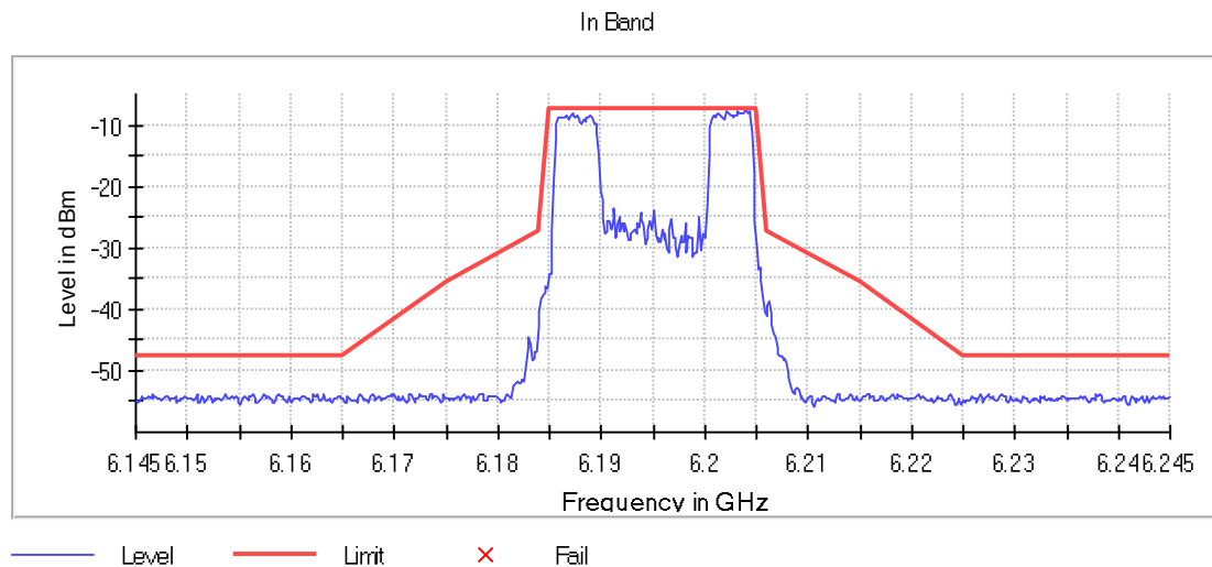
Figure 6: 6195 20MHz RU Vérification - Edge
