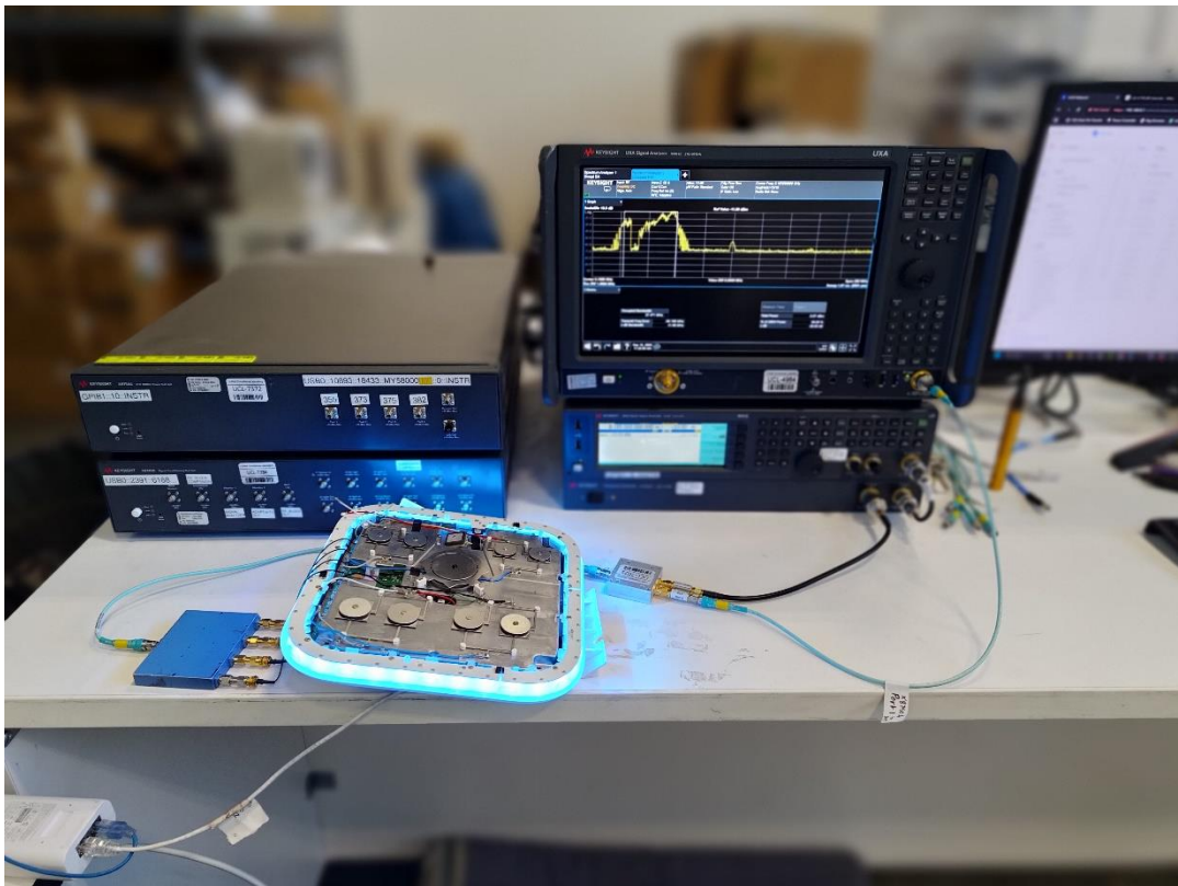
Photograph 8: View Test Set Up CBP
