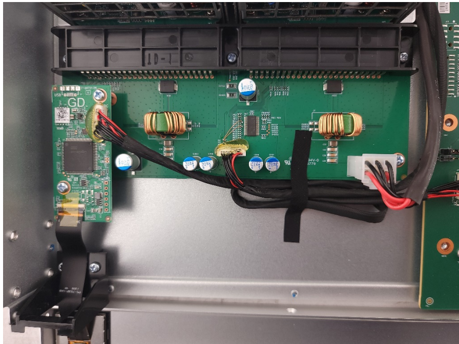
Photograph 10: Internal View of DUT Power PCB
