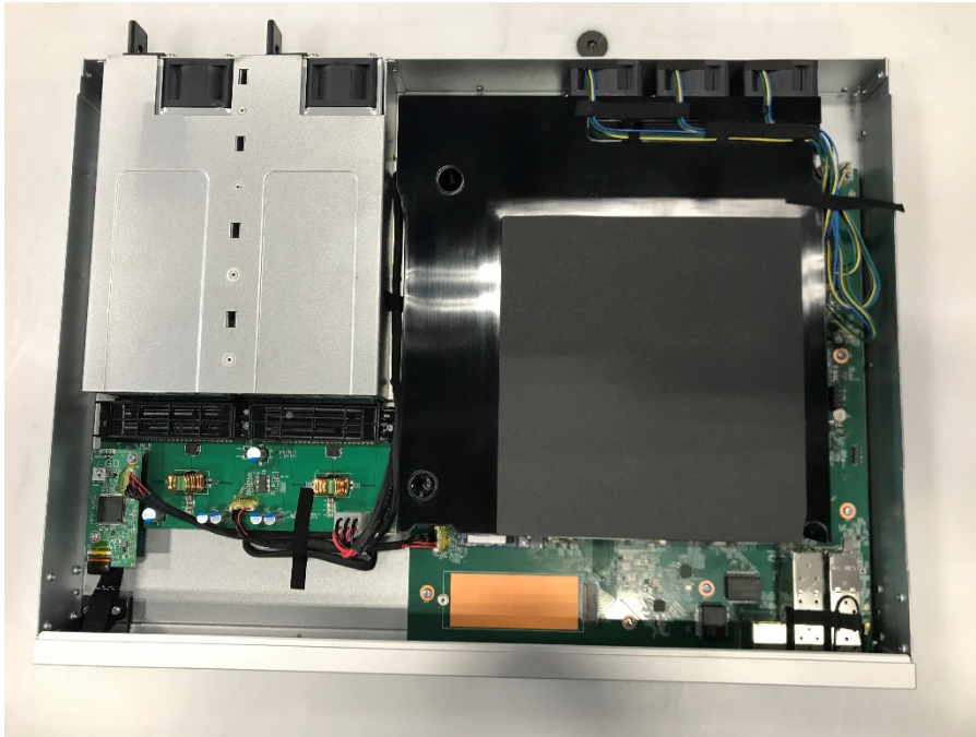
Photograph 1: Internal View of DUT With Top Cover Off
