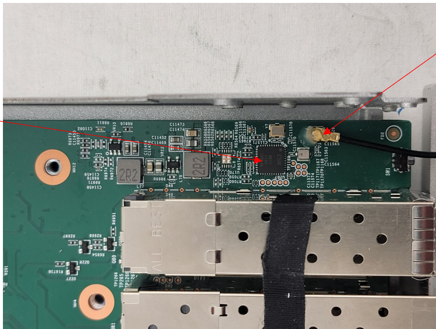
Photograph 4: Internal View of DUT Showing Bluetooth
