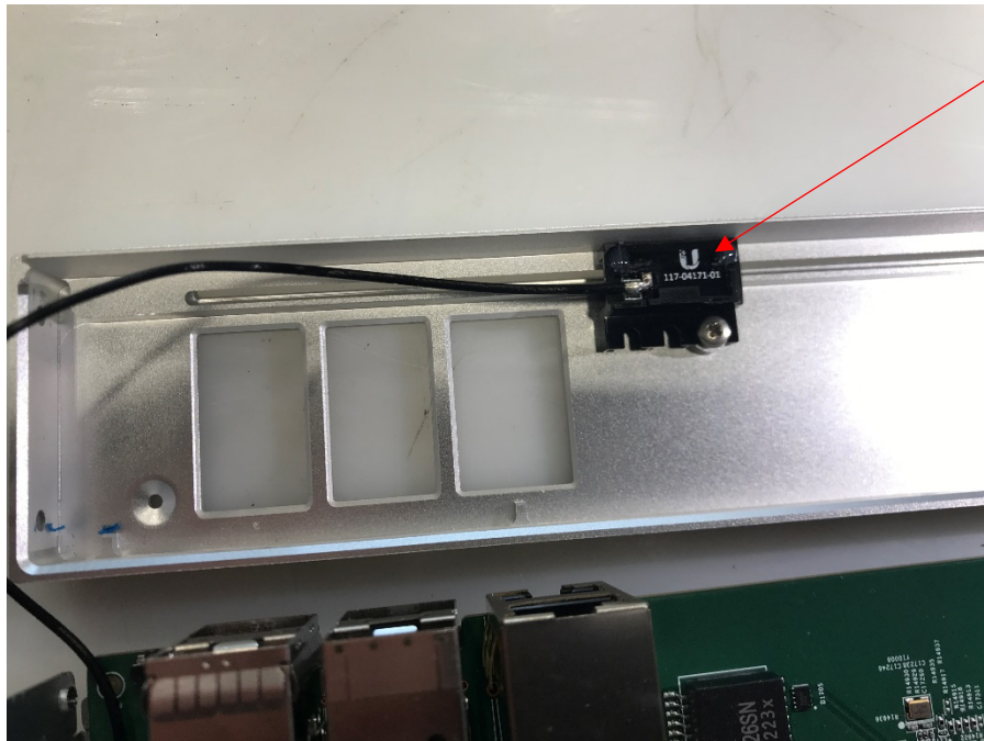
Photograph 5: Bluetooth Antenna Placement
