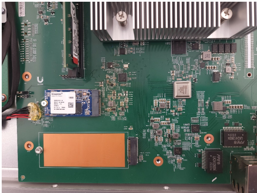
Photograph 7: Main PCB Close Up Top Right
