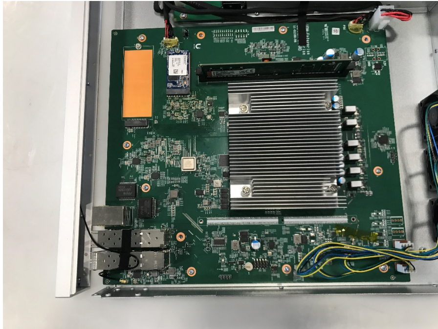
Photograph 3: Internal View of DUT Main PCB
