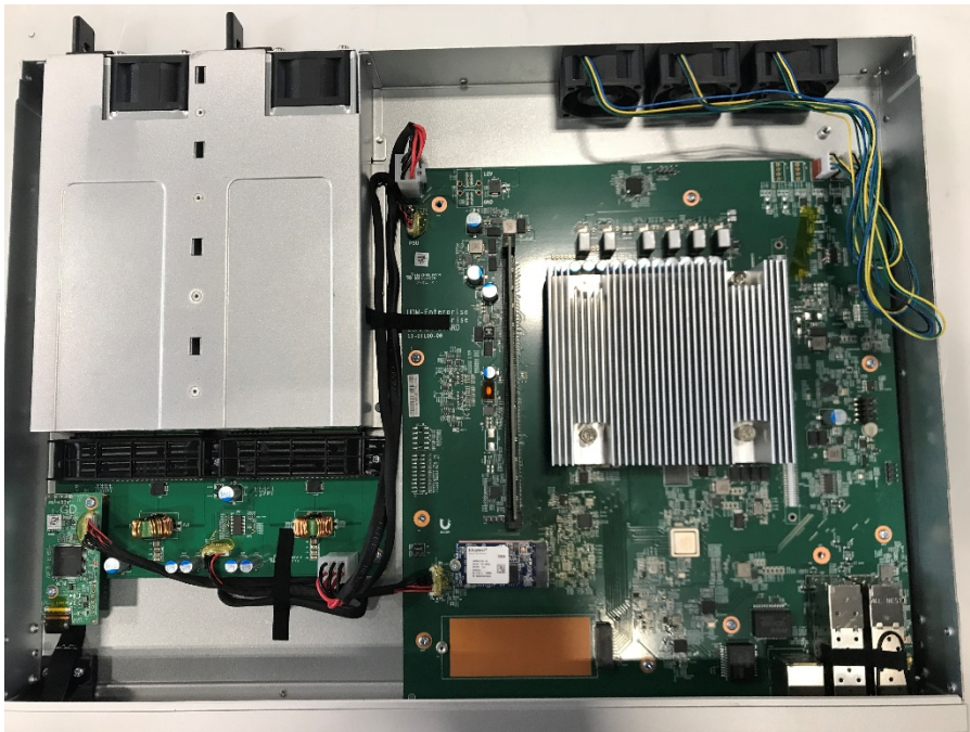
Photograph 2: Internal View of DUT With Plastic Cover Off
