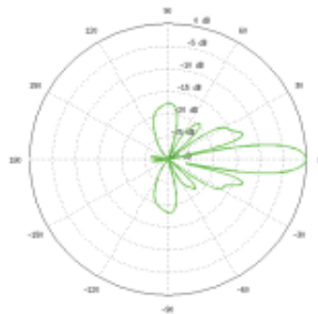
Vertical Azimuth
