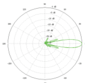
Horizontal Azimuth
