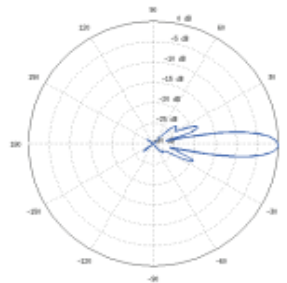
Vertical Elevation
