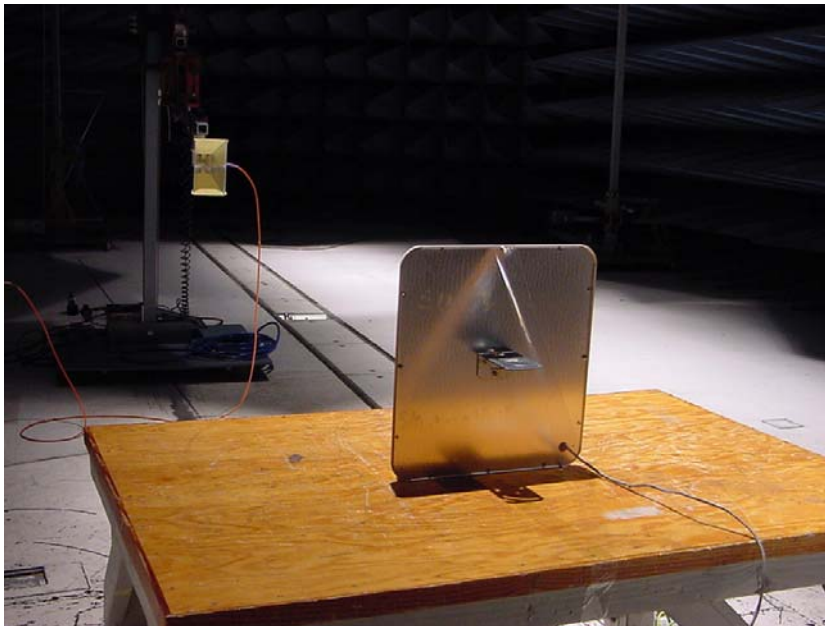
Photograph 9. Test Equipment and setup for various Radiated Measurements (Back)
