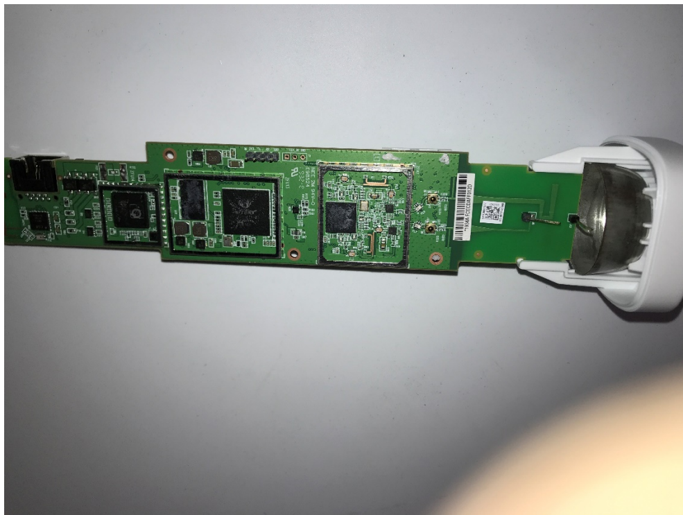
Photograph 5: Top View of the EUT – Heatsink & EMI Shield Removed
