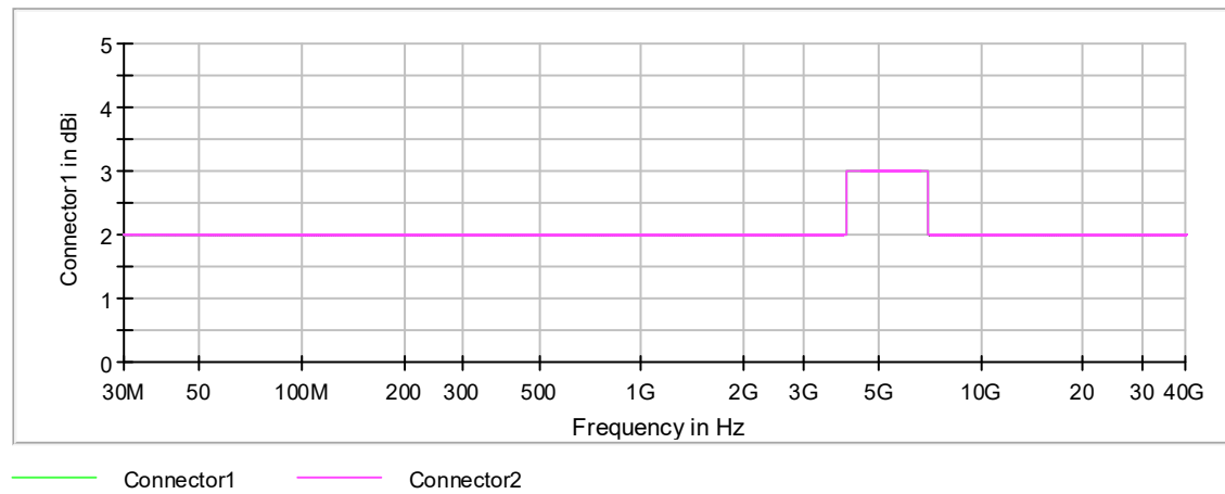
Gain
