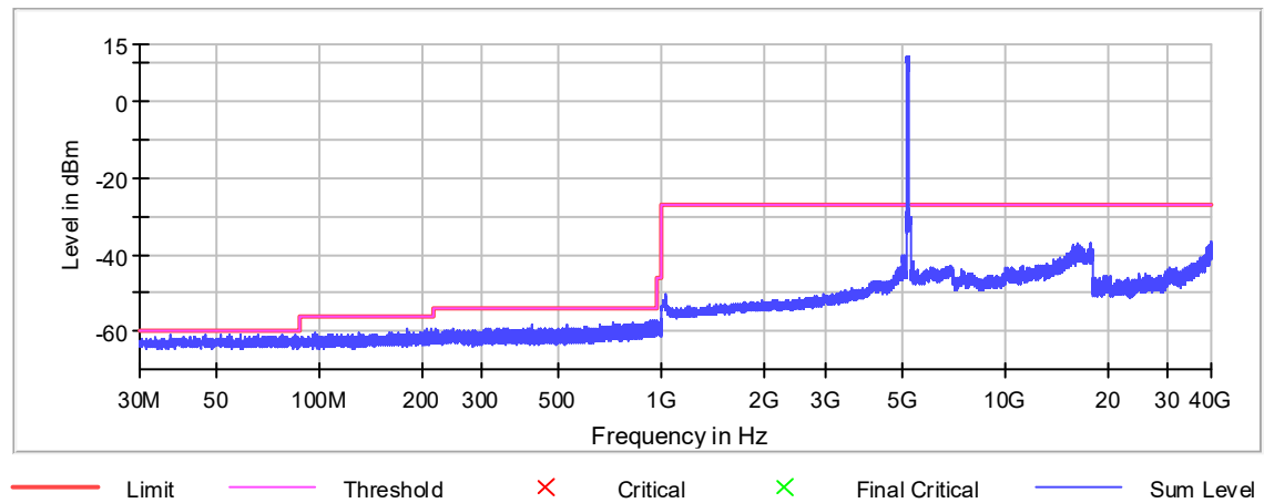
Spurious
