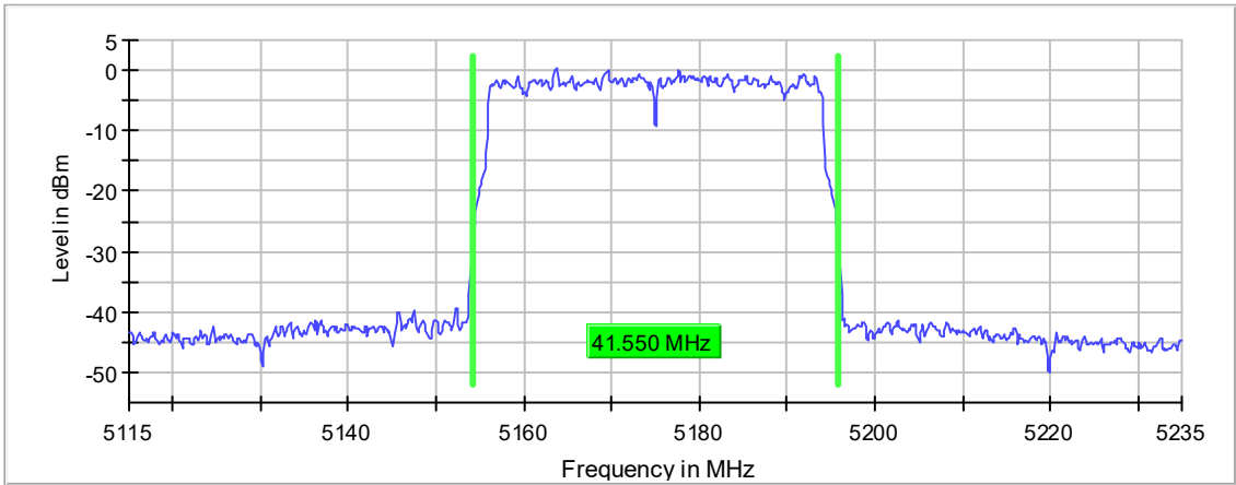
26 dB Bandwidth
