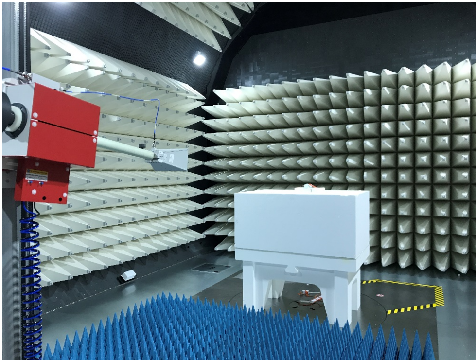
Photograph 4: Test Set Up Radiated Emissions 1-18 GHz
