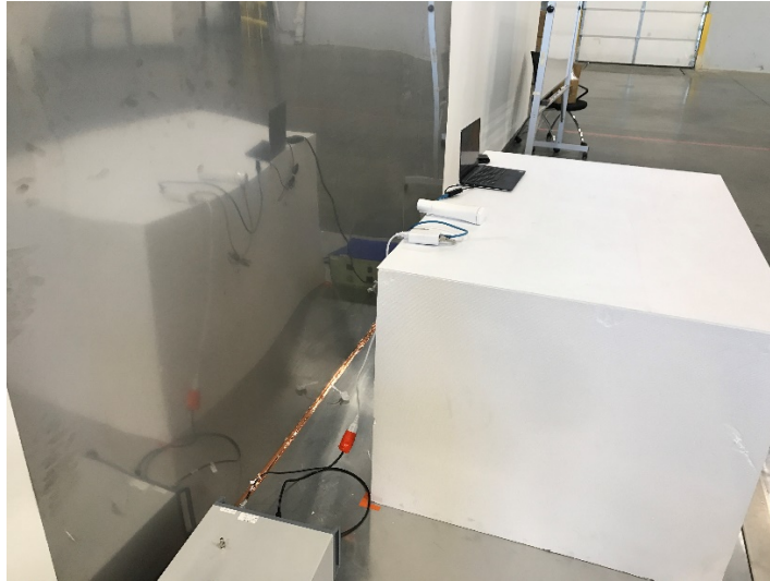
Photograph 1: Front View Test Set Up Conducted Emissions
