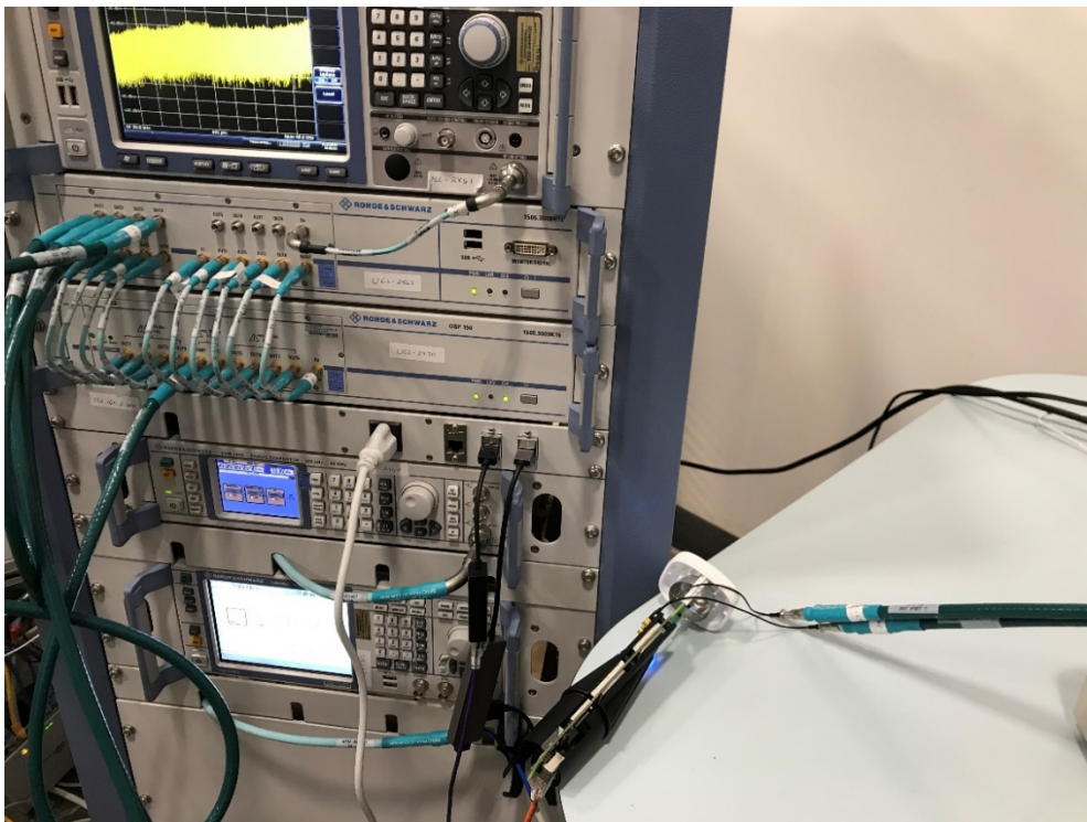
Photograph 6: Test Set Up Direct Connect
