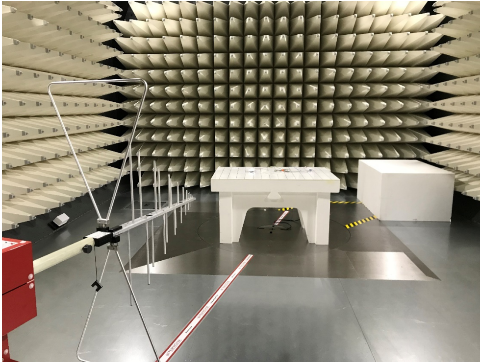
Photograph 3: Test Set Up Radiated Emissions 30-1000MHz
