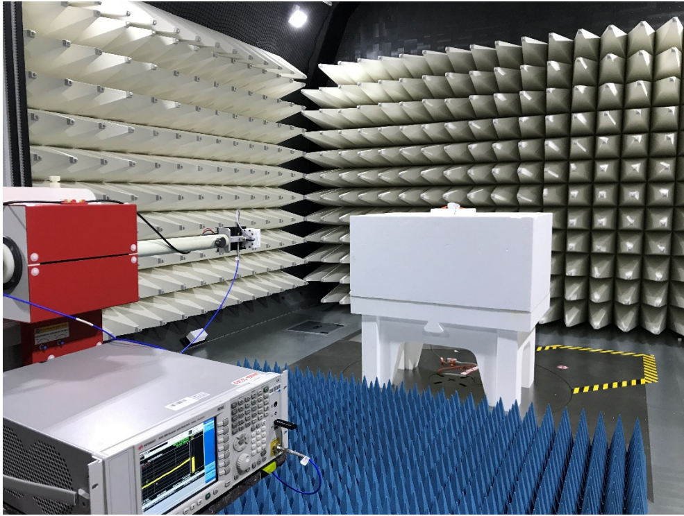
Photograph 5: Test Set Up Radiated Emissions 16-40GHz
