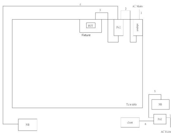
Test Setup Diagram – AC Line Conducted Emission Test (Beamforming)
