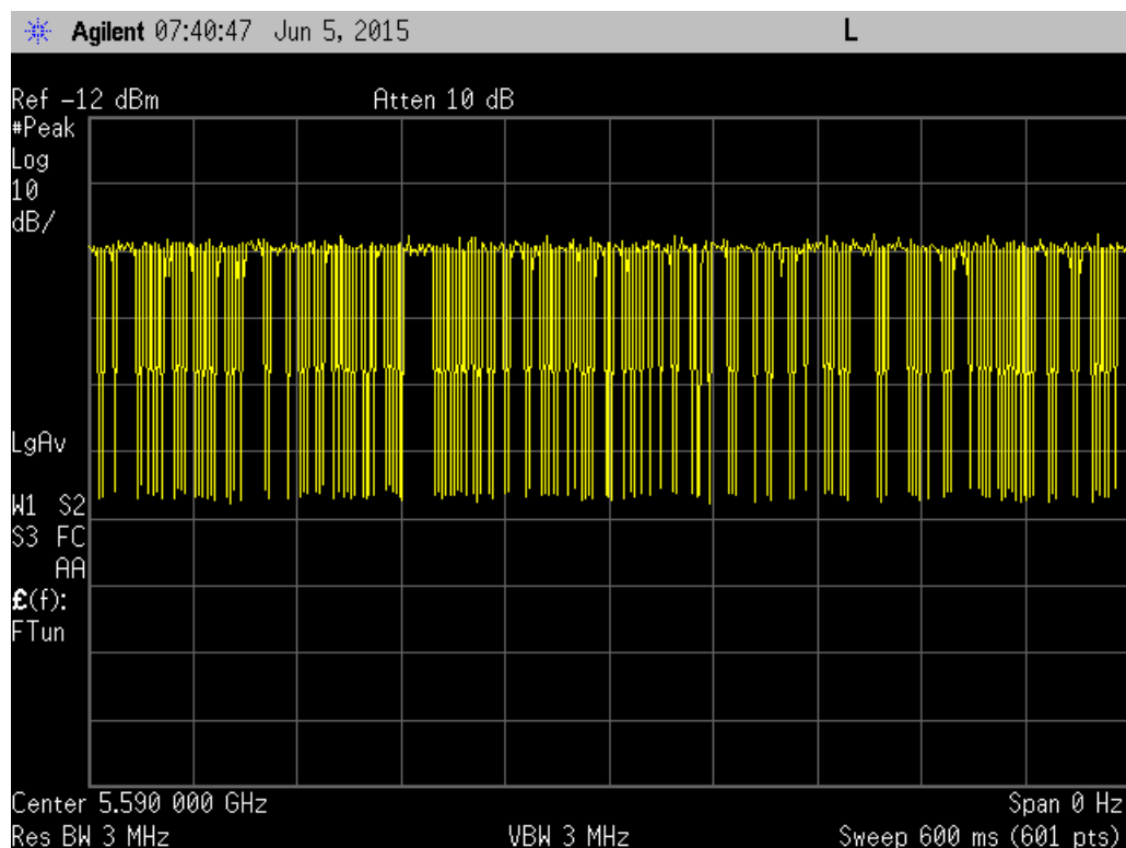
10MHz Bandwidth
