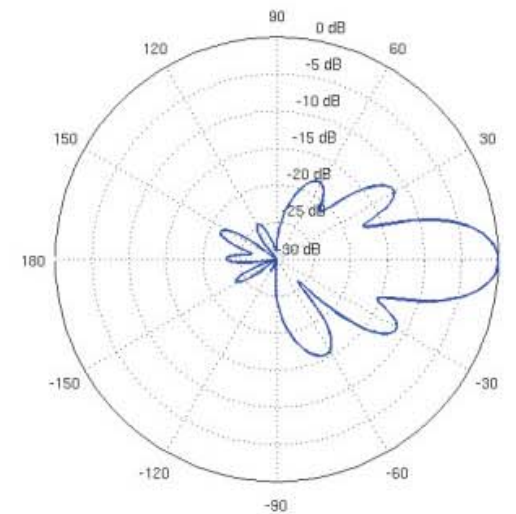
Horizontal Elevation
