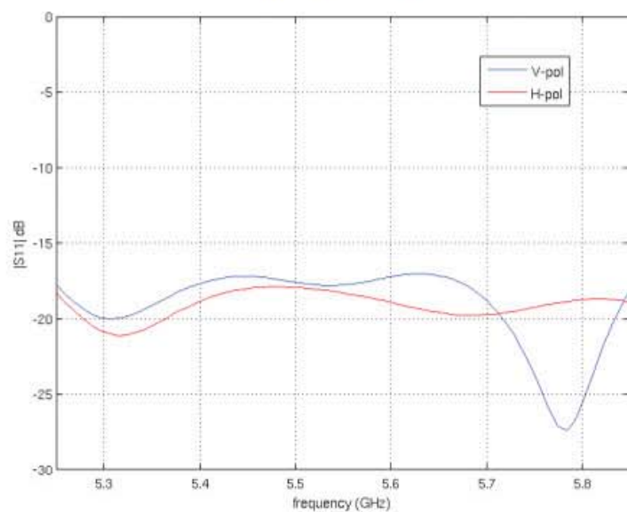
Return Loss
