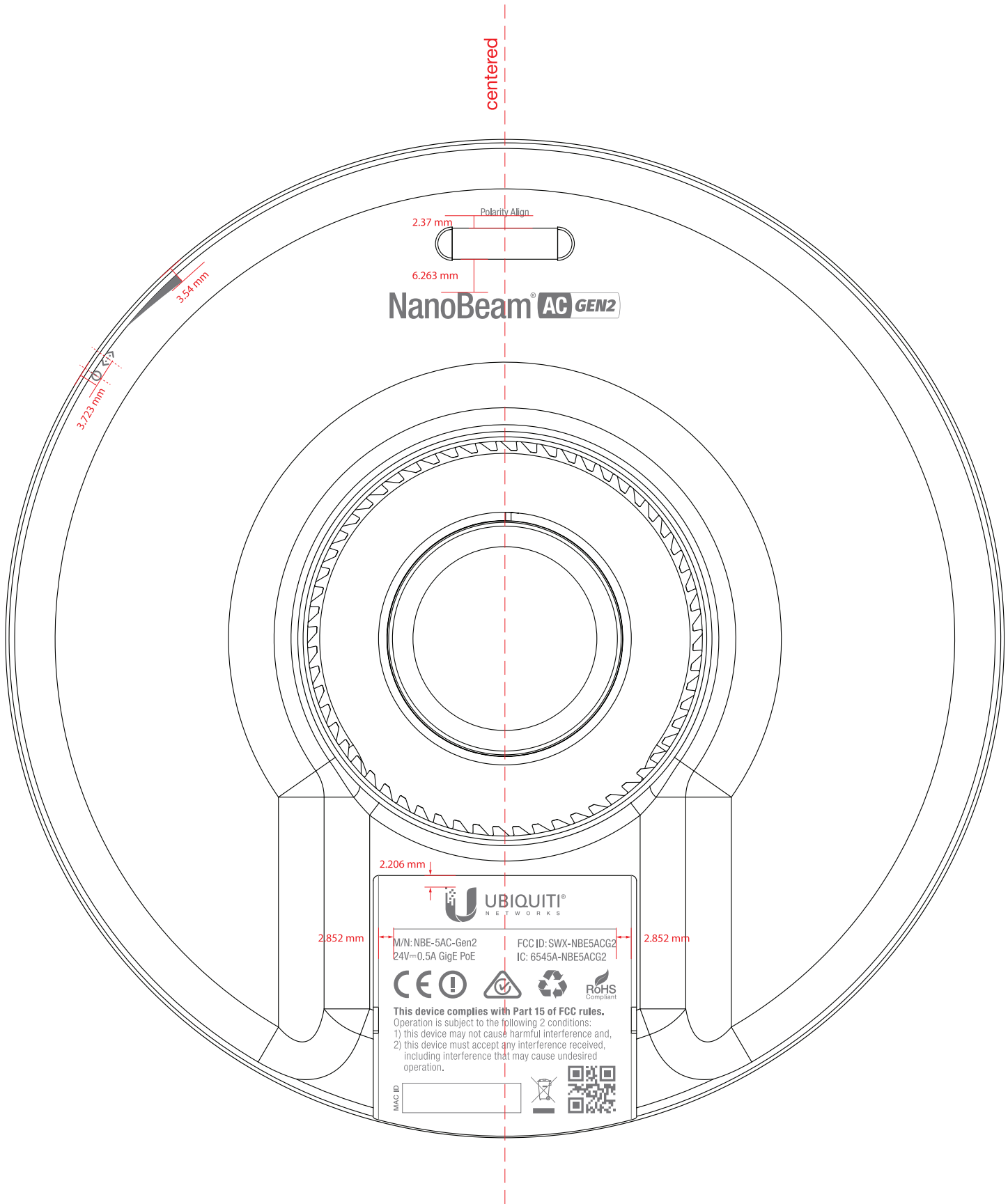
BOTTOM VIEW
