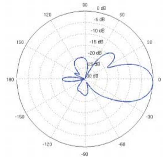
Vertical Elevation
