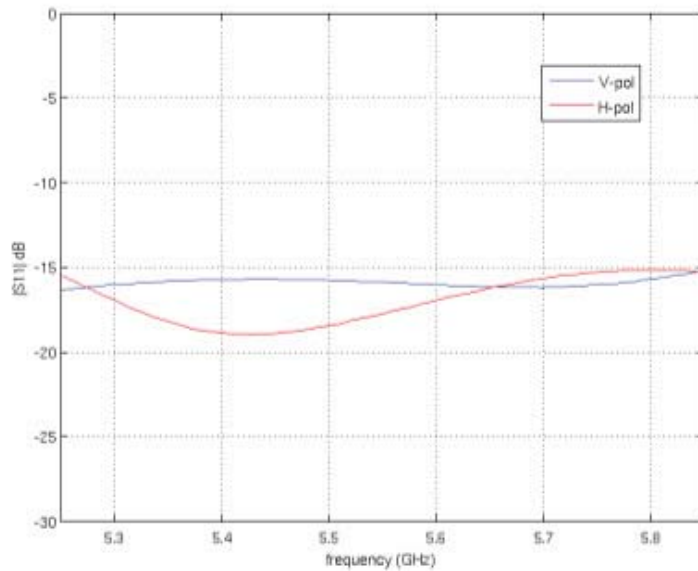
Return Loss
