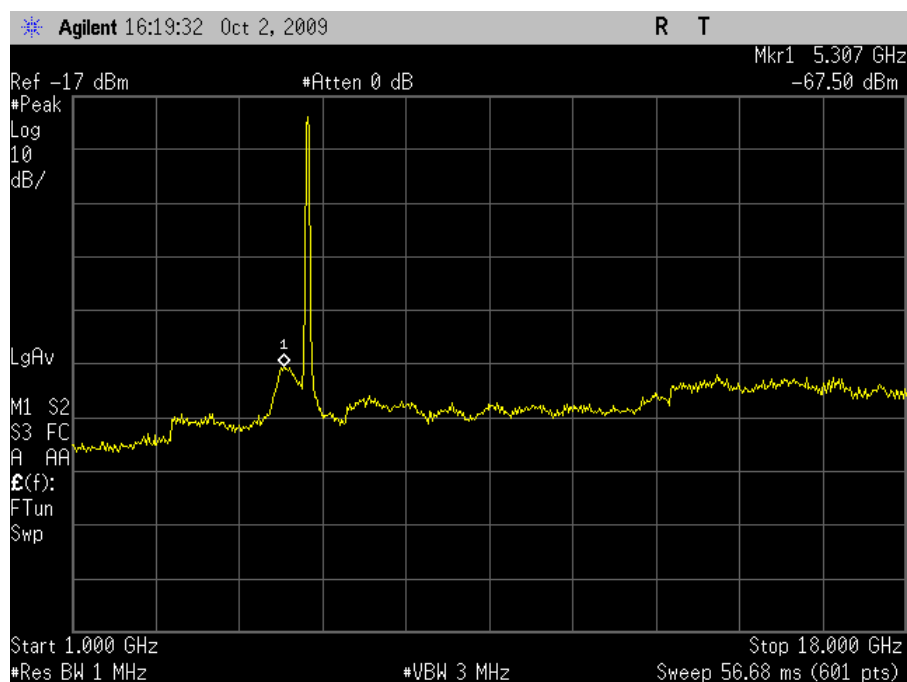
Plot 33. Radiated Spurious Emissions, Mid Channel, HT40 (Dish Antenna)
