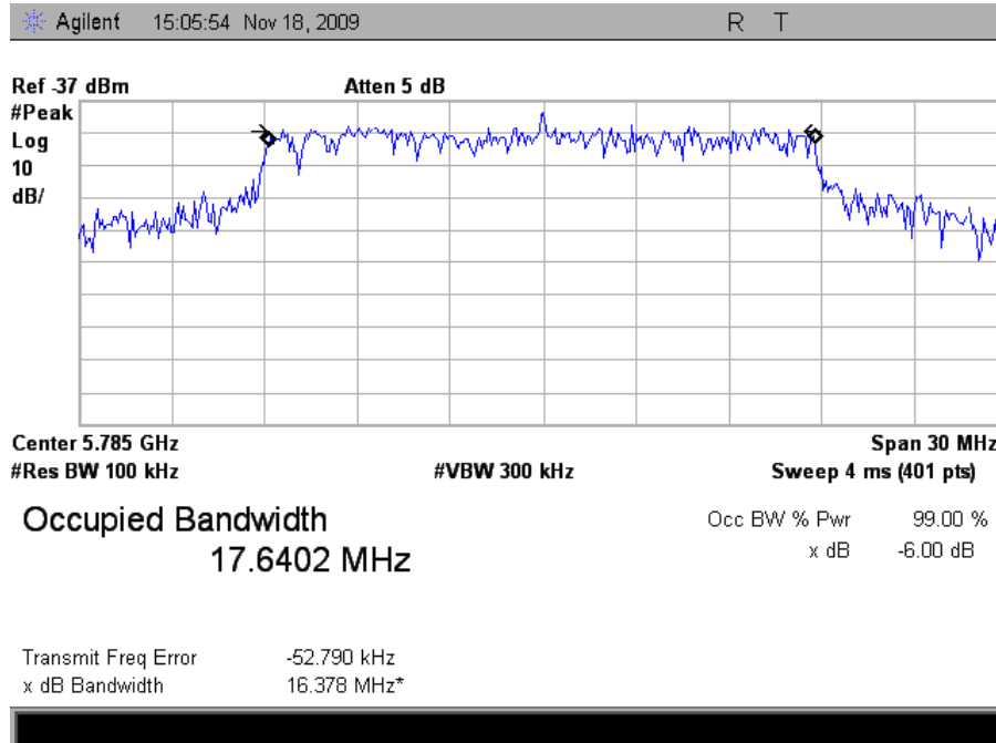
Plot 10. Occupied Band Width, Mid Channel, HT20
