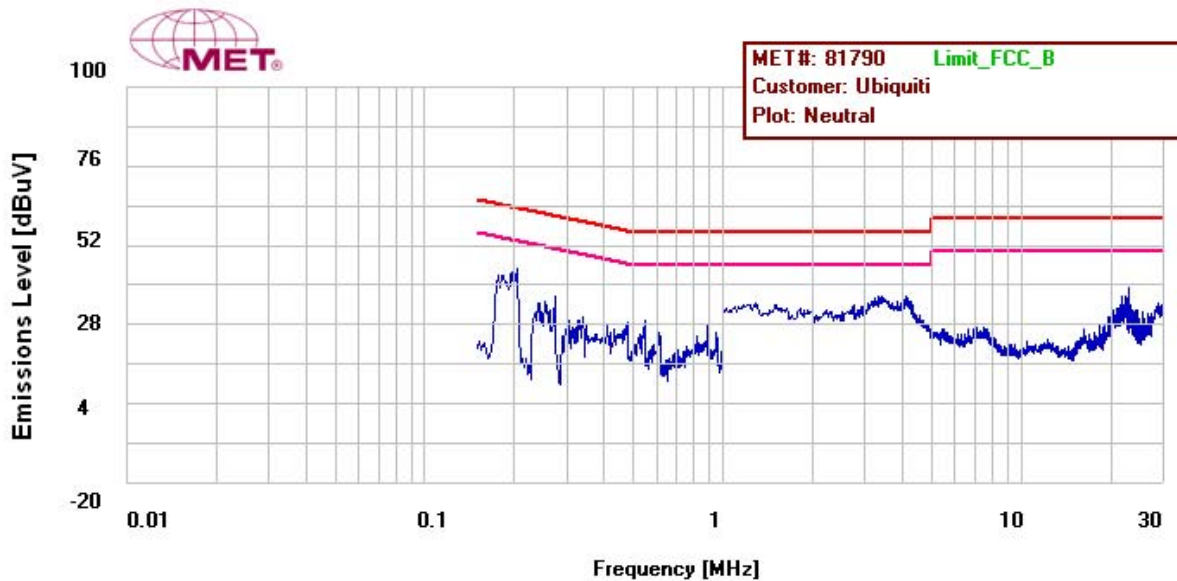
Plot 2. FCC 15B & ICES-003, Conducted Emission Limits, Neutral Line Plot
