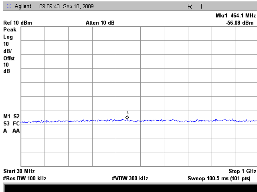
Plot 40. Conducted Emissions, Low Channel, 30 MHz – 1 GHz (HT20)
