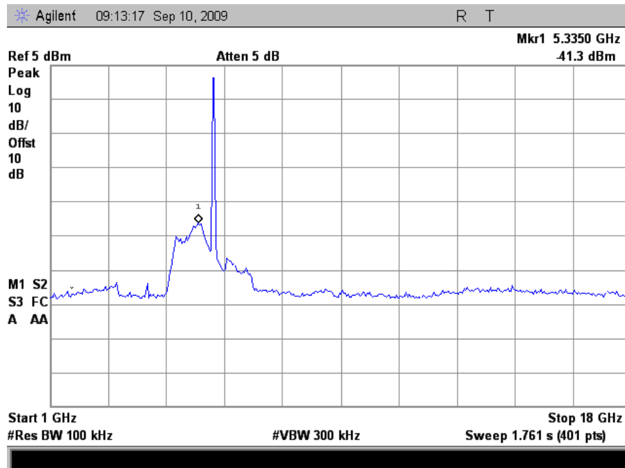
Plot 45. Conducted Emissions, Mid Channel, 1 GHz – 18 GHz (HT20)
