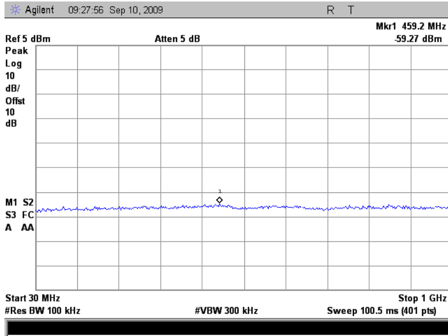
Plot 60. Conducted Emissions, High Channel, 30 MHz – 1 GHz (HT40)
