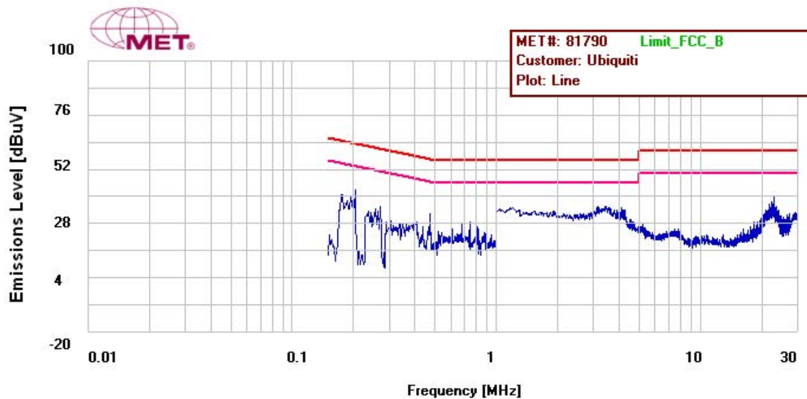
Plot 6. 15.207 Conducted Emission, Phase Line Plot
