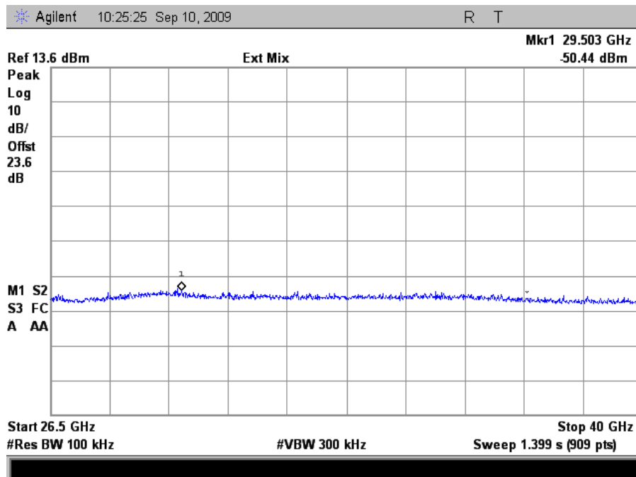
Plot 43. Conducted Emissions, Low Channel, 26.5 GHz – 40GHz (HT20)
