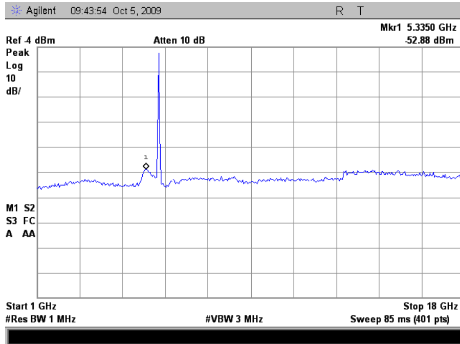
Plot 31. Radiated Spurious Emissions, High Channel, HT20 (Grid Antenna)
