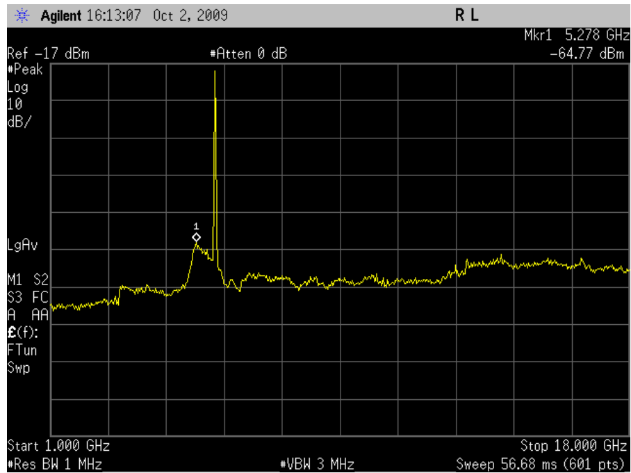
Plot 28. Radiated Spurious Emissions, High Channel, HT20 (Dish Antenna)
