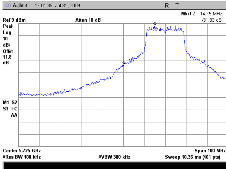
Plot 65. Conducted Band Edge, Low Channel HT20
