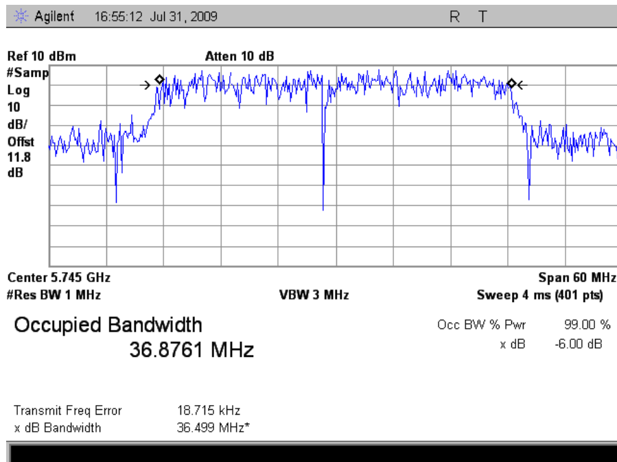
Plot 15. Occupied Band Width, Low Channel, HT40 (99%)
