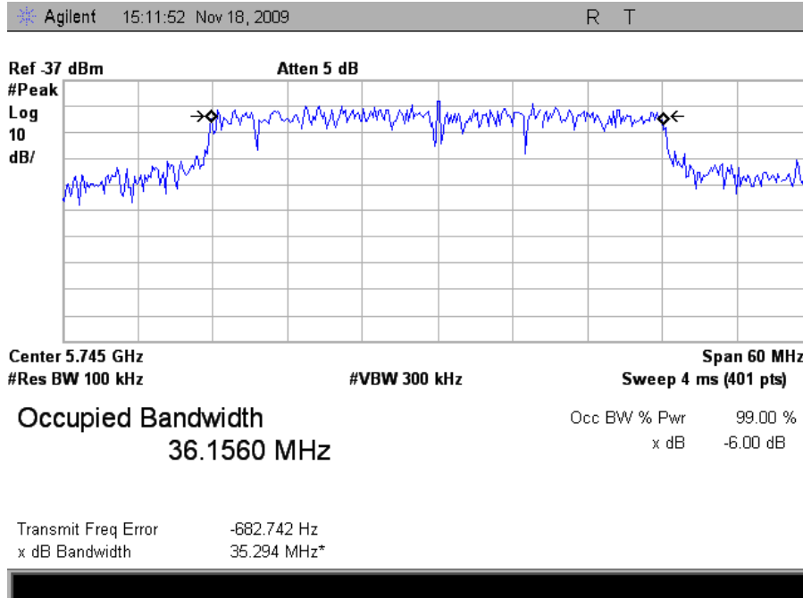
Plot 14. Occupied Band Width, Low Channel, HT40
