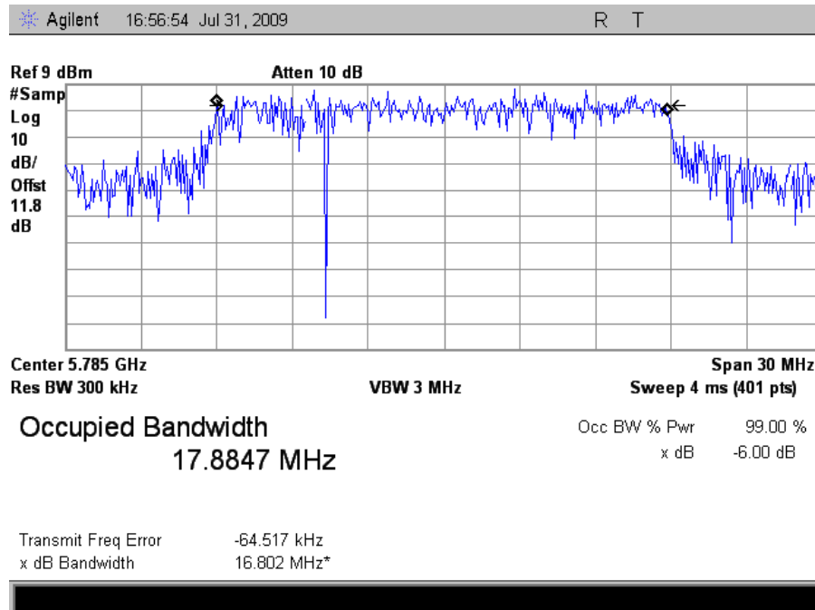
Plot 11. Occupied Band Width, Mid Channel, HT20 (99%)
