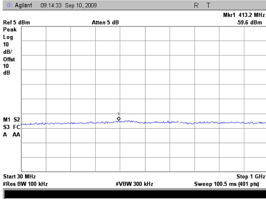
Plot 48. Conducted Emissions, High Channel, 30 MHz – 1 GHz (HT20)
