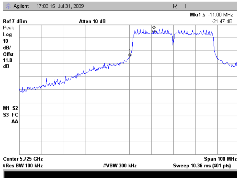
Plot 67. Conducted Band Edge, Low Channel HT40
