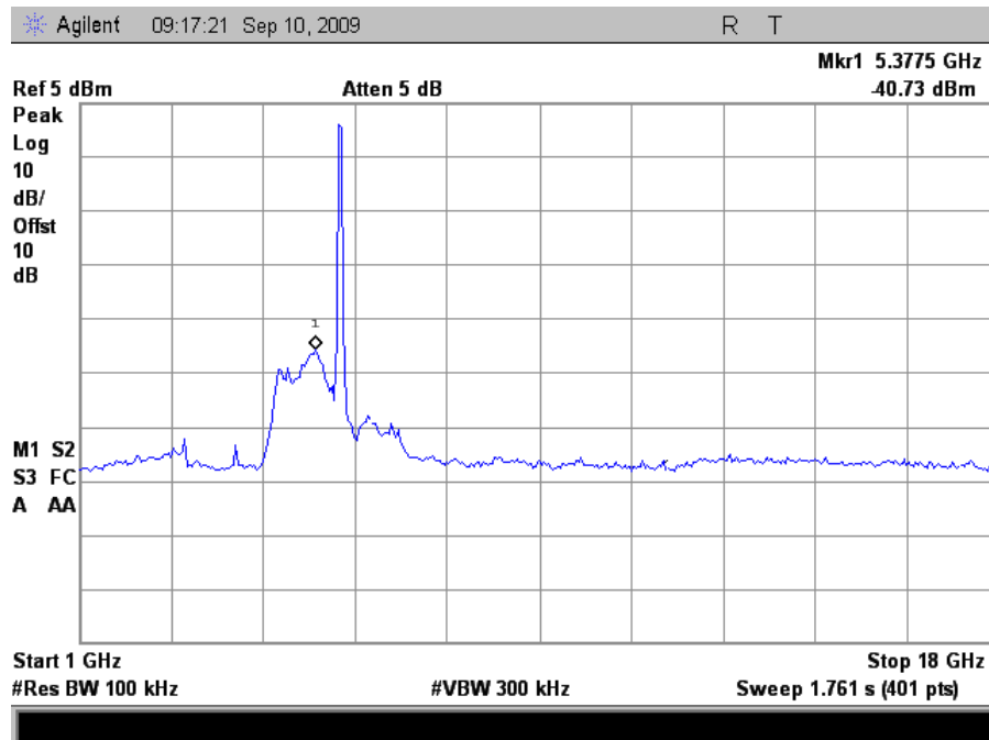
Plot 57. Conducted Emissions, Mid Channel, 1 GHz – 18 GHz (HT40)
