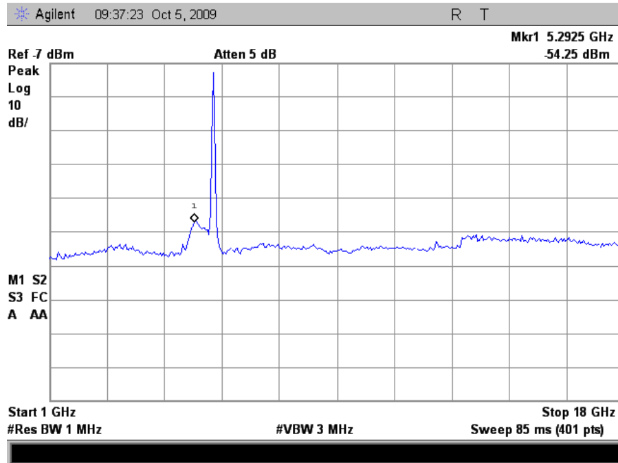
Plot 37. Radiated Spurious Emissions, High Channel, HT40 (Grid Antenna)
