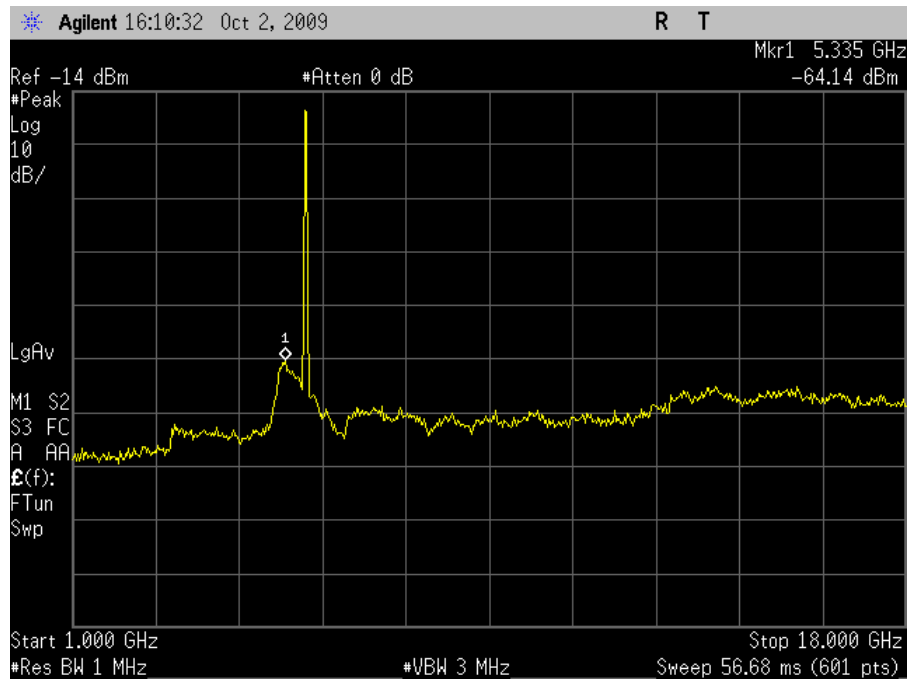
Plot 26. Radiated Spurious Emissions, Low Channel, HT20 (Dish Antenna)
