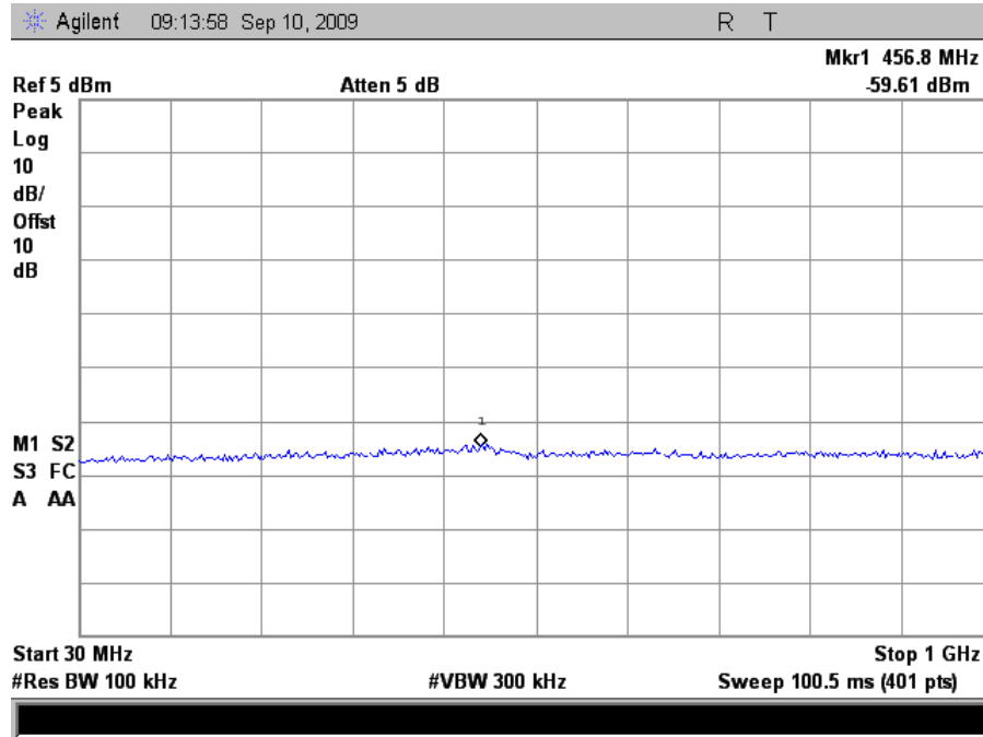
Plot 44. Conducted Emissions, Mid Channel, 30 MHz – 1 GHz (HT20)
