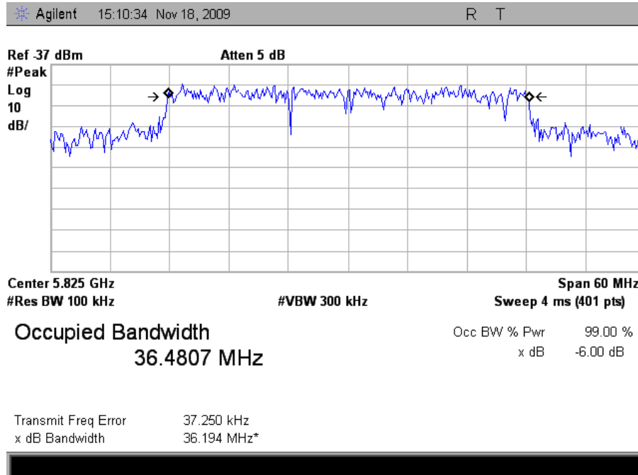
Plot 18. Occupied Band Width, High Channel, HT40
