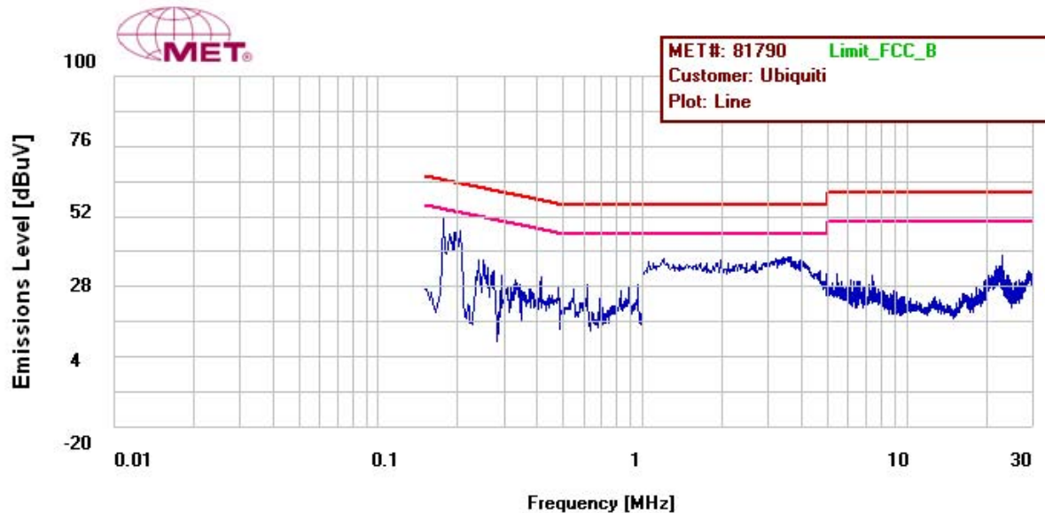
Plot 1. FCC 15B & ICES-003, Conducted Emission Limits, Phase Line Plot
