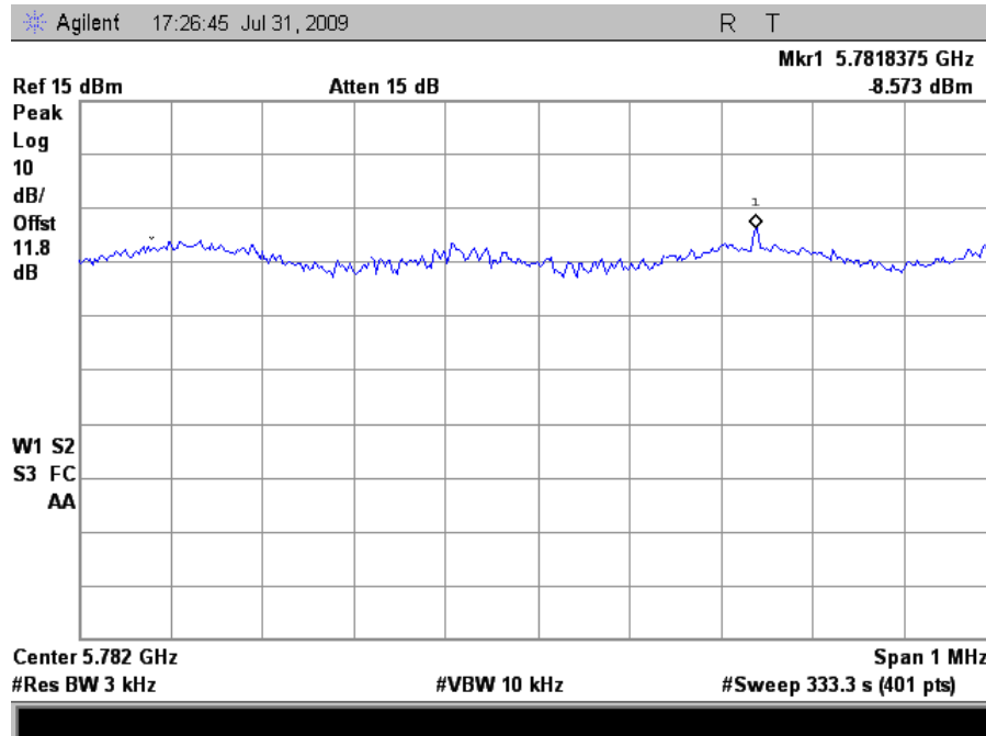
Plot 72. Peak Power Spectral Density, Mid Channel HT40
