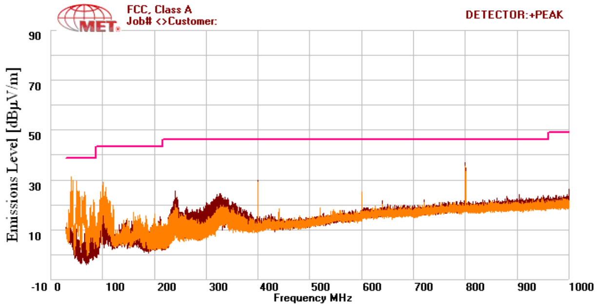
Plot 3. Radiated Emission Limits for FCC Part 15 Subpart B
