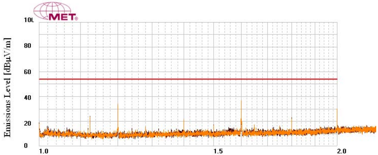
Plot 4. Radiated Emission Limits for FCC Part 15 Subpart B, Above 1GHz
