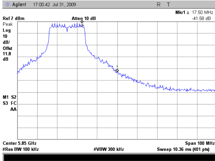
Plot 64. Conducted Band Edge, High Channel HT20
