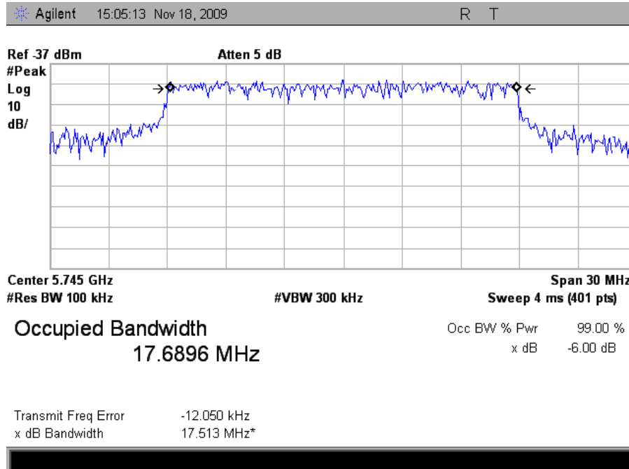
Plot 8. Occupied Band Width, Low Channel, HT20
