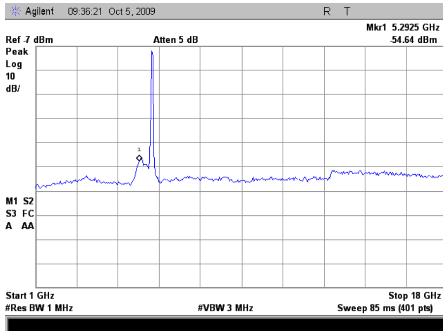
Plot 36. Radiated Spurious Emissions, Mid Channel, HT40 (Grid Antenna)
