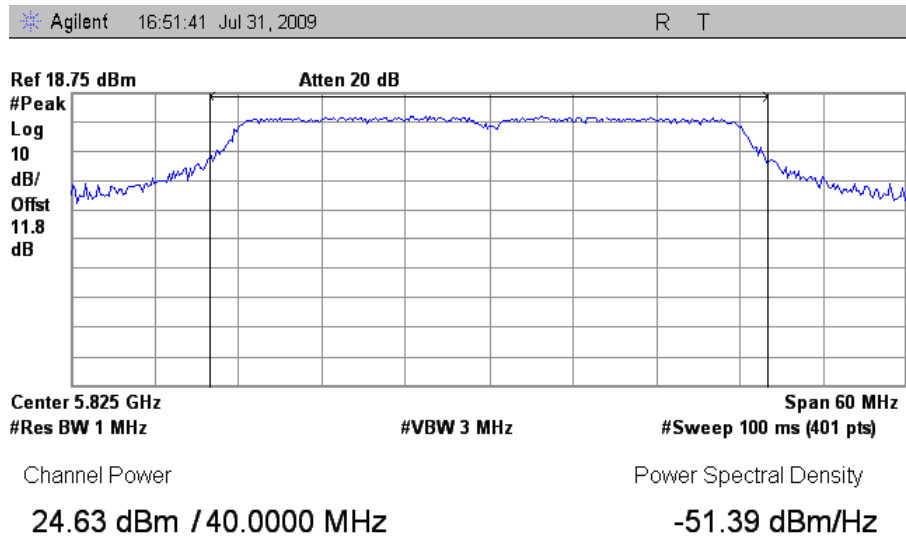
Plot 24. Peak Output Power, Mid Channel – HT40
