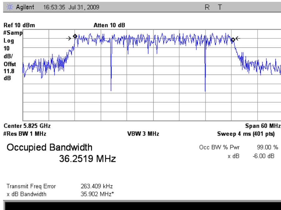
Plot 19. Occupied Band Width, High Channel, HT40 (99%)
