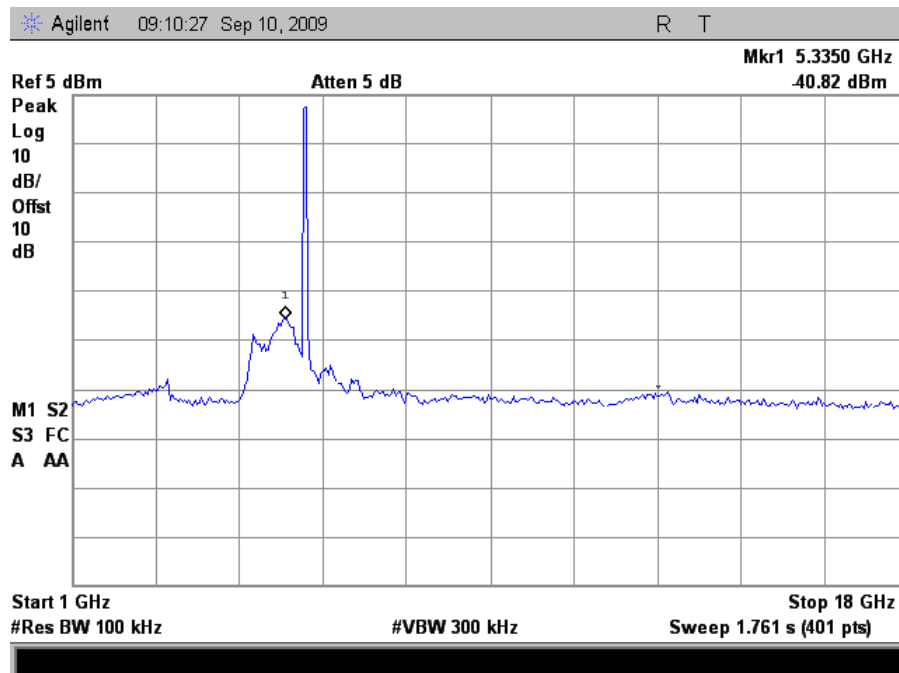
Plot 41. Conducted Emissions, Low Channel, 1 GHz – 18 GHz (HT20)
