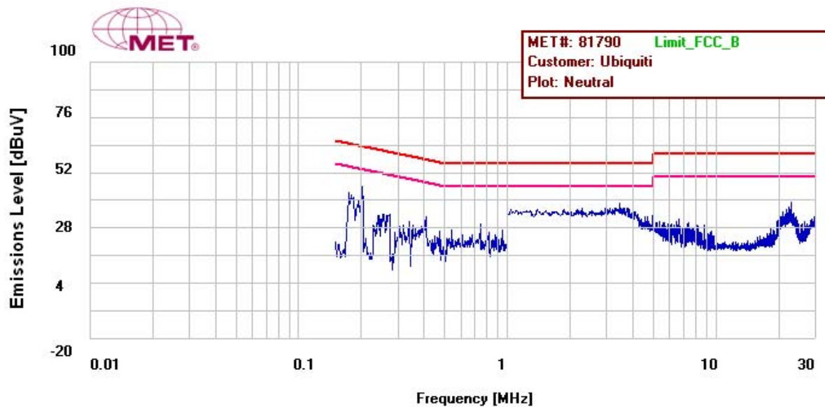
Plot 7. 15.207 Conducted Emission, Neutral Line Plot
