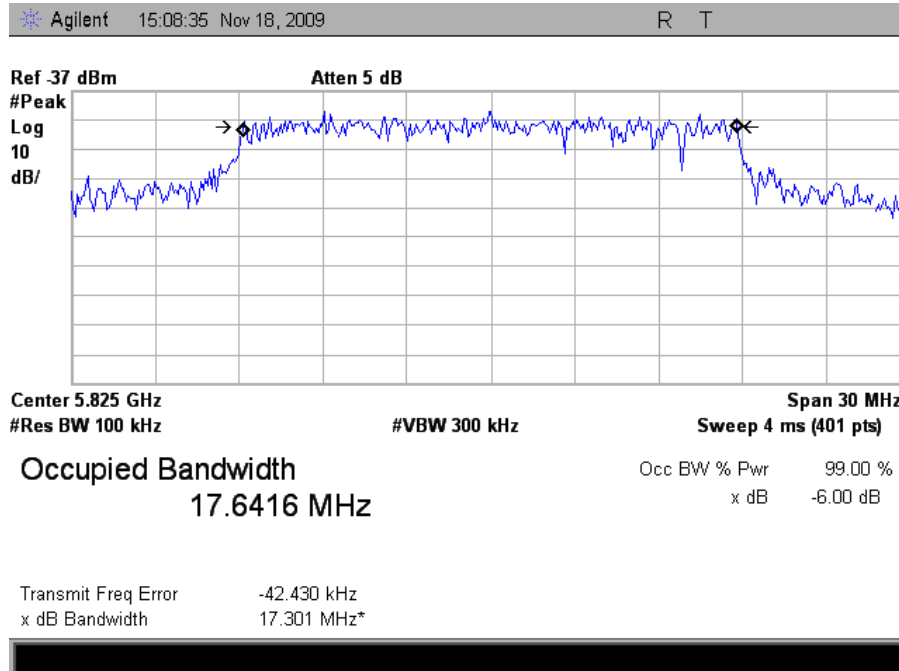
Plot 12. Occupied Band Width, High Channel, HT20
