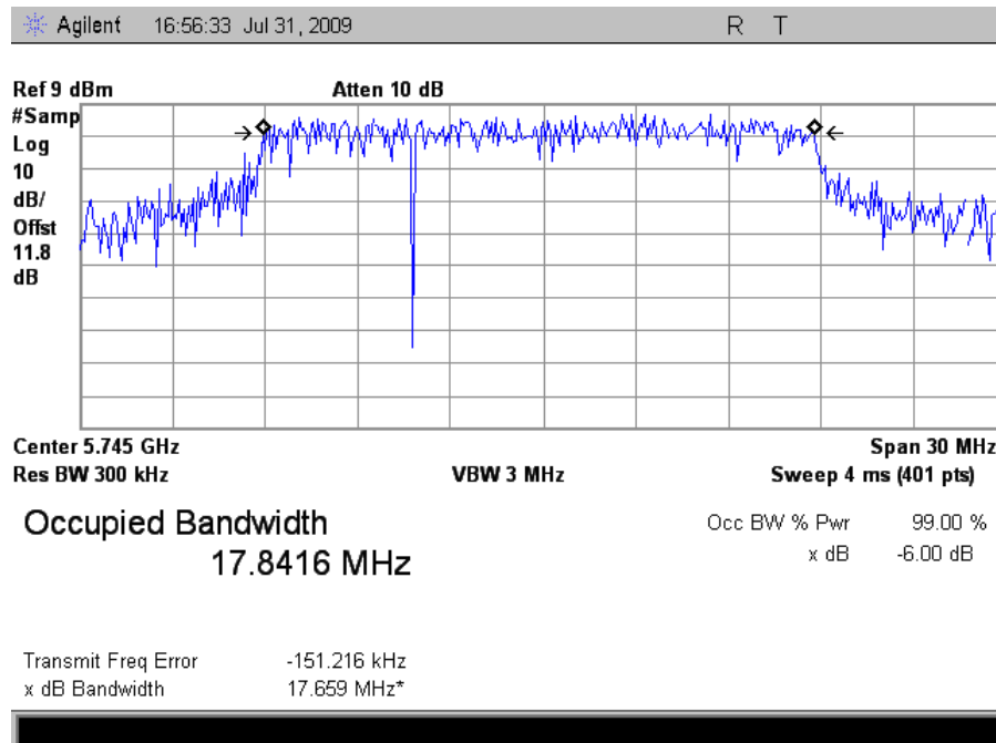
Plot 9. Occupied Band Width, Low Channel, HT20 (99%)
