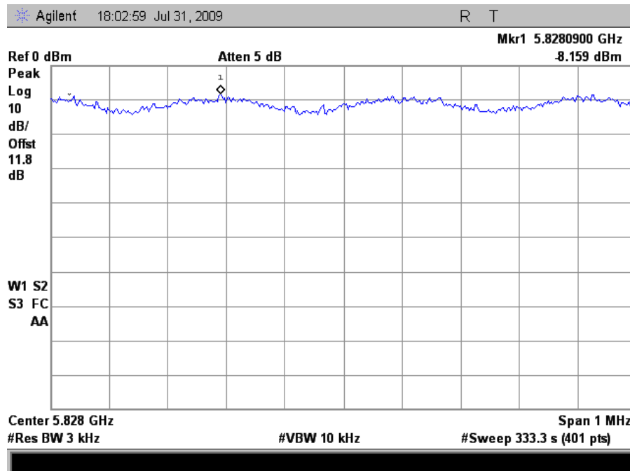
Plot 70. Peak Power Spectral Density, High Channel HT20
