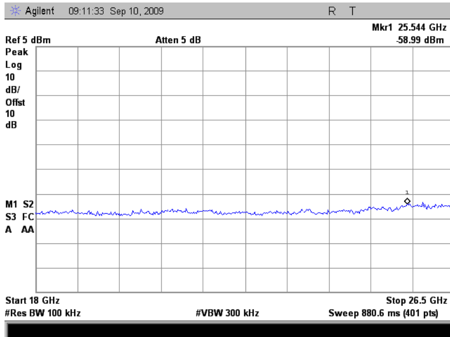
Plot 42. Conducted Emissions, Low Channel, 18 GHz – 26.5 GHz (HT20)
