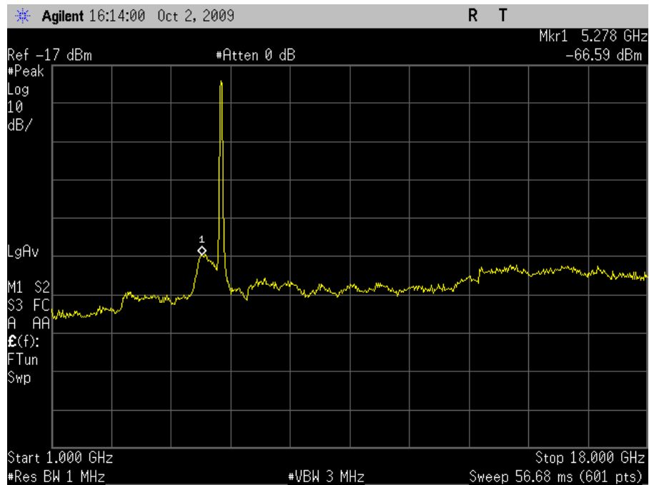
Plot 34. Radiated Spurious Emissions, High Channel, HT40 (Dish Antenna)
