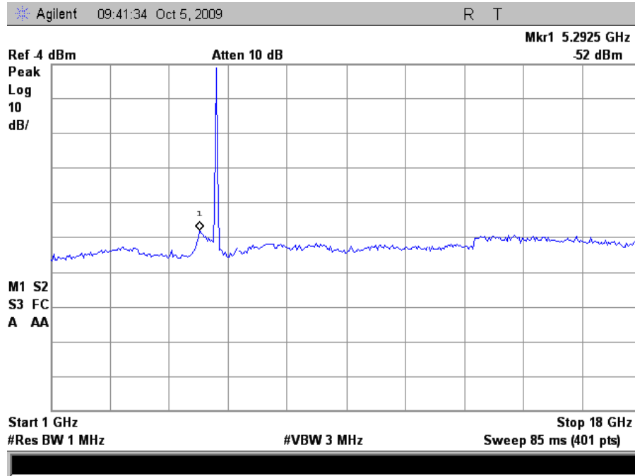
Plot 29. Radiated Spurious Emissions, Low Channel, HT20 (Grid Antenna)
