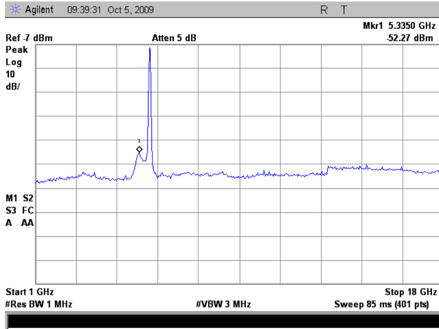
Plot 35. Radiated Spurious Emissions, Low Channel, HT40 (Grid Antenna)
