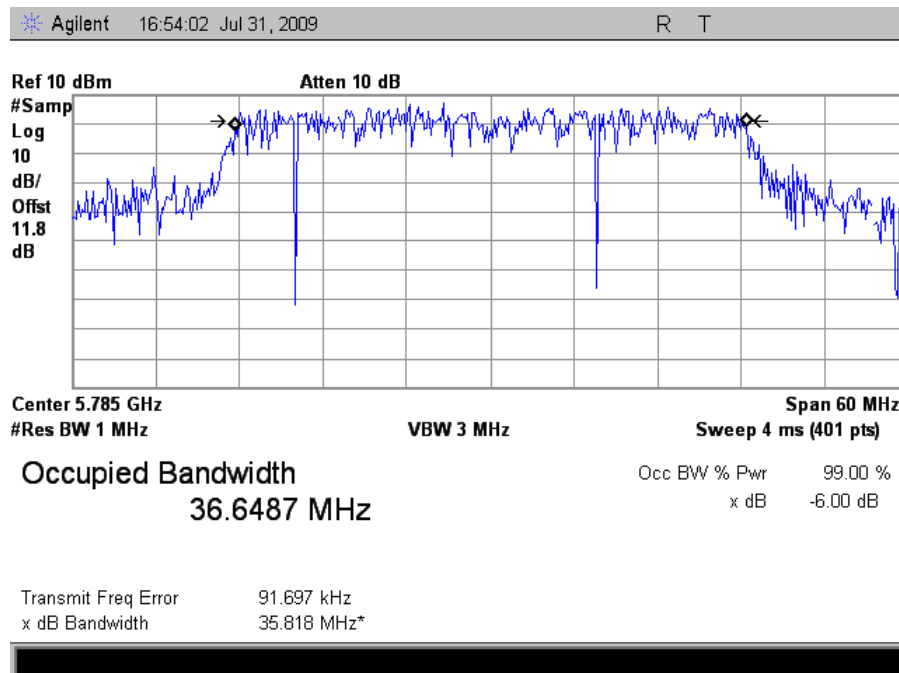
Plot 17. Occupied Band Width, Mid Channel, HT40 (99%)
