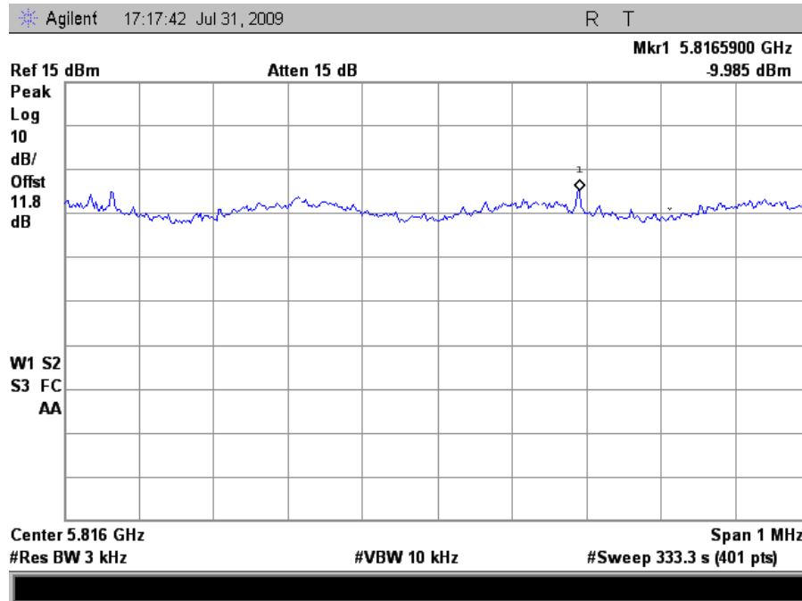
Plot 73. Peak Power Spectral Density, High Channel HT40
