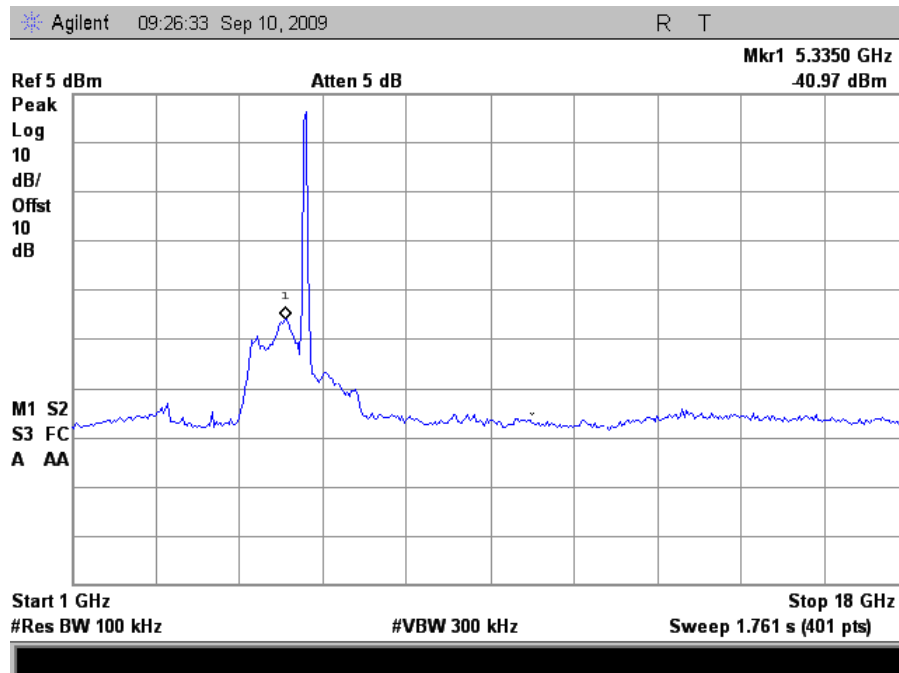
Plot 53. Conducted Emissions, Low Channel, 1 GHz – 18 GHz (HT40)
