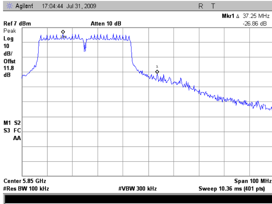
Plot 66. Conducted Band Edge, High Channel HT40
