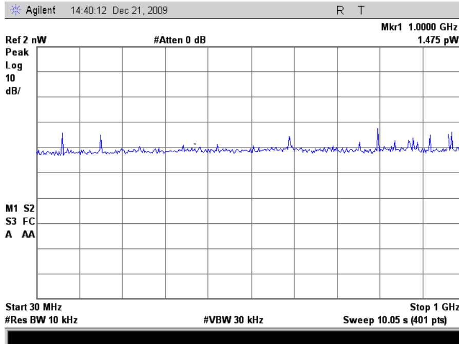
Plot 38. Receiver Spurious Emissions, 30MHz – 1GHz
