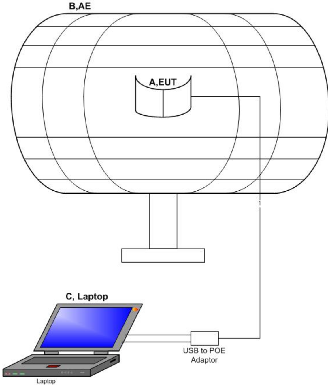
Figure 1. Block Diagram of Test Configuration 1
