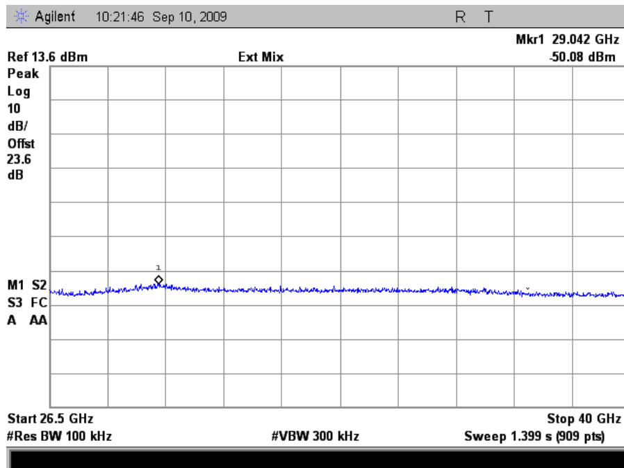
Plot 63. Conducted Emissions, High Channel, 26.5 GHz – 40GHz (HT40)
