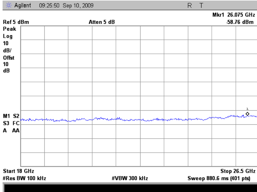
Plot 54. Conducted Emissions, Low Channel, 18 GHz – 26.5 GHz (HT40)
