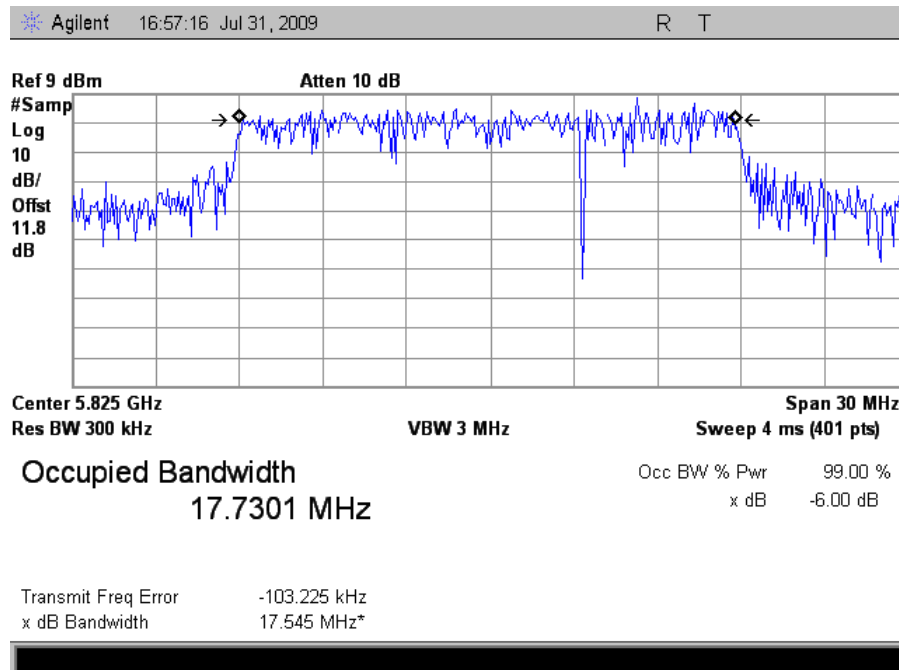
Plot 13. Occupied Band Width, High Channel, HT20 (99%)
