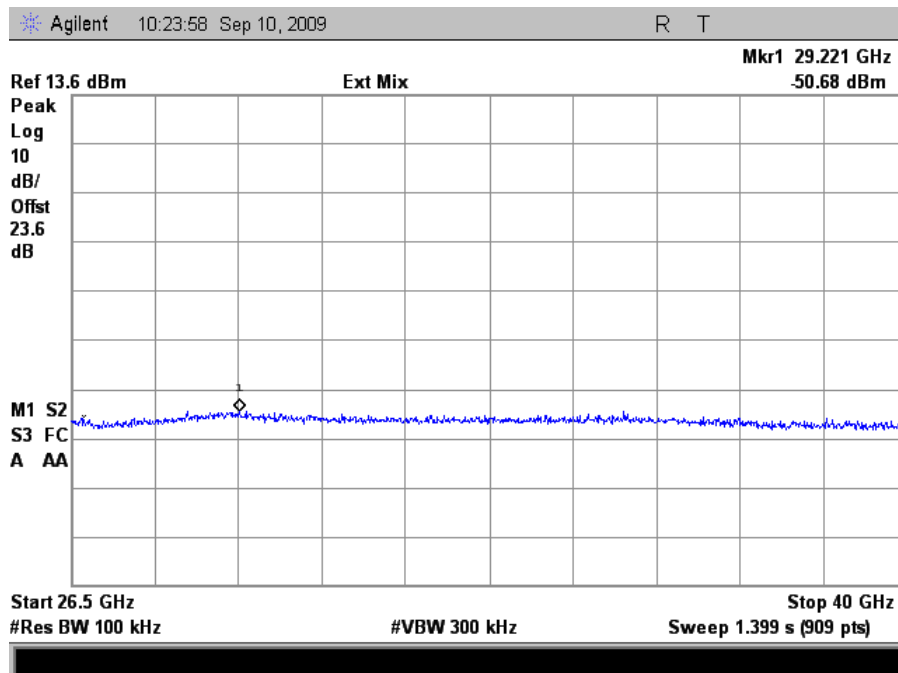
Plot 55. Conducted Emissions, Low Channel, 26.5 GHz – 40GHz (HT40)
