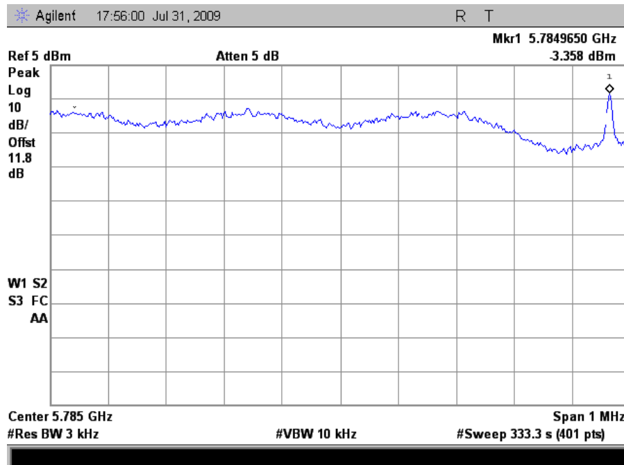
Plot 69. Peak Power Spectral Density, Mid Channel HT20
