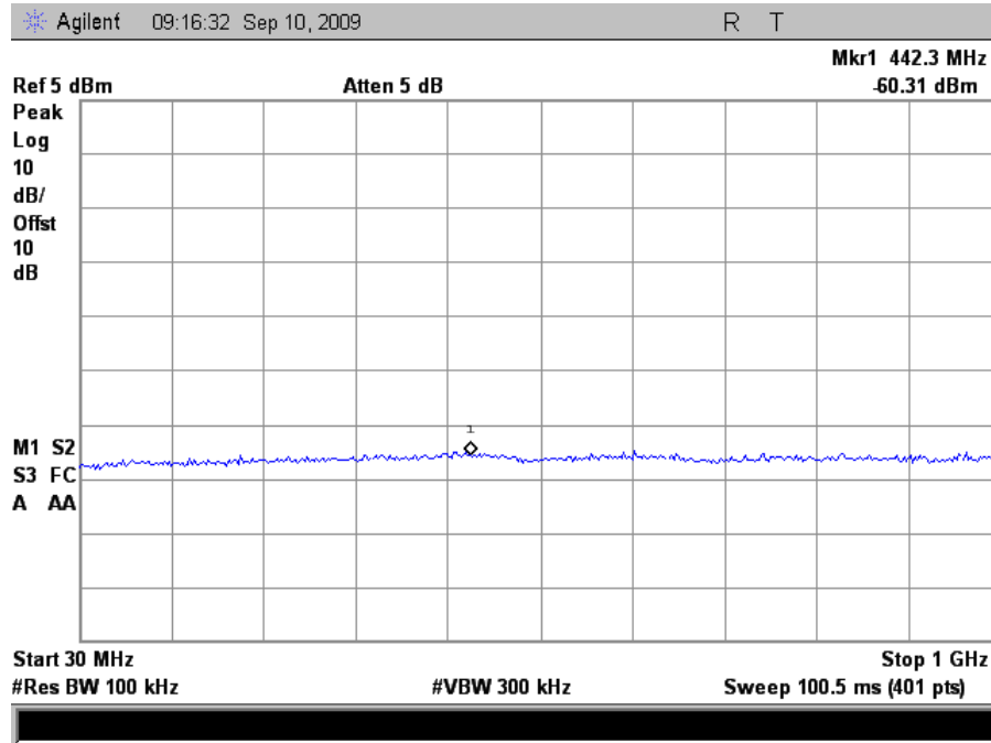
Plot 56. Conducted Emissions, Mid Channel, 30 MHz – 1 GHz (HT40)
