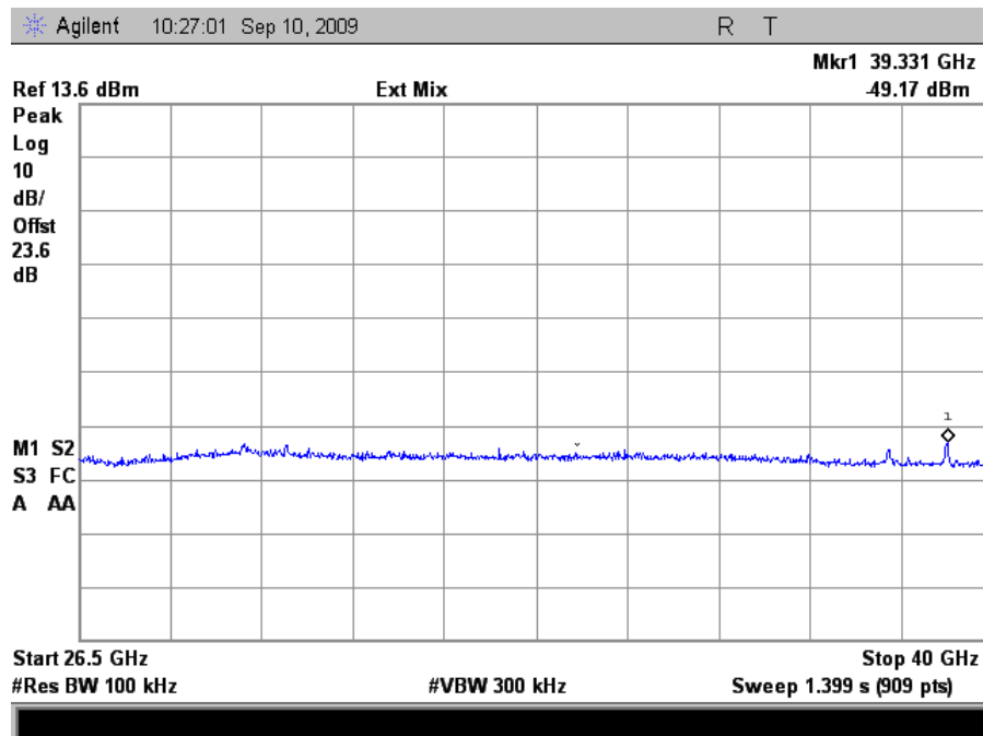
Plot 47. Conducted Emissions, Mid Channel, 26.5 GHz – 40GHz (HT20)
