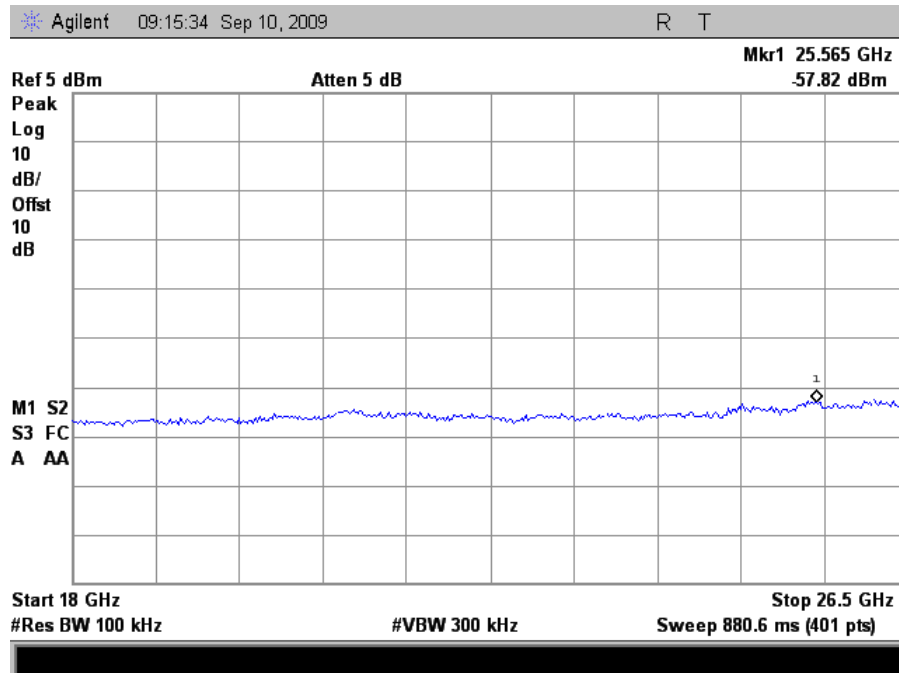
Plot 50. Conducted Emissions, High Channel, 18 GHz – 26.5 GHz (HT20)
