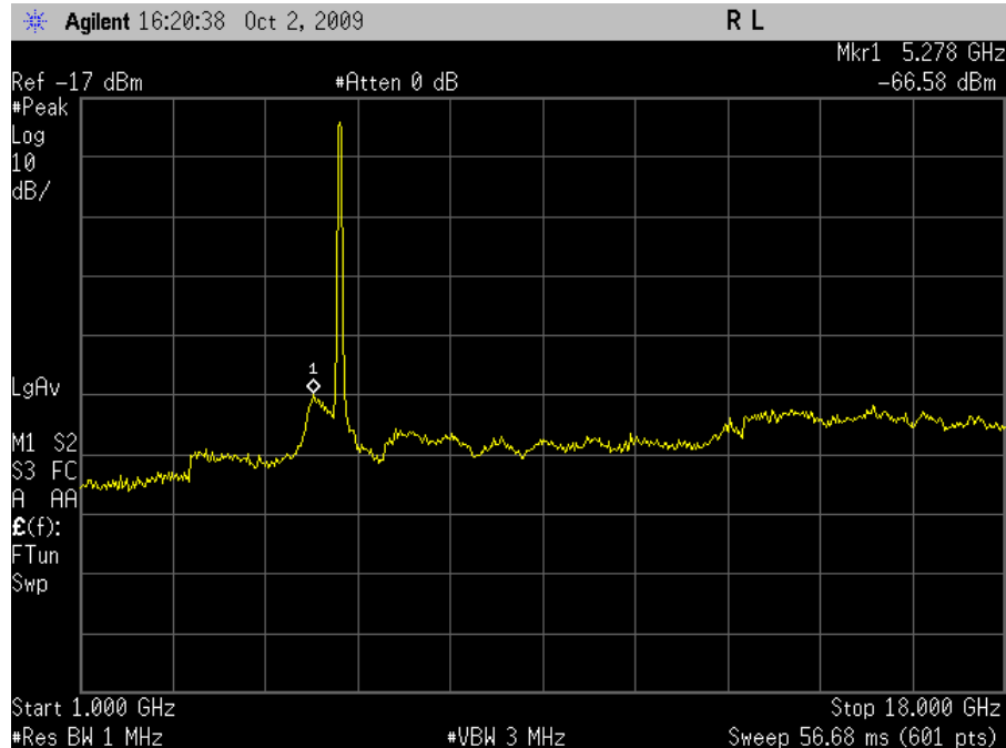
Plot 32. Radiated Spurious Emissions, Low Channel, HT40 (Dish Antenna)
