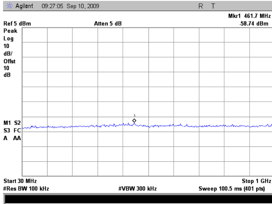
Plot 52. Conducted Emissions, Low Channel, 30 MHz – 1 GHz (HT40)
