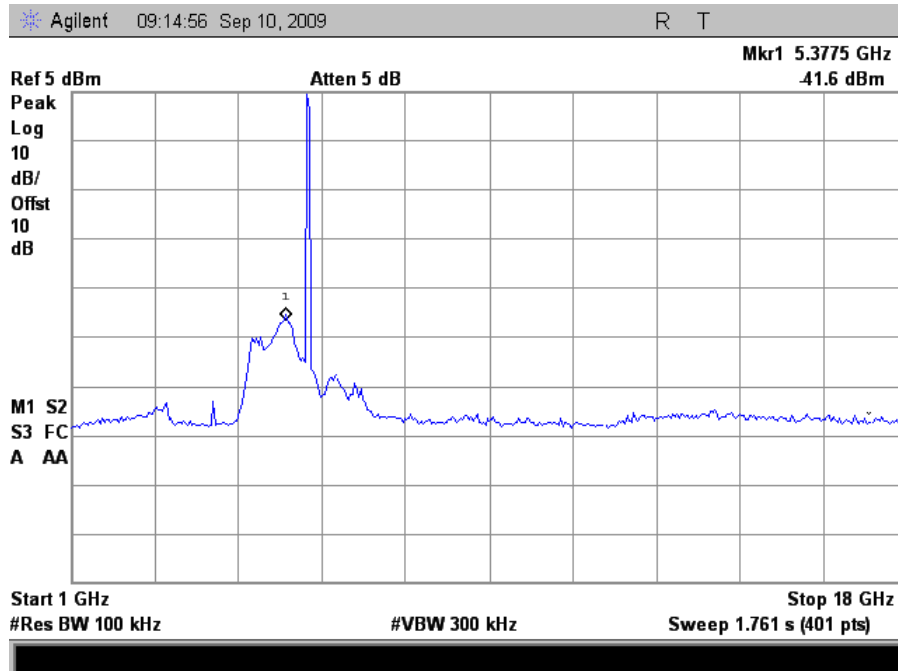
Plot 49. Conducted Emissions, High Channel, 1 GHz – 18 GHz (HT20)
