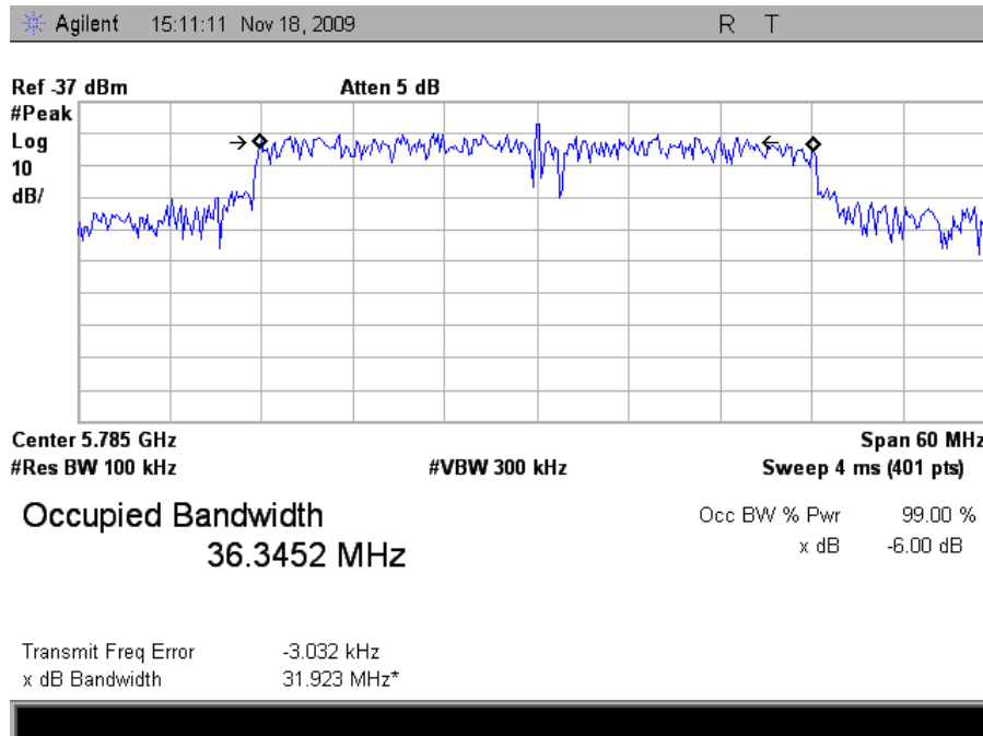
Plot 16. Occupied Band Width, Mid Channel, HT40
