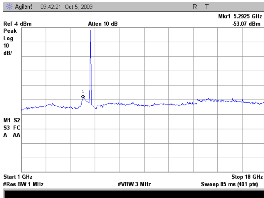
Plot 30. Radiated Spurious Emissions, Mid Channel, HT20 (Grid Antenna)
