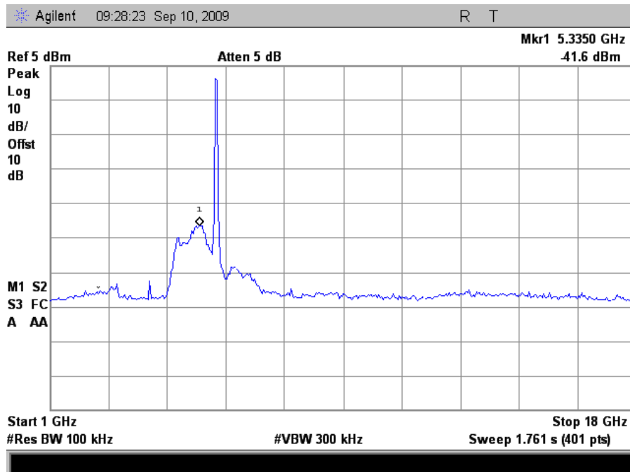
Plot 61. Conducted Emissions, High Channel, 1 GHz – 18 GHz (HT40)
