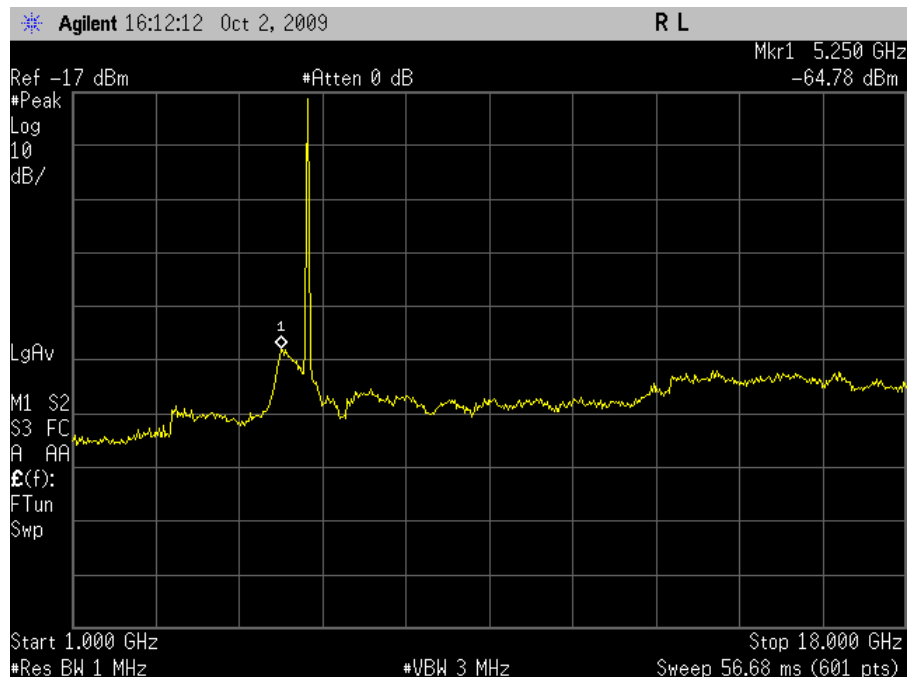
Plot 27. Radiated Spurious Emissions, Mid Channel, HT20 (Dish Antenna)
