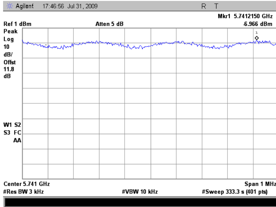
Plot 68. Peak Power Spectral Density, Low Channel HT20
