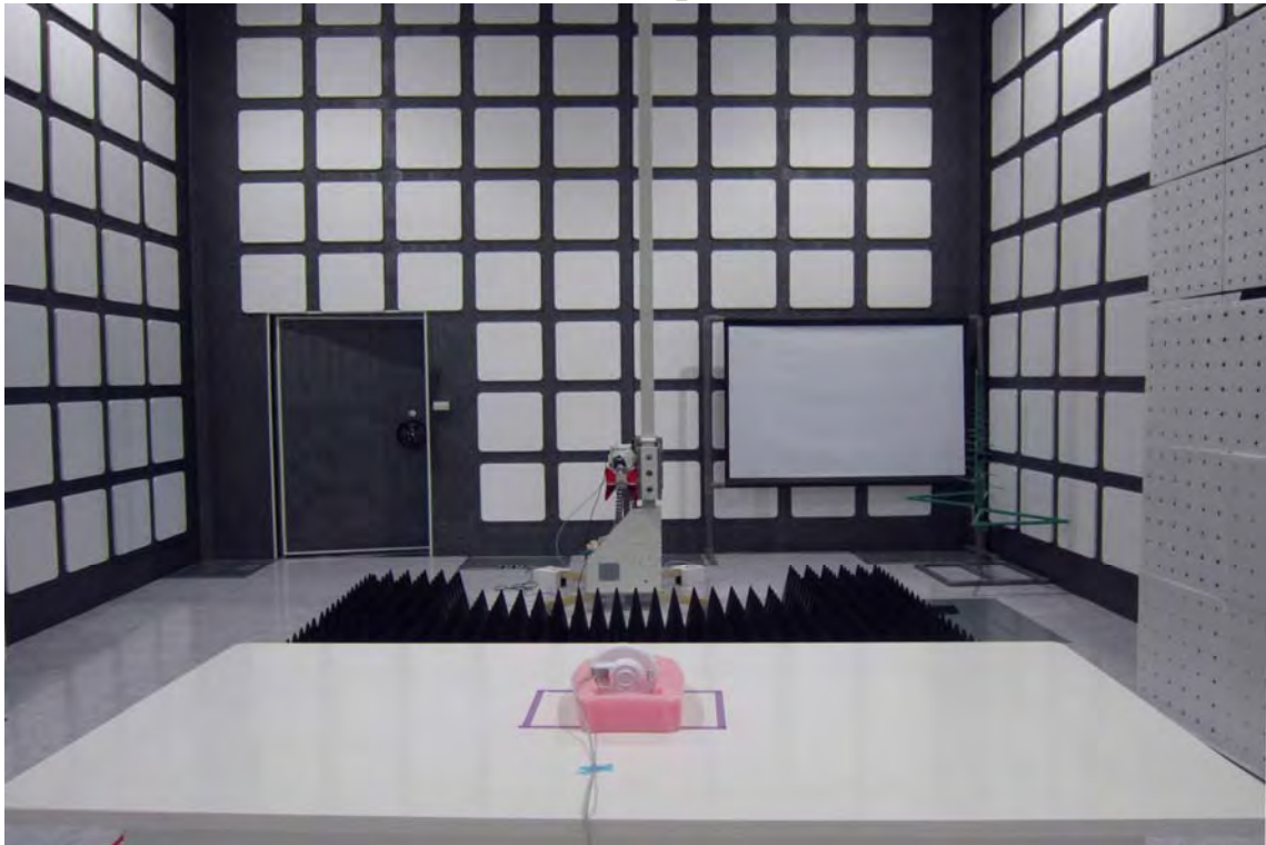
Radiated Emission Set up Photos (E1 Plane)
