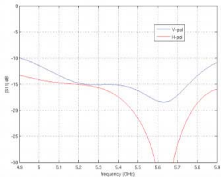
Return Loss
