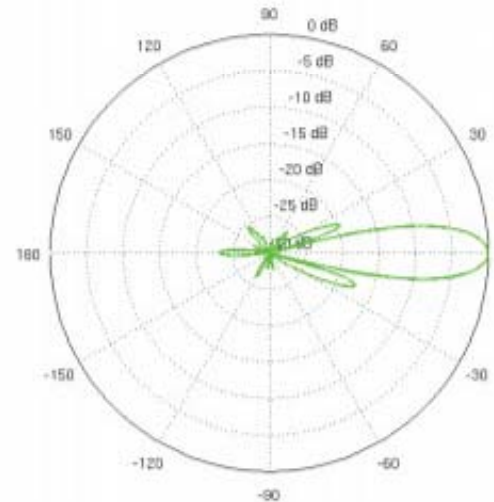
Horizontal Azimuth
