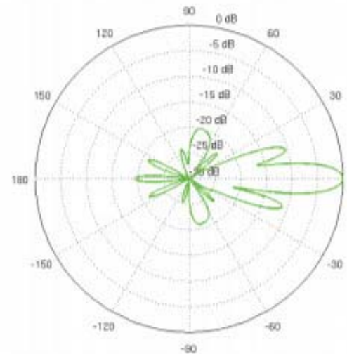
Vertical Azimuth
