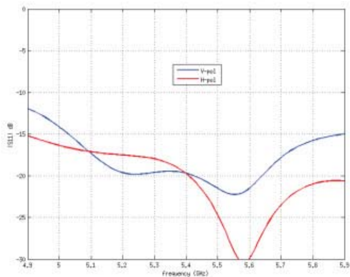
Return Loss
