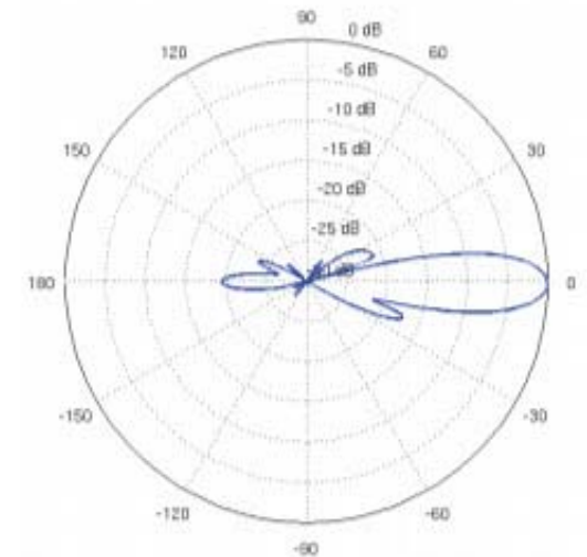
Vertical Elevation
