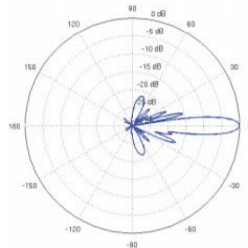
Horizontal Elevation
