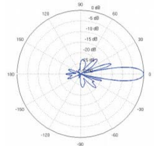
Horizontal Elevation
