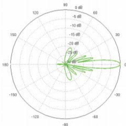
Vertical Azimuth
