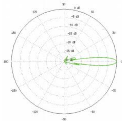
Horizontal Azimuth
