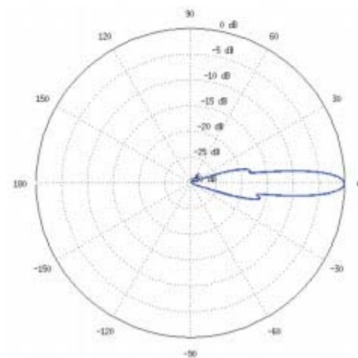
Vertical Elevation
