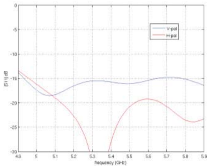
Return Loss
