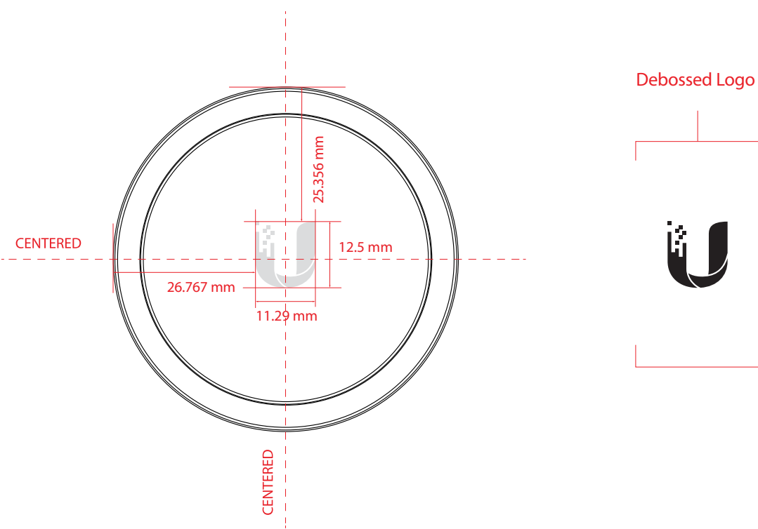
Front Cap 1, Debossed Logo
