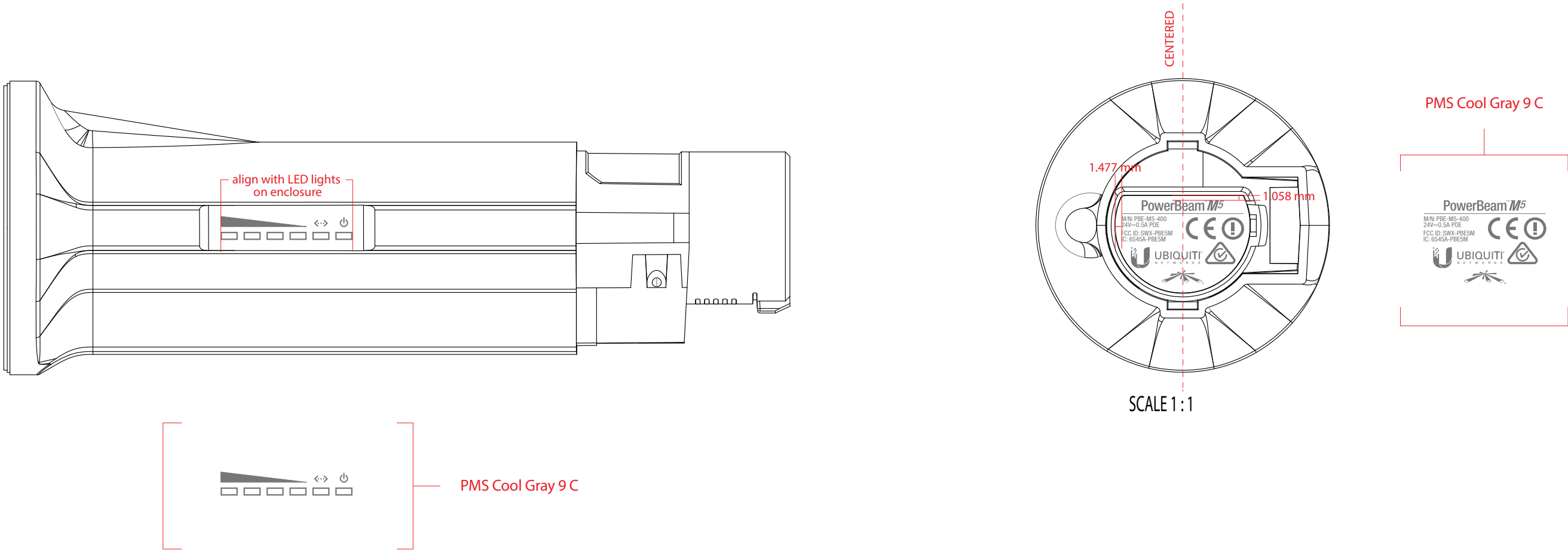
Feed Housing 1, Led pattern 2, Product label
