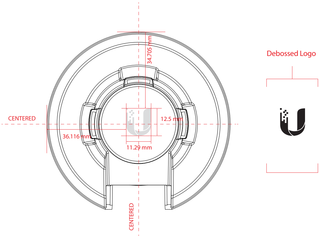
Rear Housing 1, Debossed Logo
