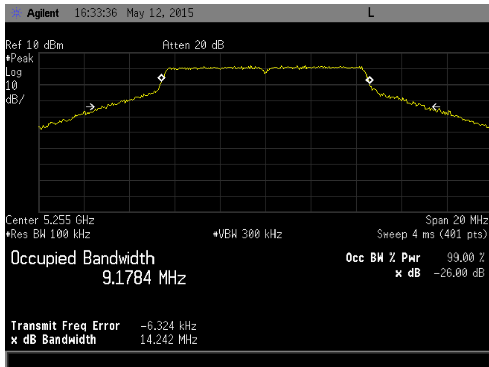
UNII-2A_J8_10 MHz BW_low
