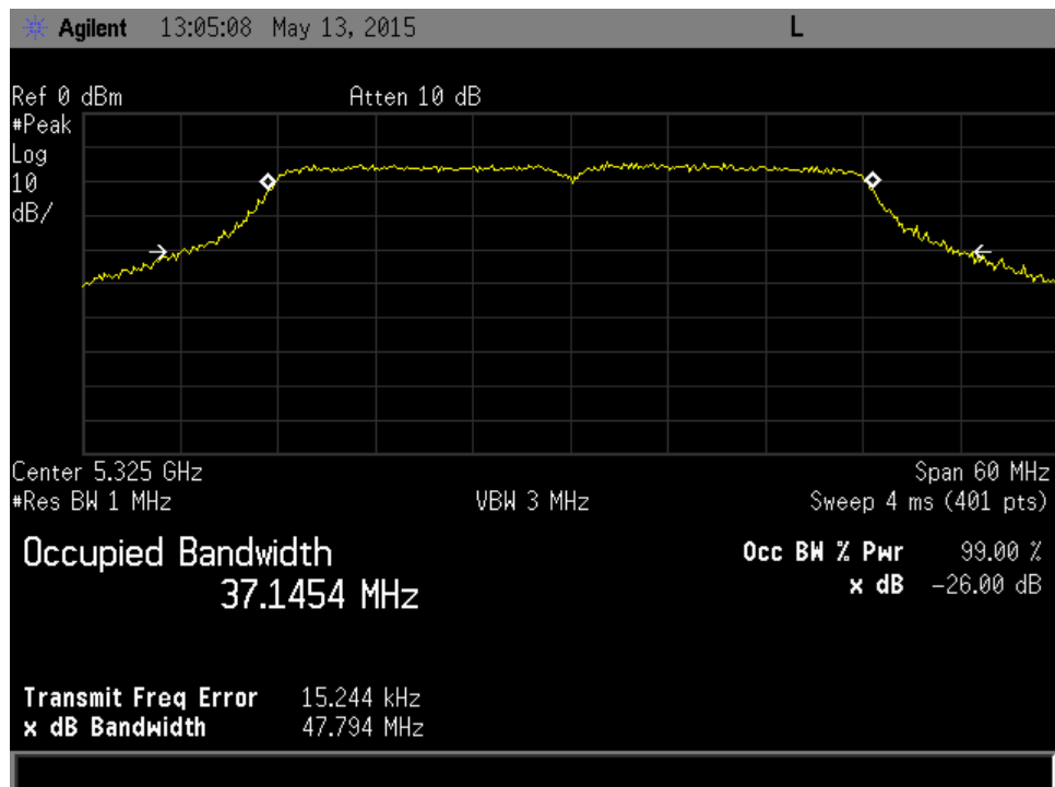
UNII-2A_J8_40 MHz BW_hi
