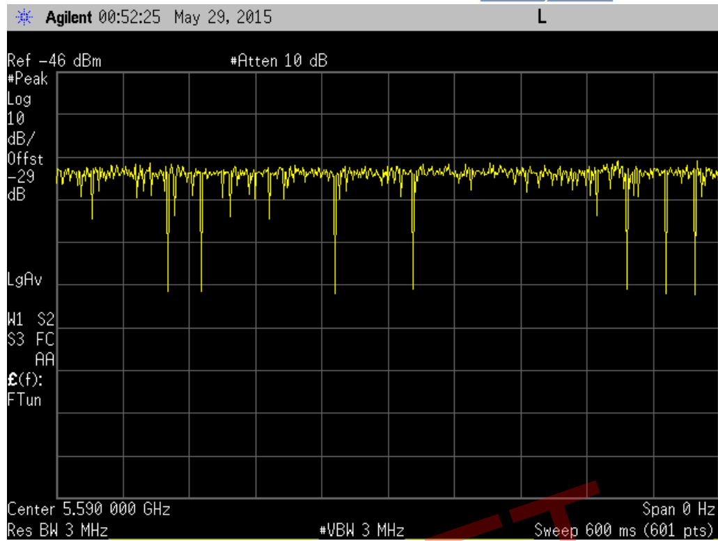
20MHz Traffic
