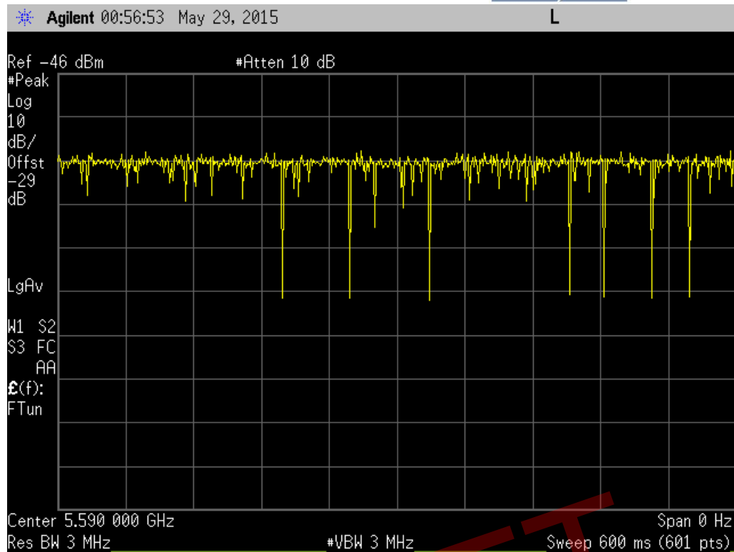
40MHz Traffic
