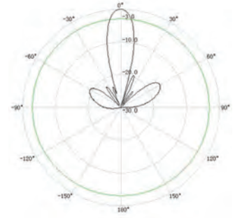
Vertical Elevation
