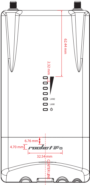
TOP VIEW
