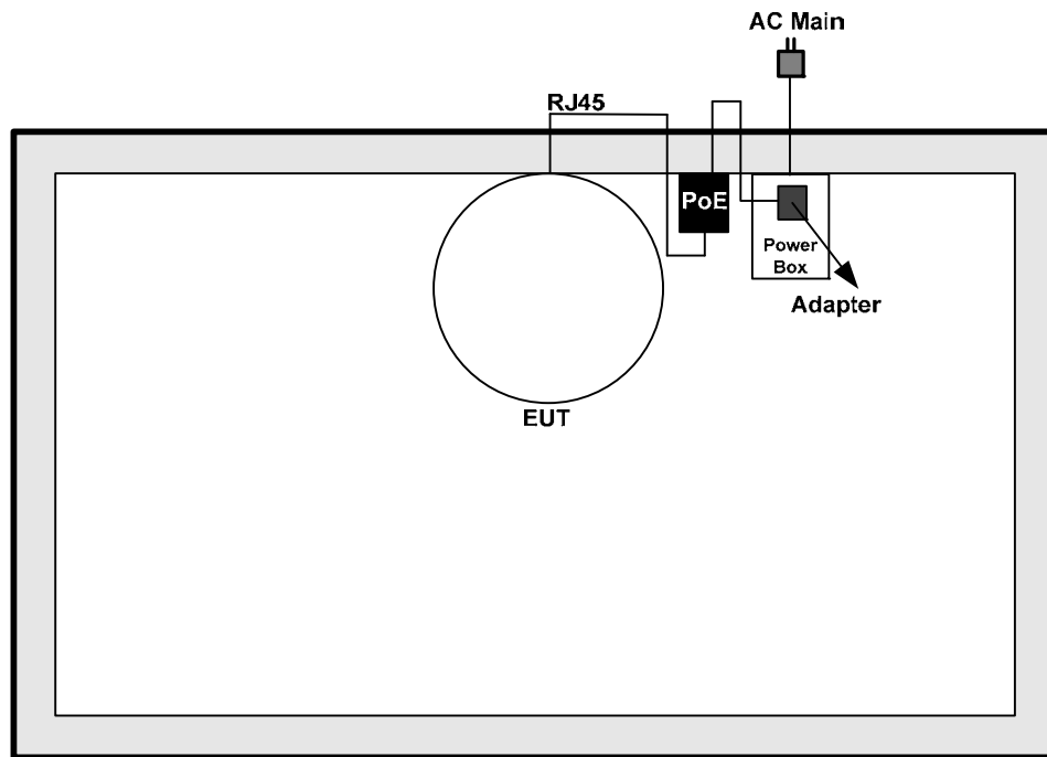
Test Setup Diagram - Radiated Emission Below 1GHz Test (Mode 3)
