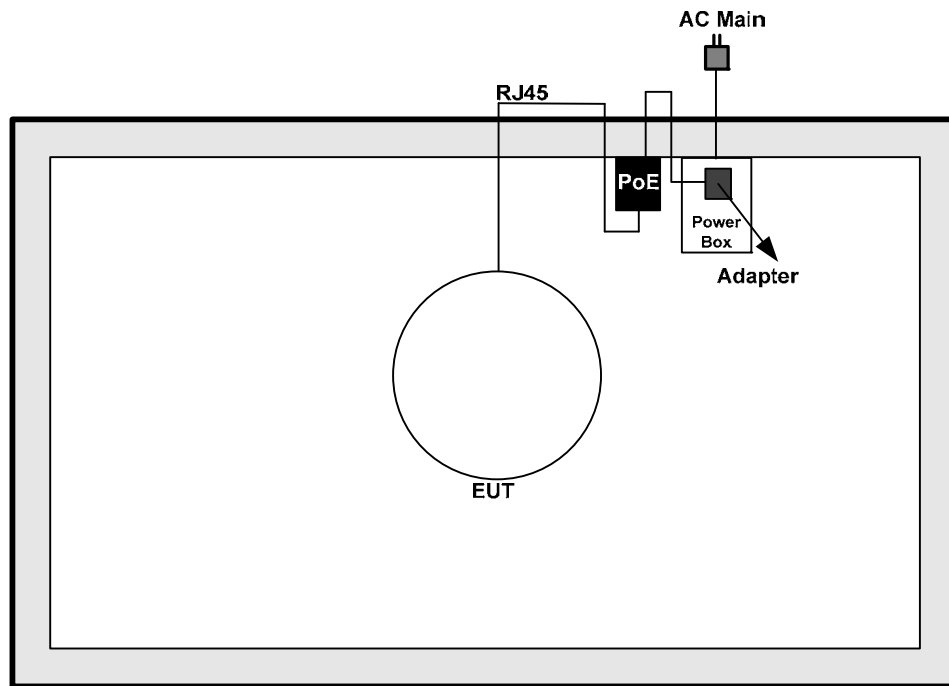
Test Setup Diagram - Radiated Emission Above 1GHz Test (Mode 3)
