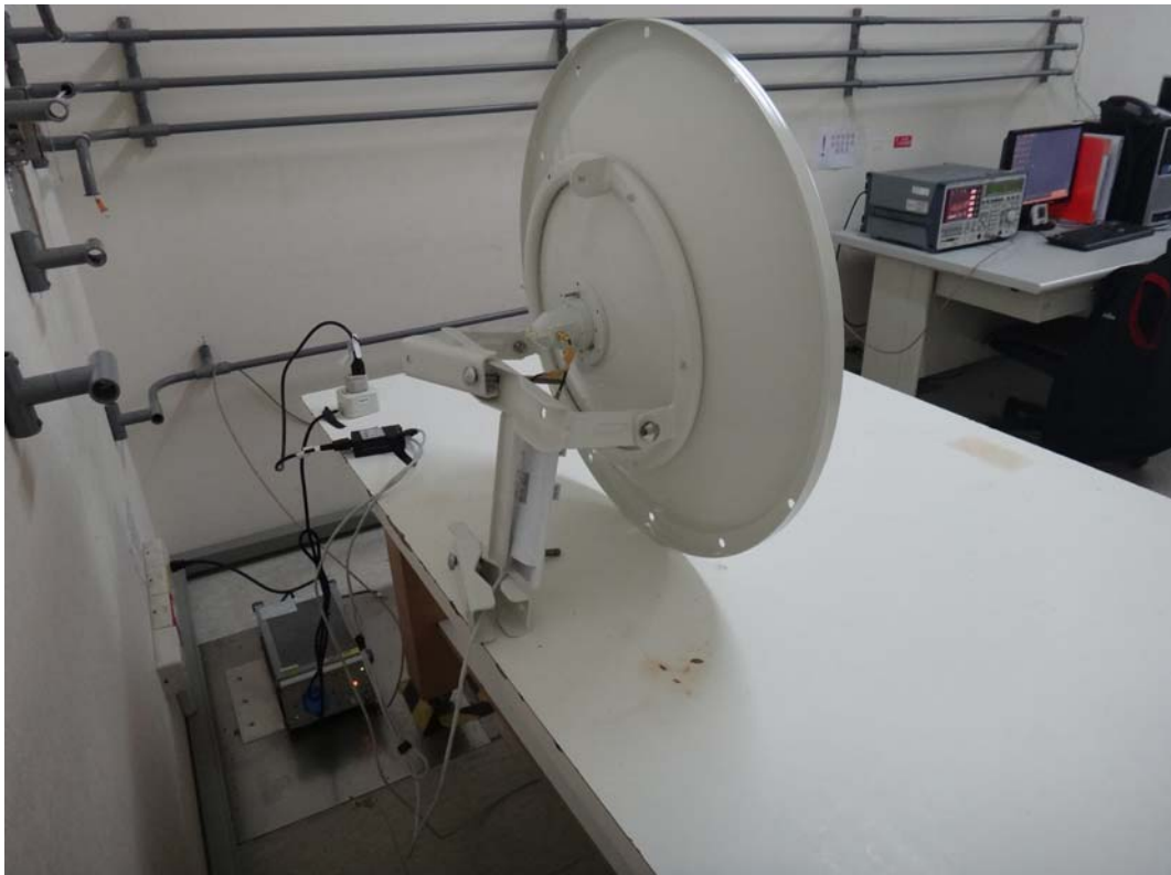
Back View of Conducted Test – Dish Antenna
