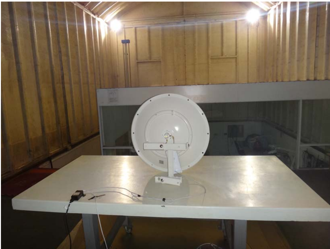
Back View of Radiated Test – Dish Antenna
