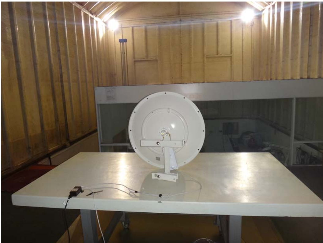
Back View of Radiated Test (Horn) - Dish Antenna
