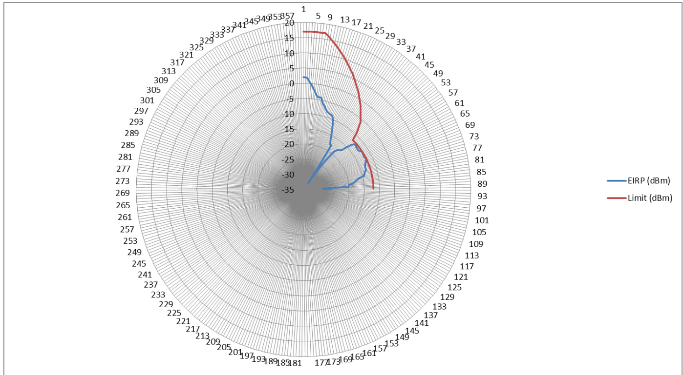
AMO-5G13 - Horizontal
