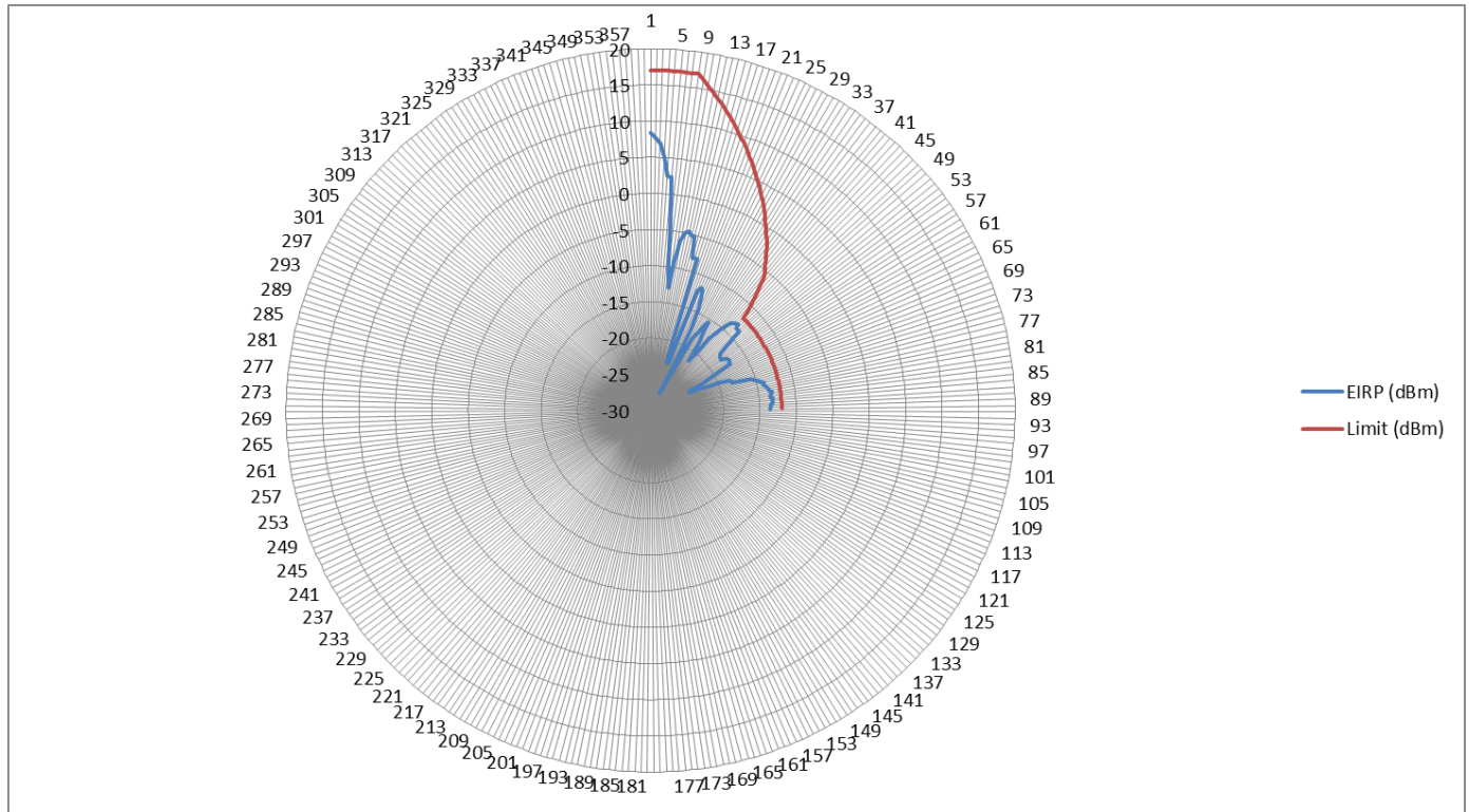
AM-5G16-Horizontal
