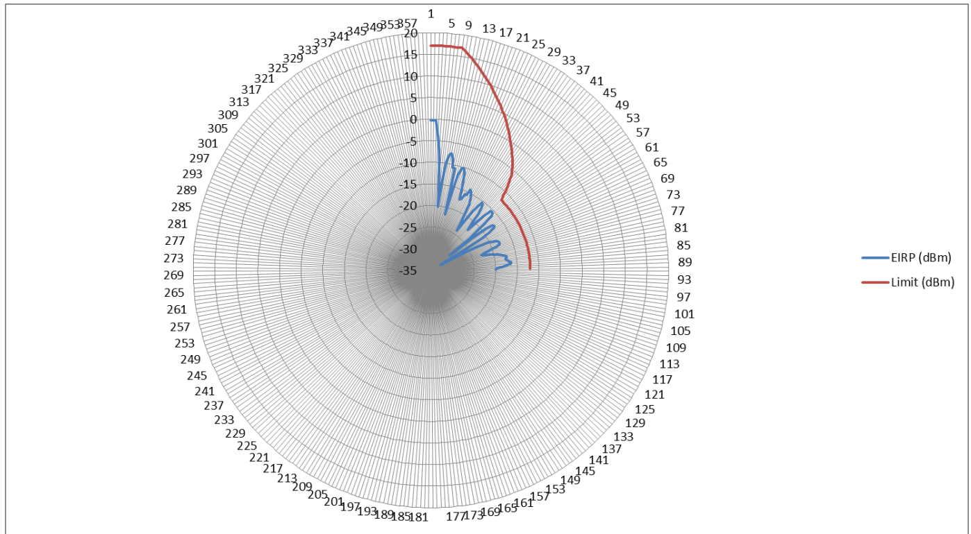
AMO-5G13 - Horizontal
