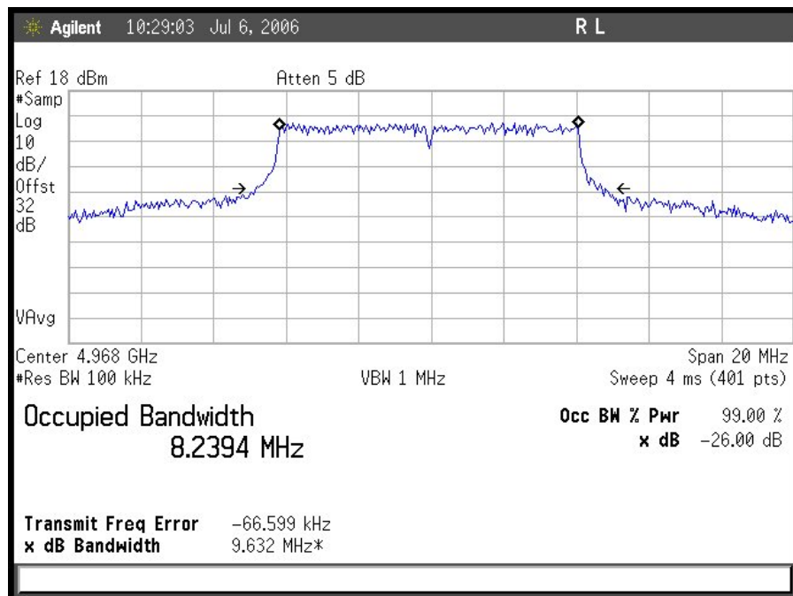
Plot 2. Occupied Bandwidth 10 MHz
