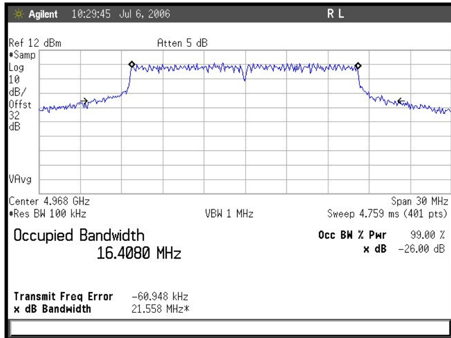
Plot 3. Occupied Bandwidth 20 MHz
