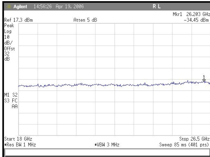
Plot 25. Conducted Spurious Emissions 20 MHz Low Ch (18 GHz – 26 GHz)
