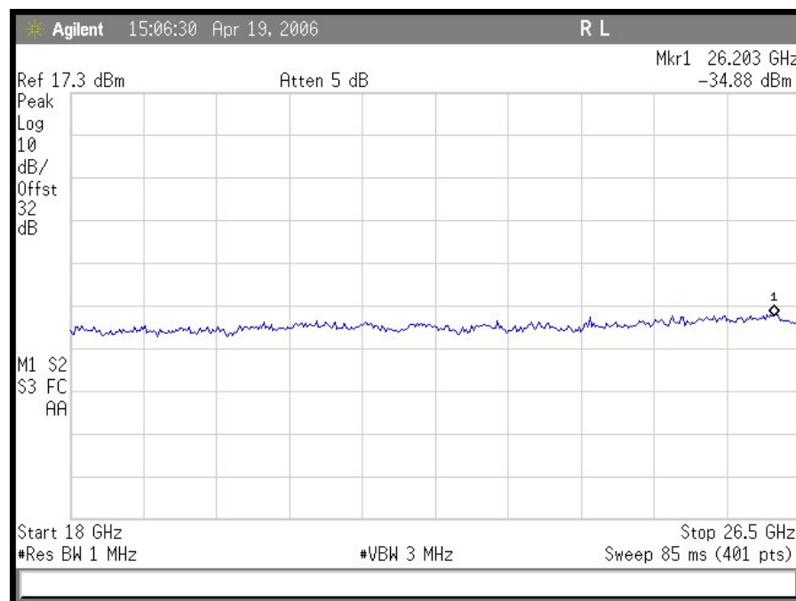
Plot 38. Conducted Spurious Emissions 5 MHz Hi Ch (18 GHz – 26 GHz)
