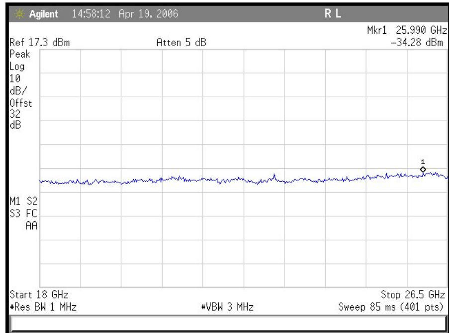
Plot 23. Conducted Spurious Emissions 10 MHz Low Ch (18 GHz – 26 GHz)
