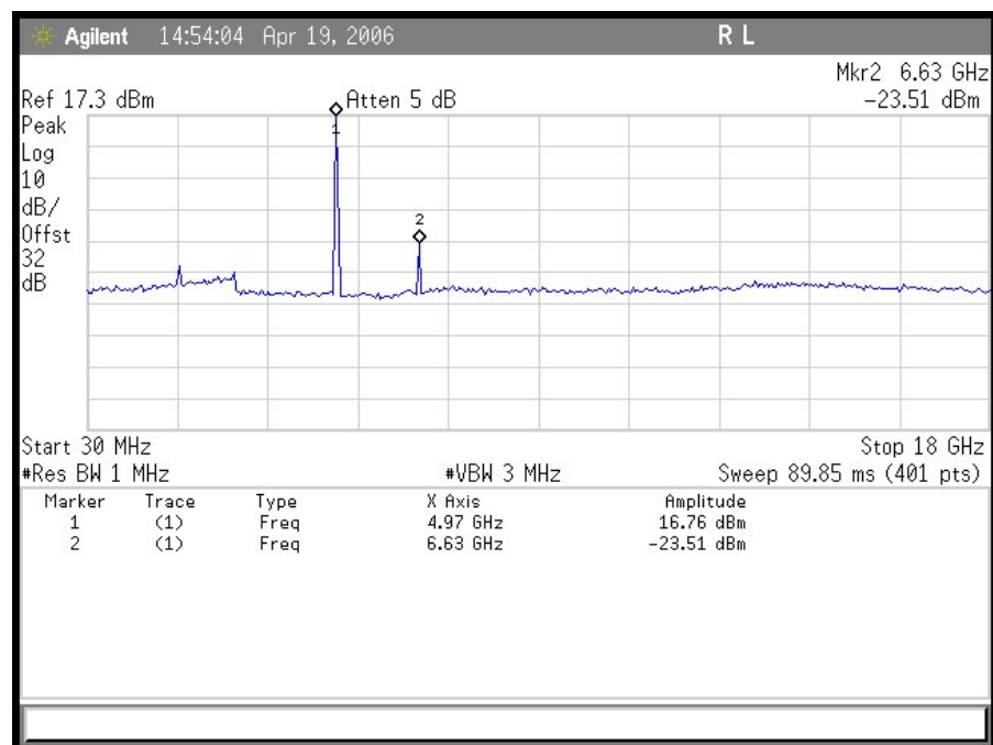
Plot 34. Conducted Spurious Emissions 20 MHz Mid Ch (30 MHz – 18 GHz)
