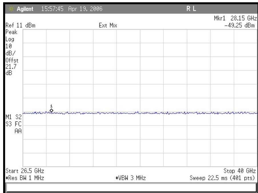
Plot 42. Conducted Spurious Emissions 10 MHz Hi Ch (26.5 GHz – 40 GHz)
