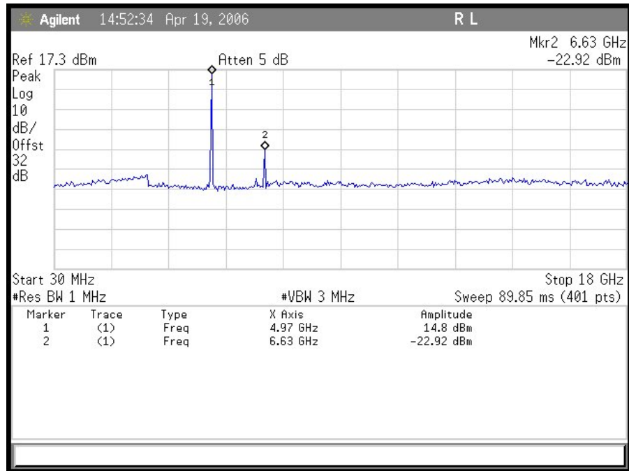
Plot 27. Conducted Spurious Emissions 20 MHz Low Ch (30 MHz – 18 GHz)
