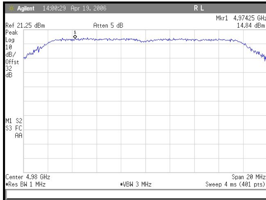
Plot 9. PSD 20 MHz High Ch
