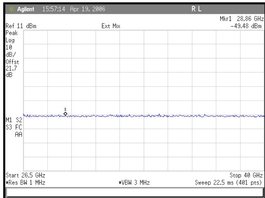
Plot 32. Conducted Spurious Emissions 10 MHz Mid Ch (26.5 GHz – 40 GHz)
