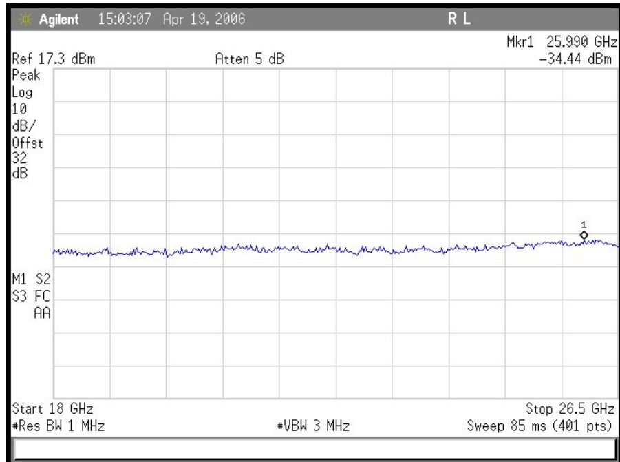
Plot 29. Conducted Spurious Emissions 5 MHz Mid Ch (18 GHz – 26 GHz)
