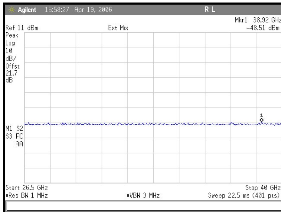
Plot 26. Conducted Spurious Emissions 20 MHz Low Ch (26.5 GHz – 40 GHz)
