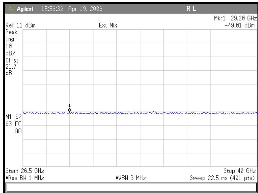
Plot 24. Conducted Spurious Emissions 10 MHz Low Ch (26.5 GHz – 40 GHz)
