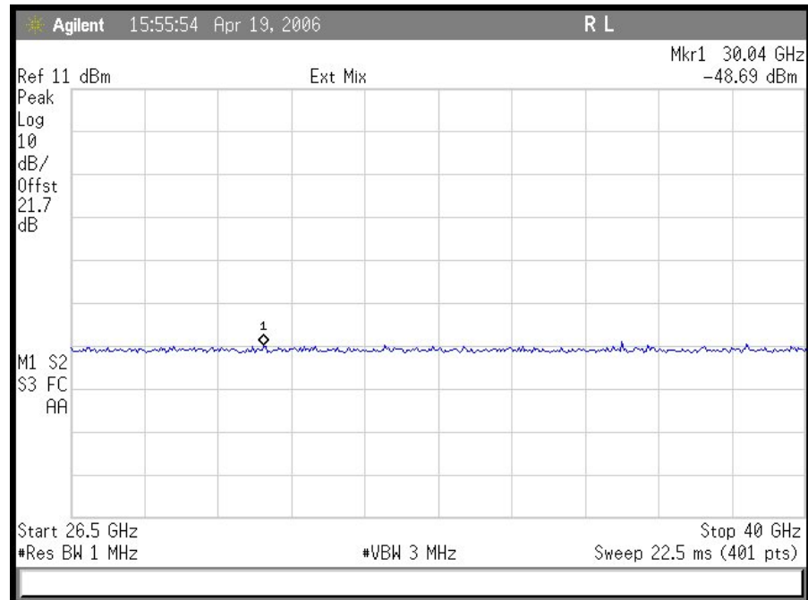
Plot 39. Conducted Spurious Emissions 5 MHz Hi Ch (26.5 GHz – 40 GHz)
