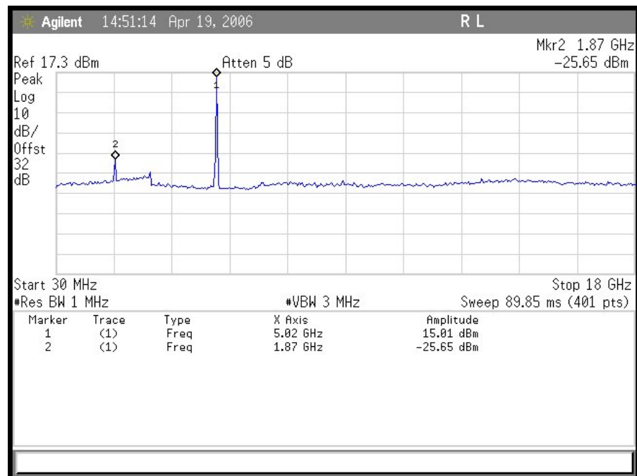
Plot 40. Conducted Spurious Emissions 5 MHz Hi Ch (30 MHz – 18 GHz)
