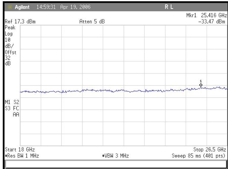
Plot 31. Conducted Spurious Emissions 10 MHz Mid Ch (18 GHz – 26 GHz)
