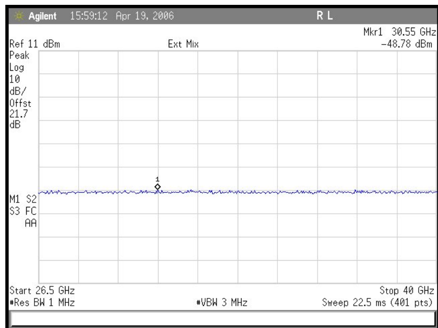
Plot 36. Conducted Spurious Emissions 20 MHz Mid Ch (26.5 GHz – 40 GHz)
