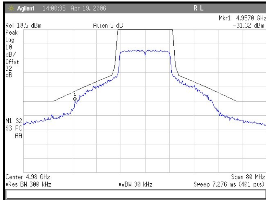
Plot 18. Emission Mask 20 MHz Hi Ch
