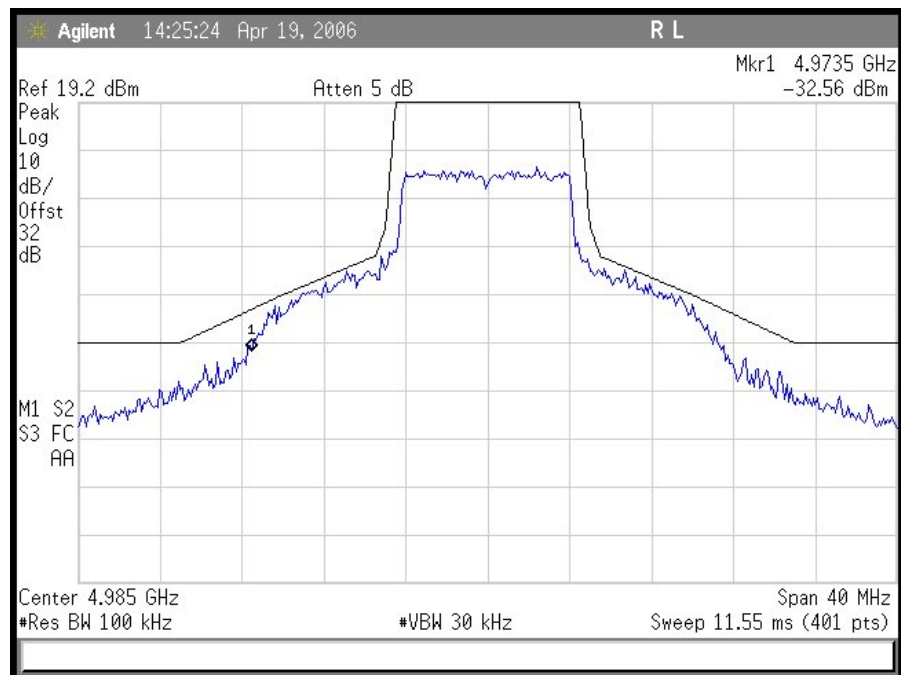
Plot 15. Emission Mask 10 MHz Hi Ch
