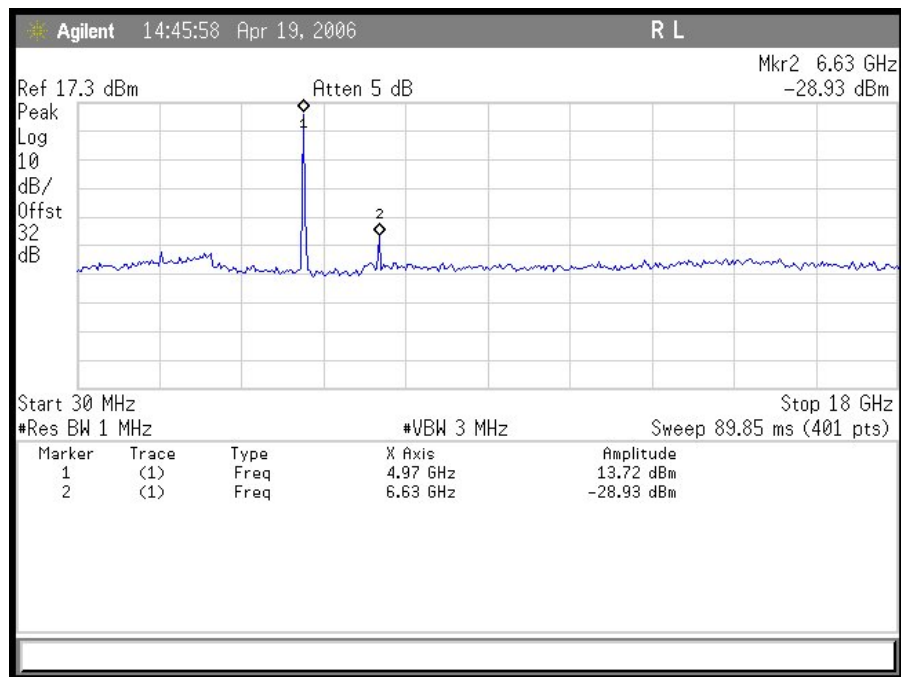
Plot 28. Conducted Spurious Emissions 5 MHz Mid Ch (30 MHz – 18 GHz)
