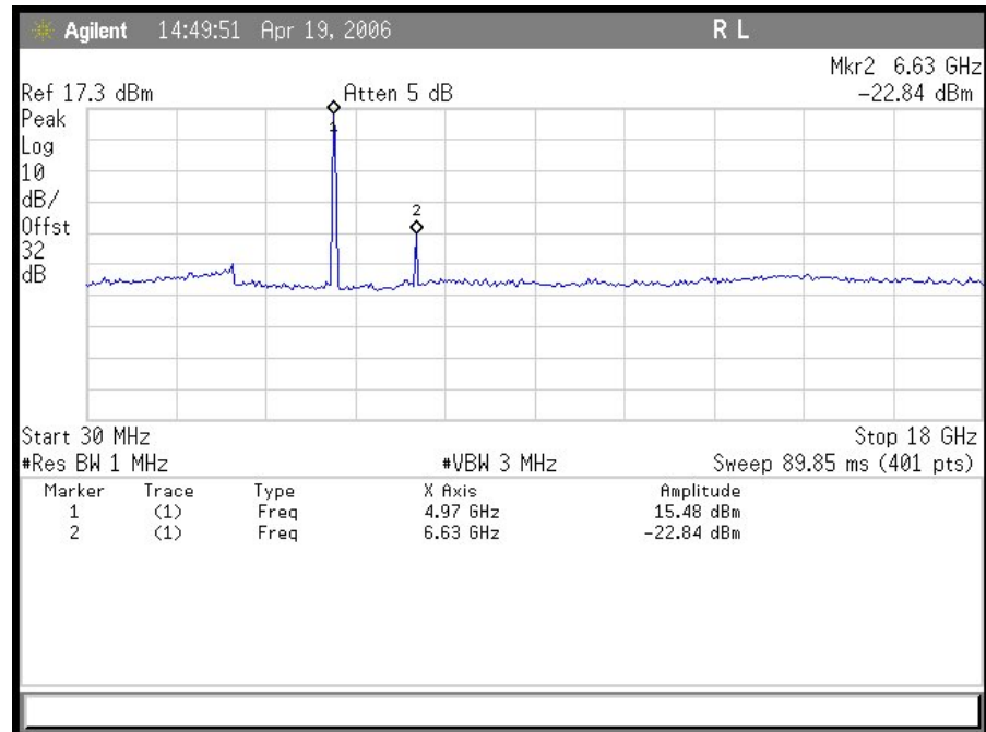
Plot 33. Conducted Spurious Emissions 10 MHz Mid Ch (30 MHz – 18 GHz)
