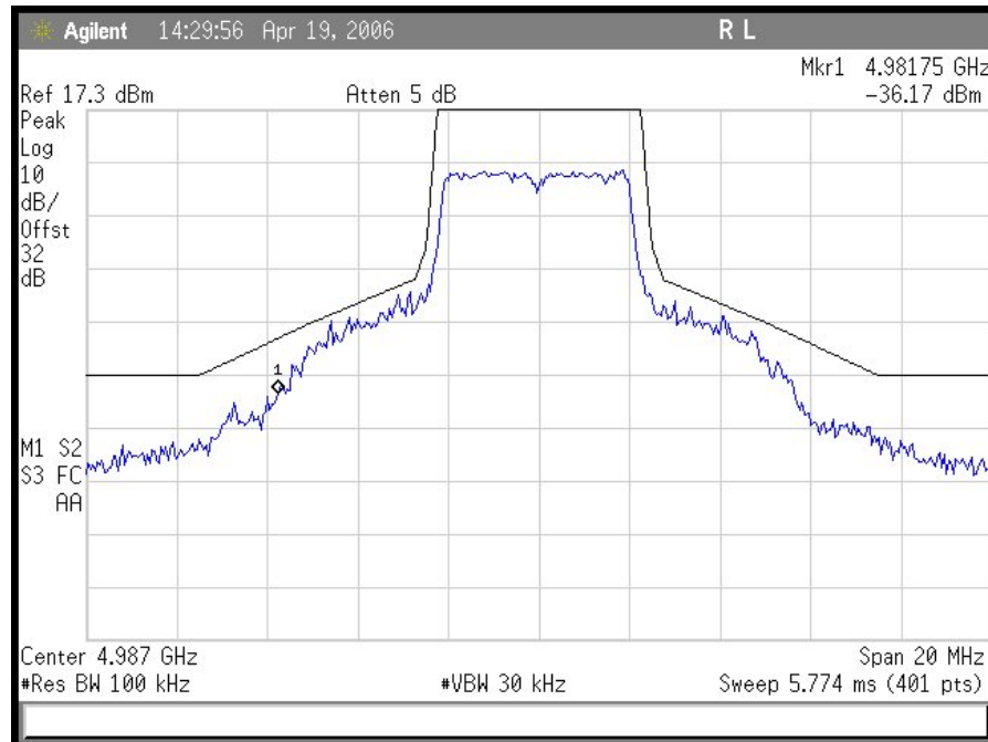
Plot 12. Emission Mask 5 MHz Hi Ch
