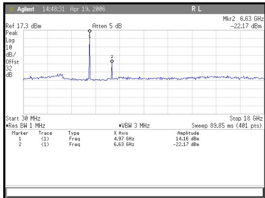
Plot 22. Conducted Spurious Emissions 10 MHz Low Ch (30 MHz – 18 GHz)
