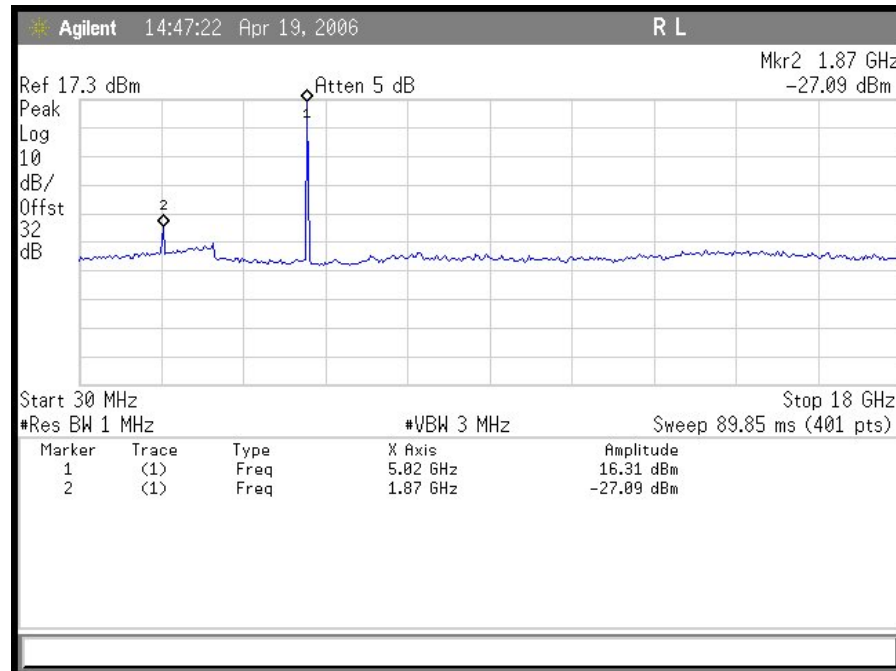
Plot 37. Conducted Spurious Emissions 5 MHz Hi Ch (30 MHz – 18 GHz)
