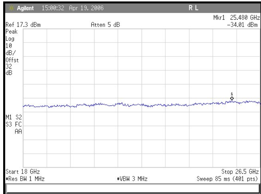
Plot 41. Conducted Spurious Emissions 10 MHz Hi Ch (18 GHz – 26 GHz)
