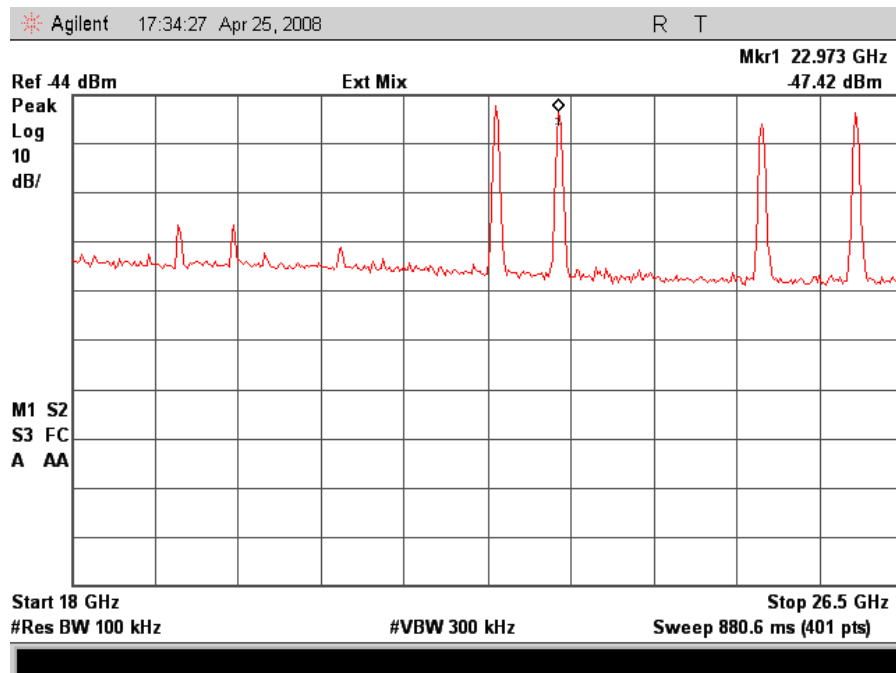
802.11/a – Low Channel Conducted Emissions 18GHz – 26.5GHz
