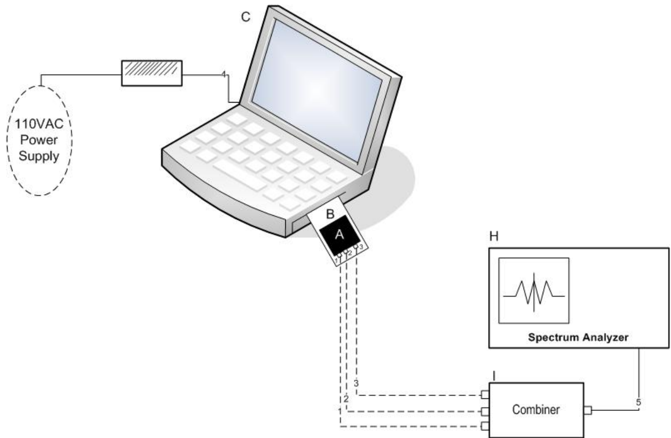
Figure 3. Block Diagram of Test Configuration (Combiner)
