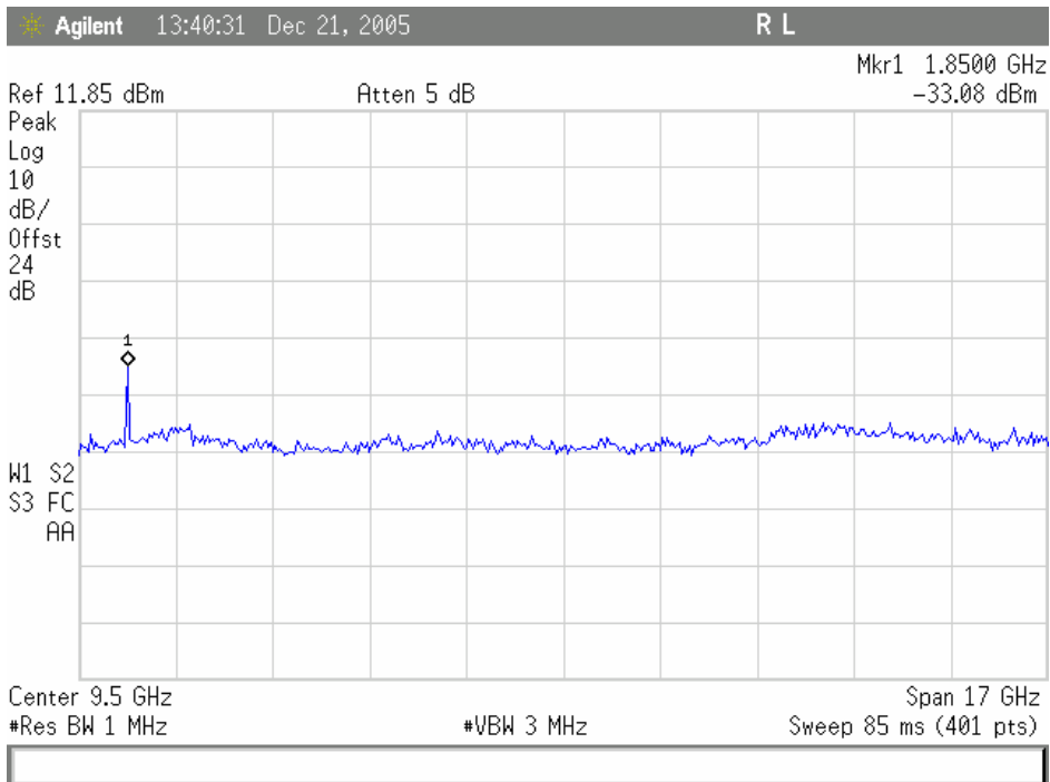
Plot 6. 802.11/b – High Channel Conducted Emissions 1-18GHz
