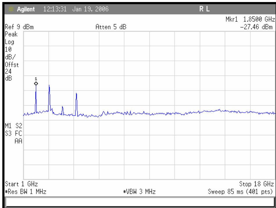
Plot 8. 802.11/g – Low Channel Conducted Emissions 1-18GHz
