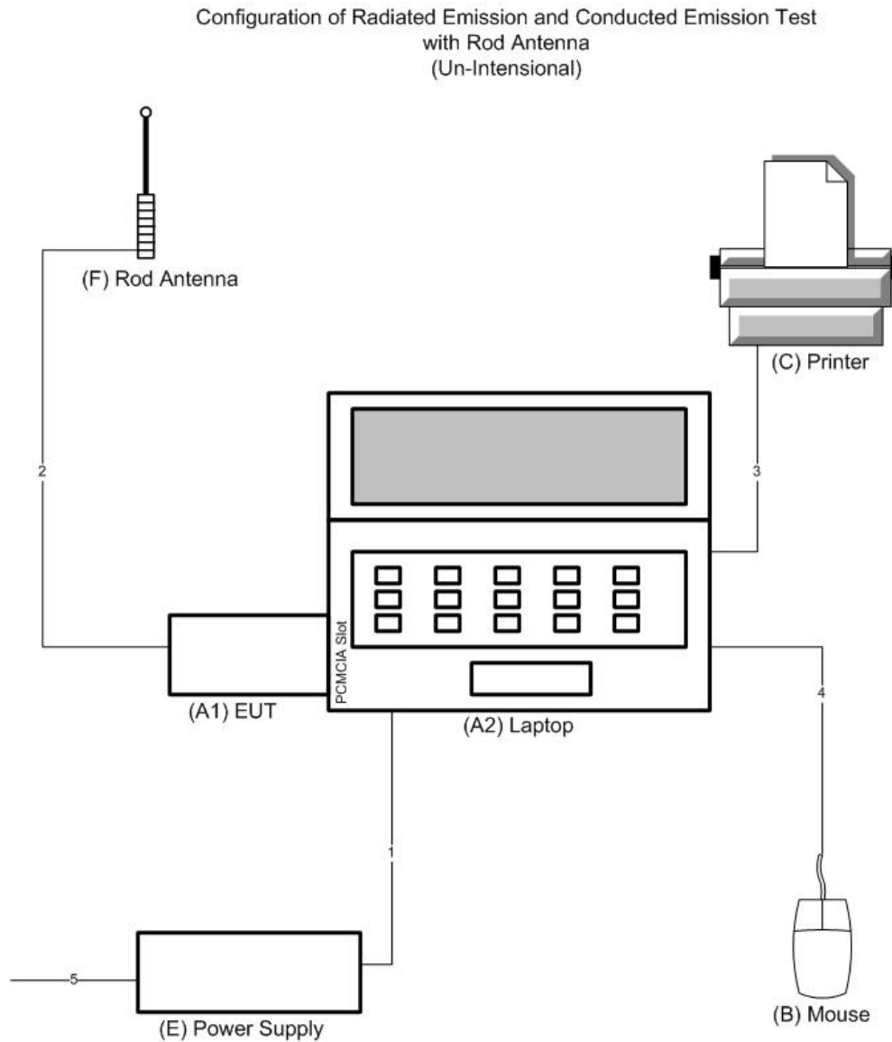
Figure 2. Block Diagram of Test Configuration (Radiated and Conducted Emissions with Rod Antenna)
