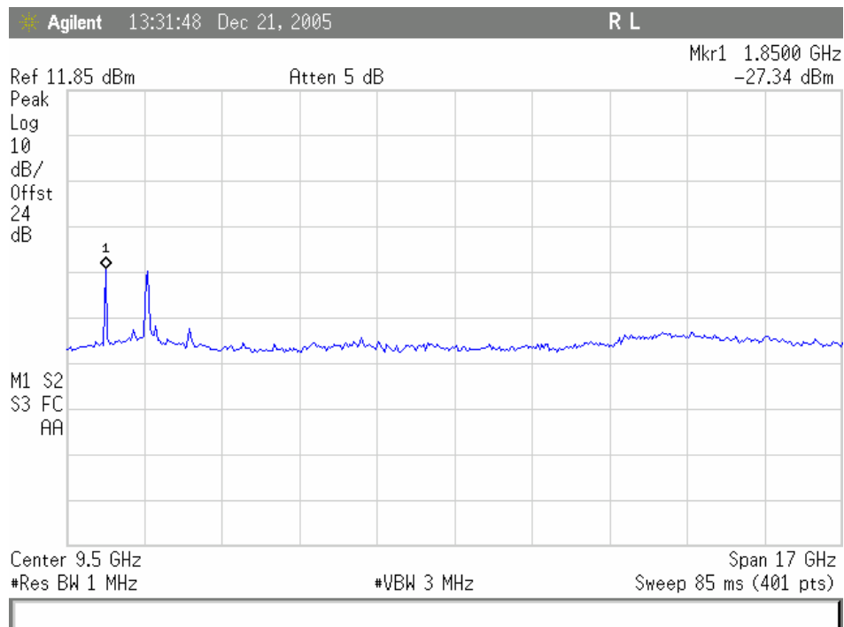
Plot 10. 802.11/g – High Channel Conducted Emissions 1-18GHz
