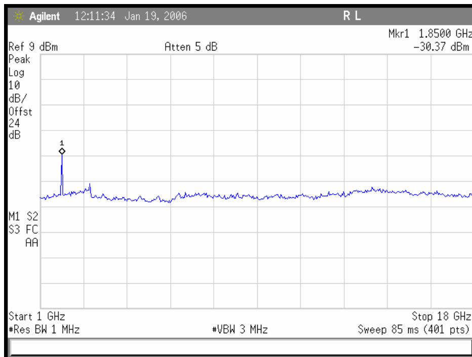
Plot 4. 802.11/b – Low Channel Conducted Emissions 1-18GHz
