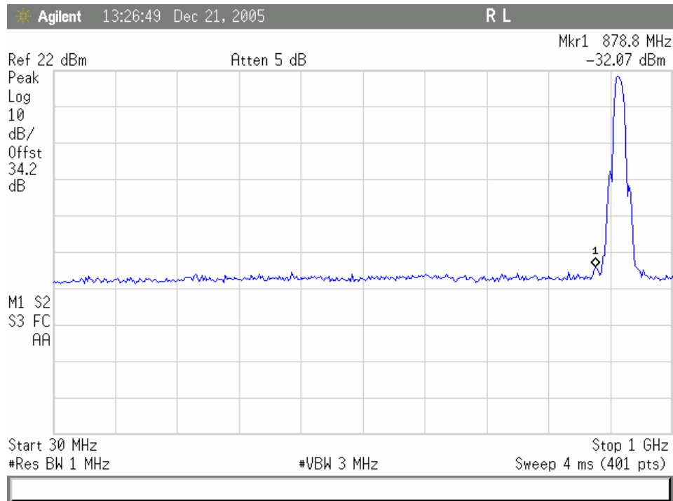
Plot 9. 802.11/g – High Channel Conducted Emissions 30MHz – 1GHz
