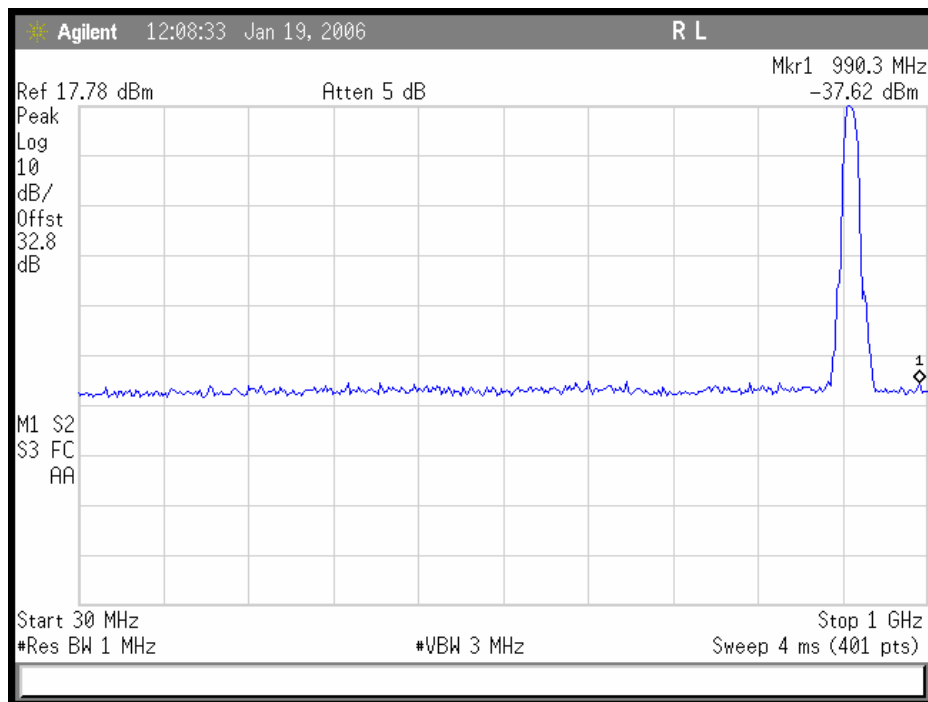
Plot 3. 802.11/b – Low Channel Conducted Emissions 30MHz - 1GHz
