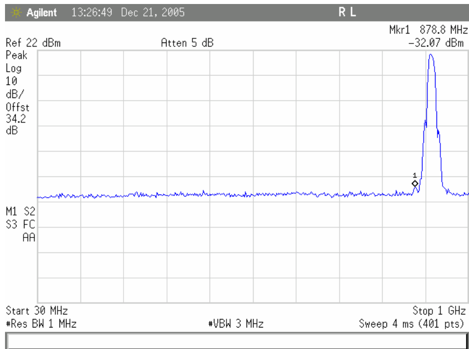
Plot 5. 802.11/b – High Channel Conducted Emissions 30MHz- 1GHz
