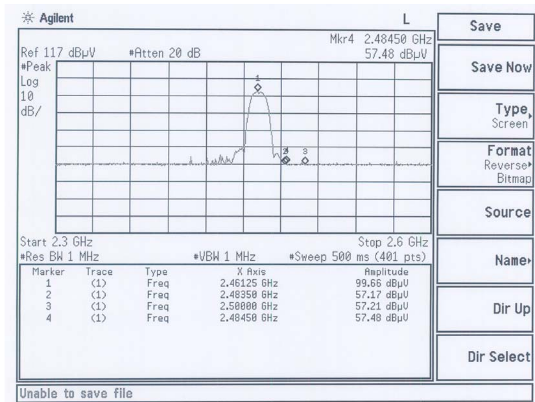
Figure Channel 11: (Horizontal)
