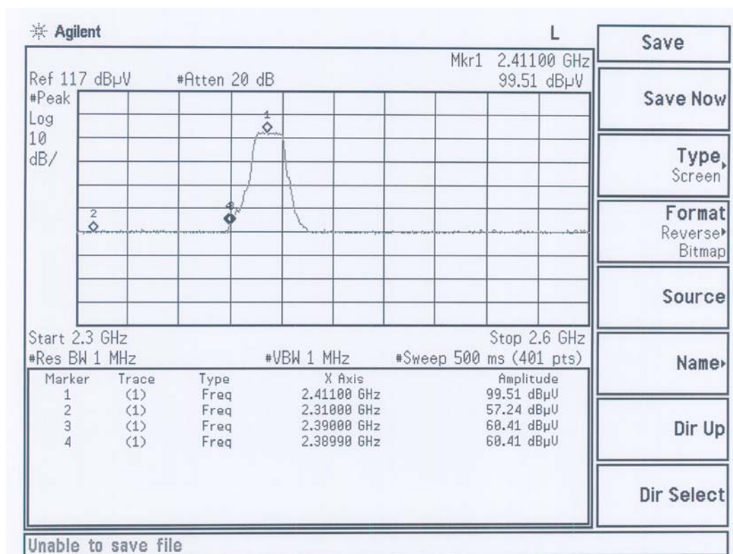
Figure Channel 1: (Horizontal)
