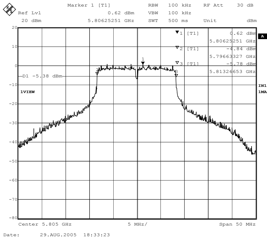
Figure Channel 4: 54Mbps
