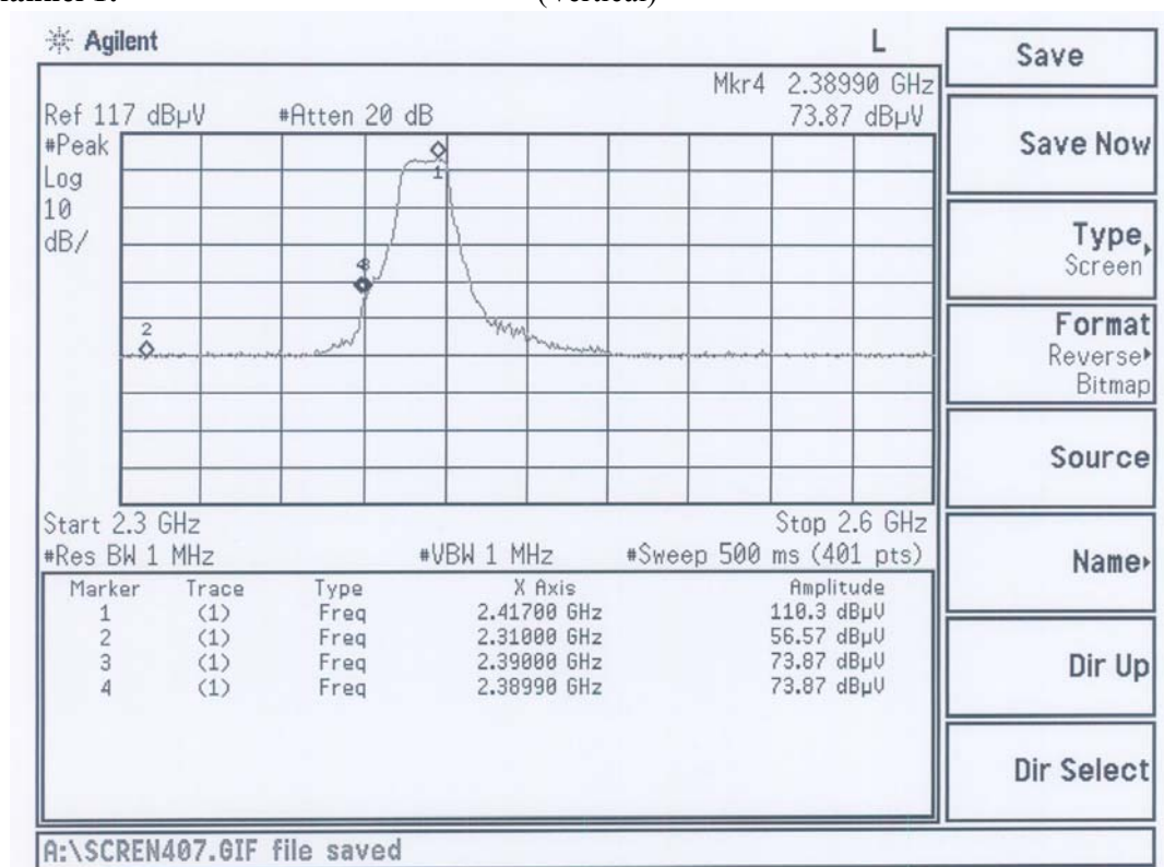
Figure Channel 1: (Vertical)
