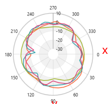
xy-cut
