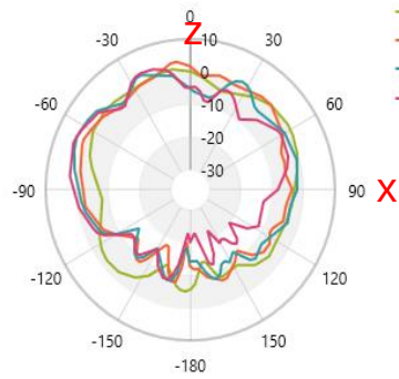
xz-cut
