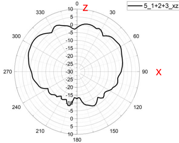
xz cut
