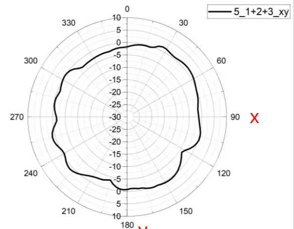
xy cut
