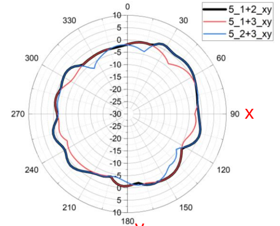
xy cut
