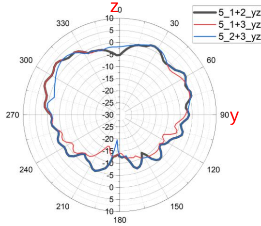
yz cut
