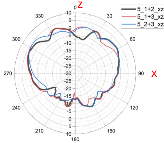
xz cut
