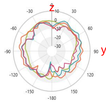
yz-cut
