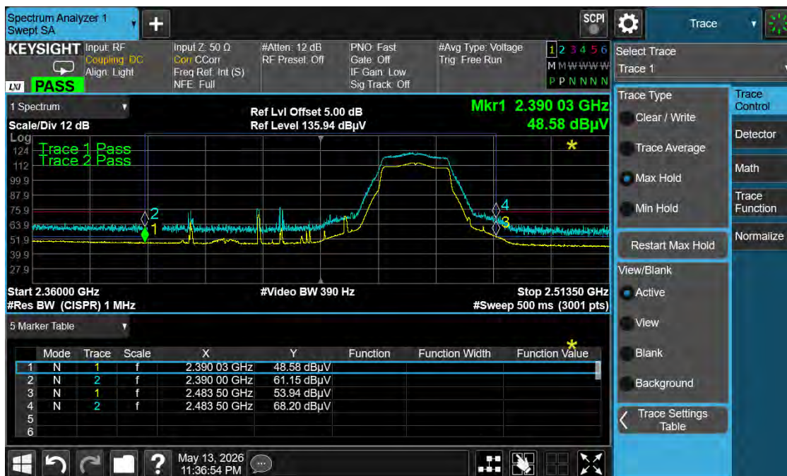
Graph 29: Upper Band Edge Plot – 2462 MHz – n20 Mode
