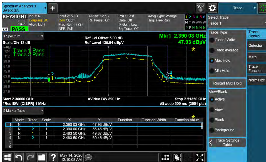
Graph 38: Upper Band Edge Plot – 2452 MHz – be40 Mode
