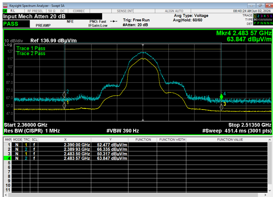
Graph 10: Middle Band Edge Plot – 2437 MHz – n20 Mode
