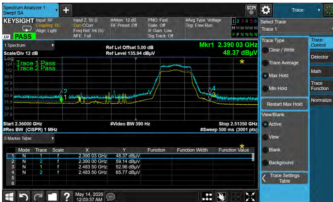
Graph 35: Upper Band Edge Plot – 2462 MHz – be20 Mode
