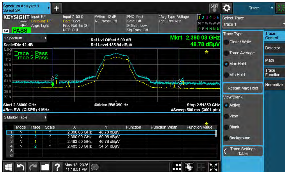
Graph 28: Middle Band Edge Plot – 2437 MHz – n20 Mode
