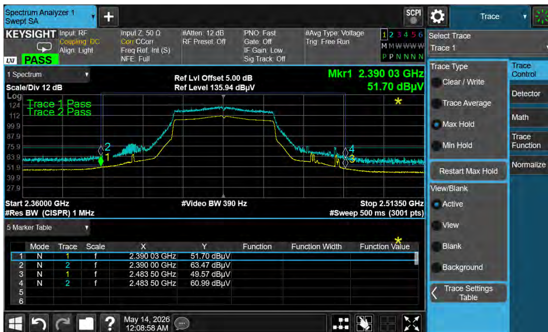
Graph 37: Middle Band Edge Plot – 2437 MHz – be40 Mode
