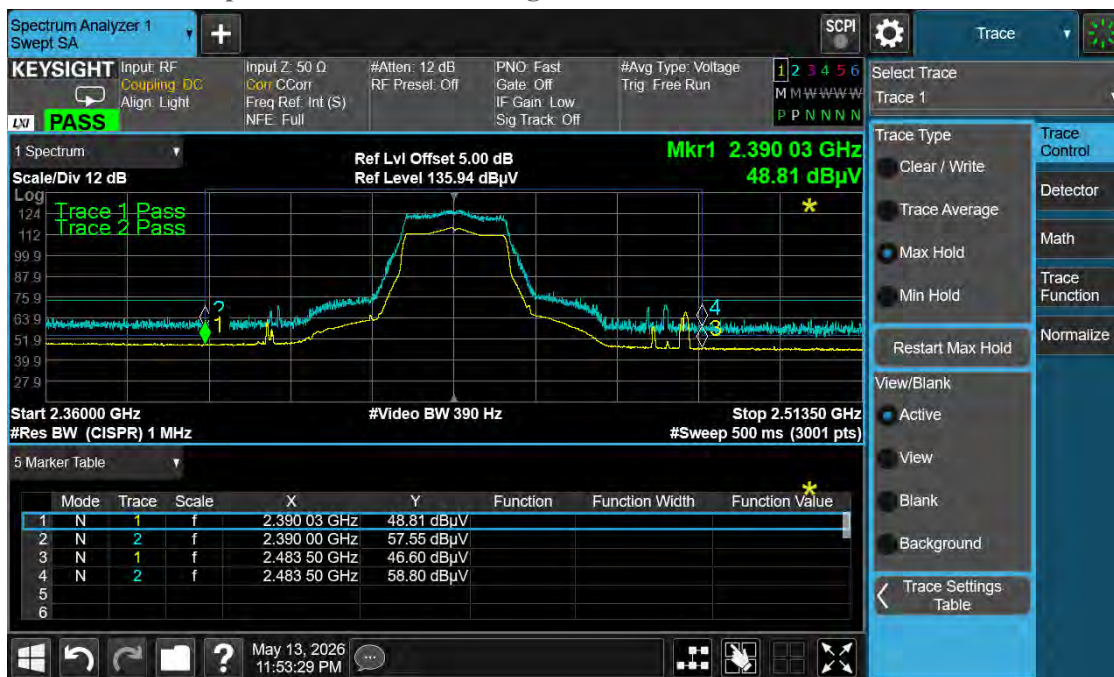
Graph 34: Middle Band Edge Plot – 2437 MHz – be20 Mode
