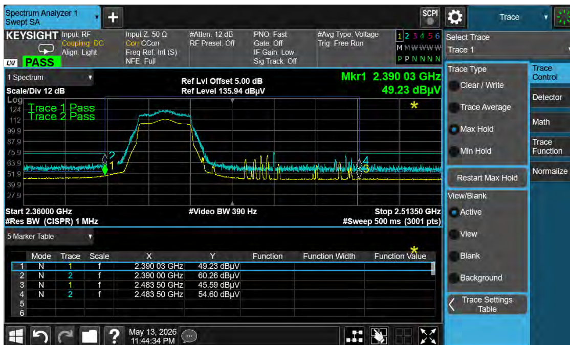
Graph 33: Lower Band Edge Plot – 2412 MHz – be20 Mode
