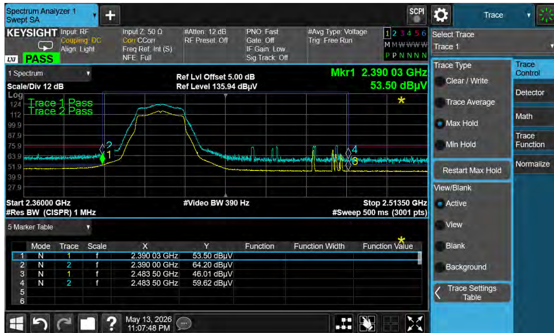
Graph 27: Lower Band Edge Plot – 2412 MHz – n20 Mode
