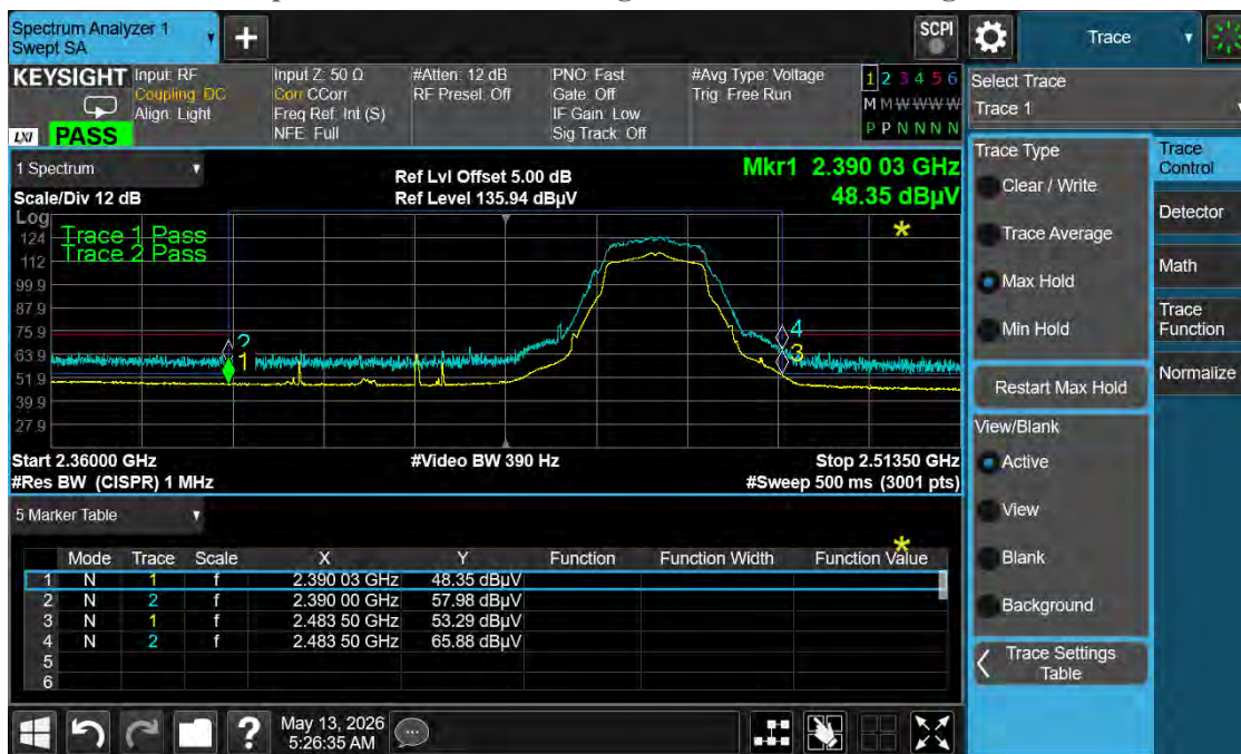
Graph 26: Upper Band Edge Plot – 2462 MHz – g Mode
