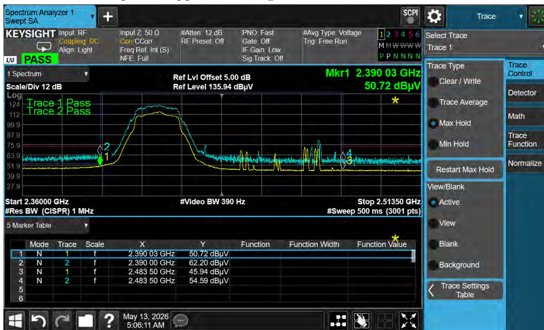
Graph 24: Lower Band Edge Plot – 2412 MHz – g Mode
