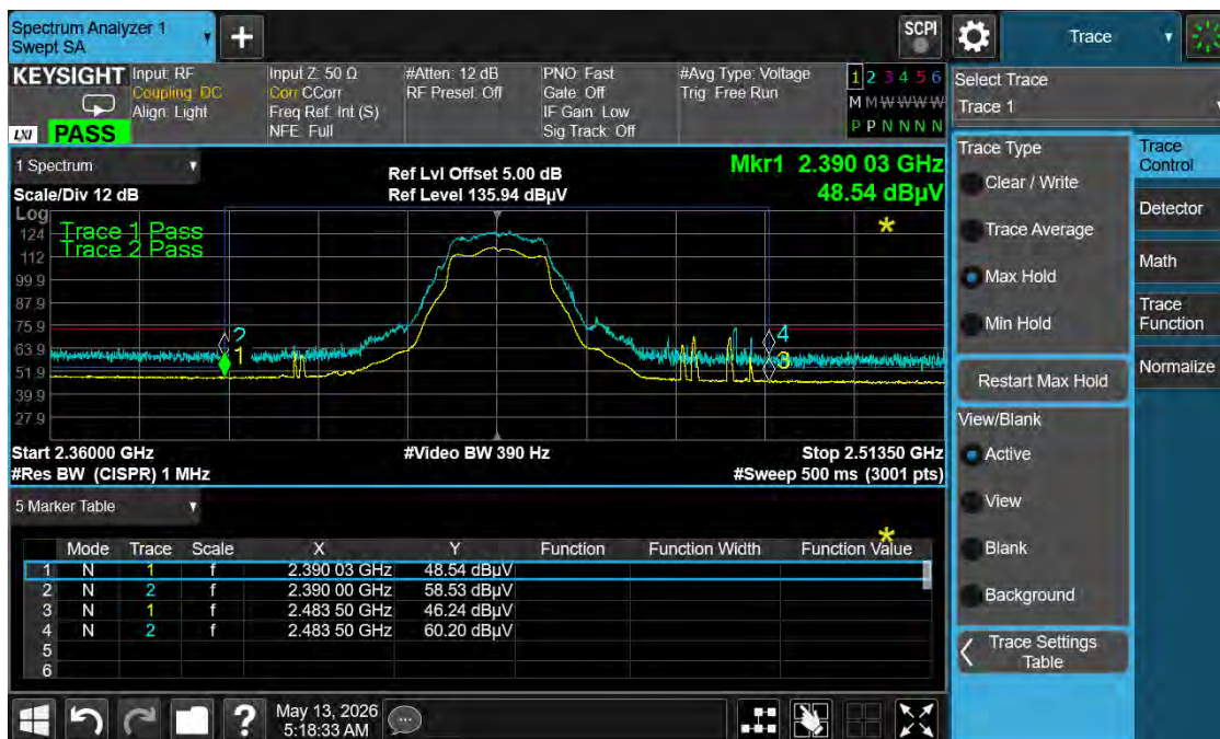
Graph 25: Middle Band Edge Plot – 2437 MHz – g Mode
