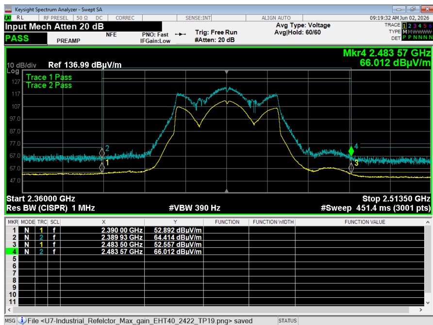
Graph 19: Middle Band Edge Plot – 2437 MHz – be40 Mode
