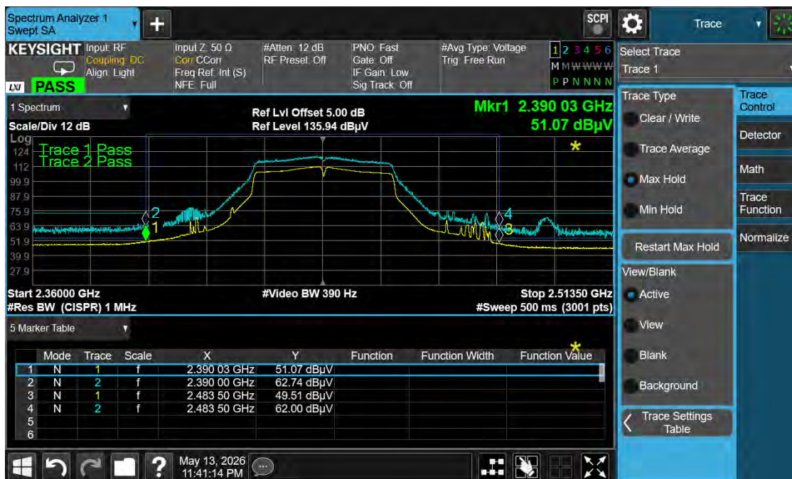
Graph 31: Middle Band Edge Plot – 2437 MHz – n40 Mode
