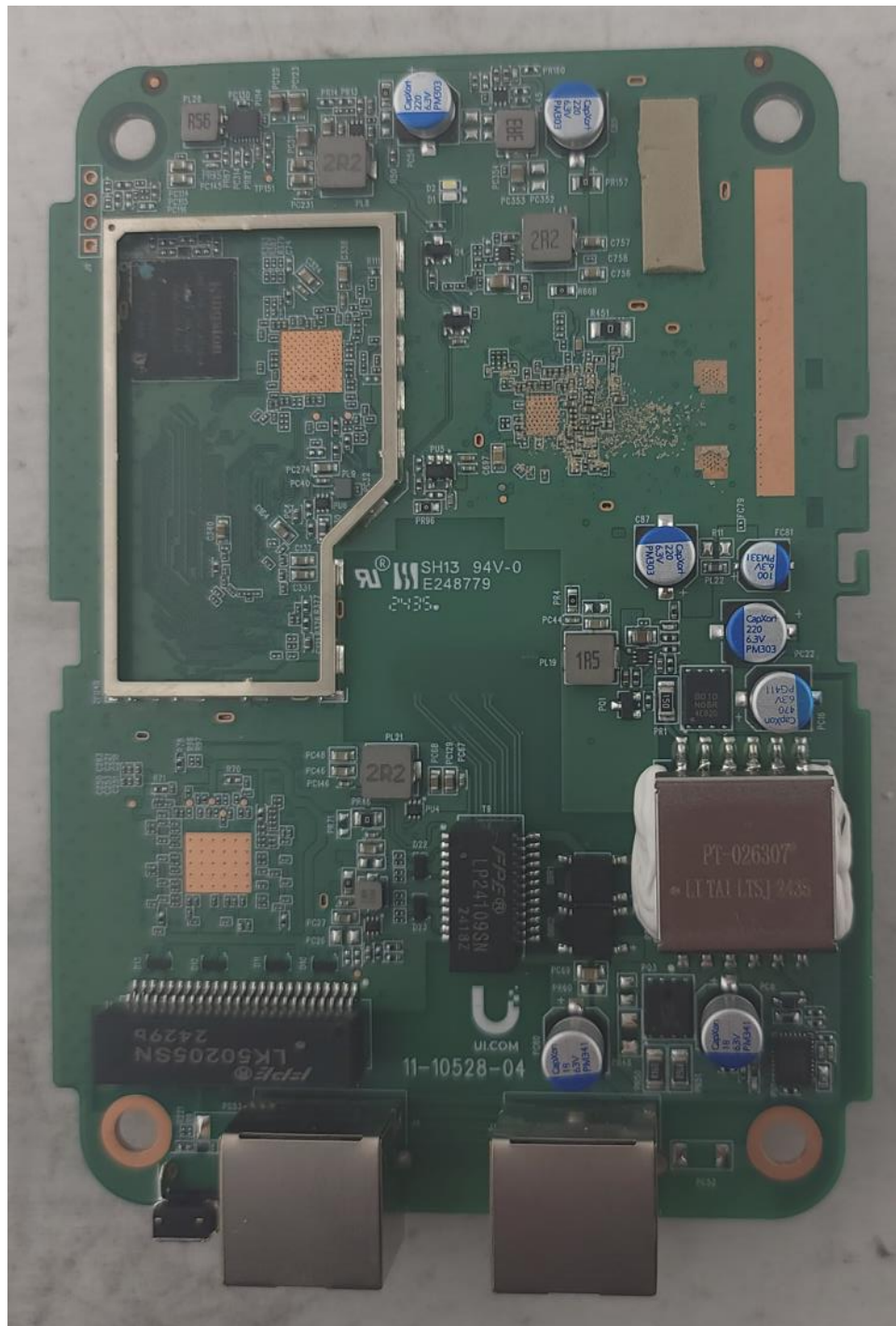
Photograph 6: Front Side of PCB with Can Off
