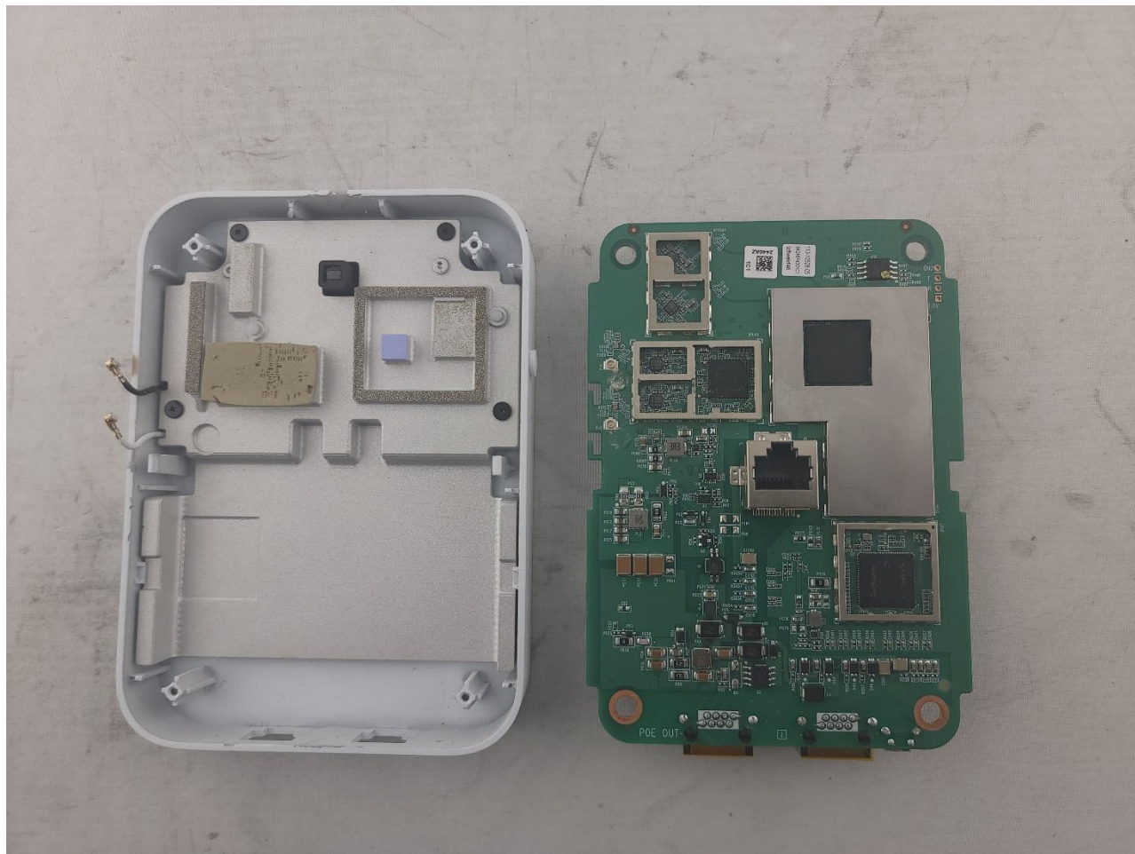
Photograph 2: Main PCB Outside Housing
