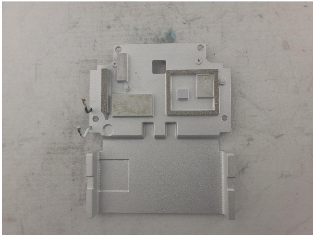
Photograph 7: Back of Antenna Board
