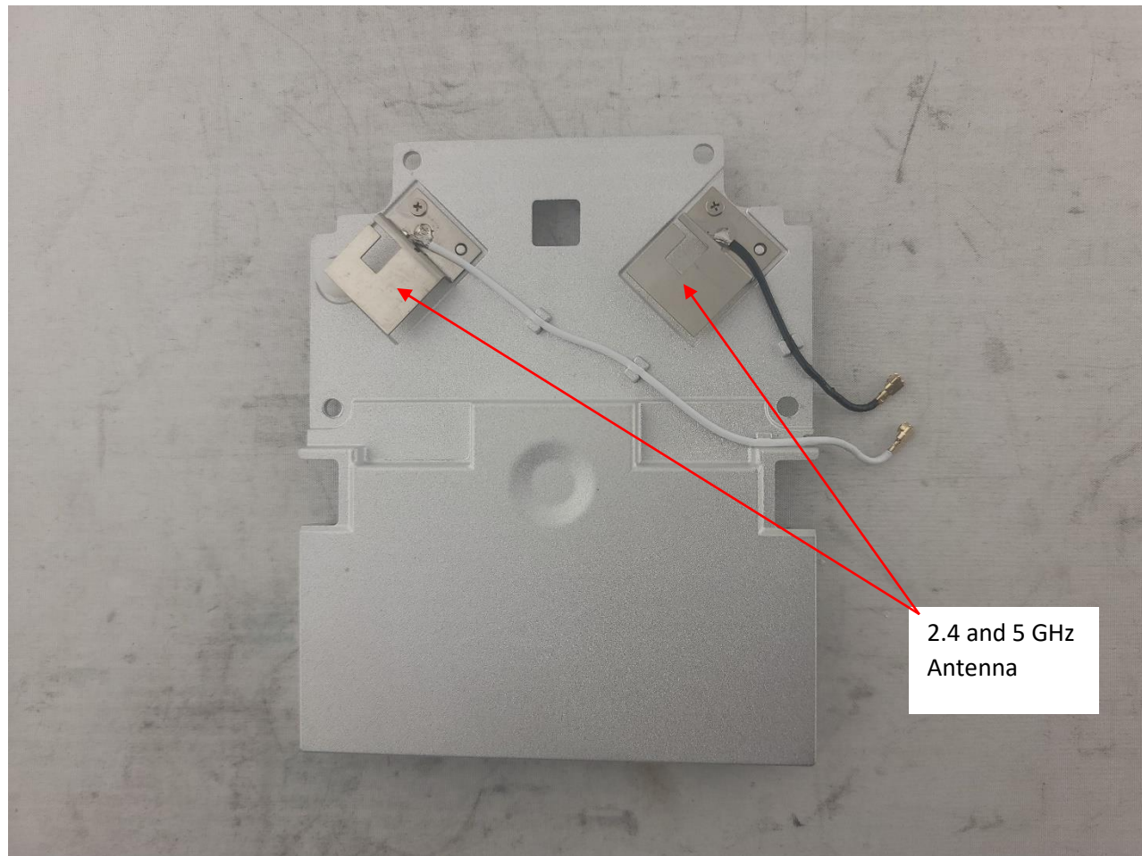
Photograph 8: Front of Antenna Board
