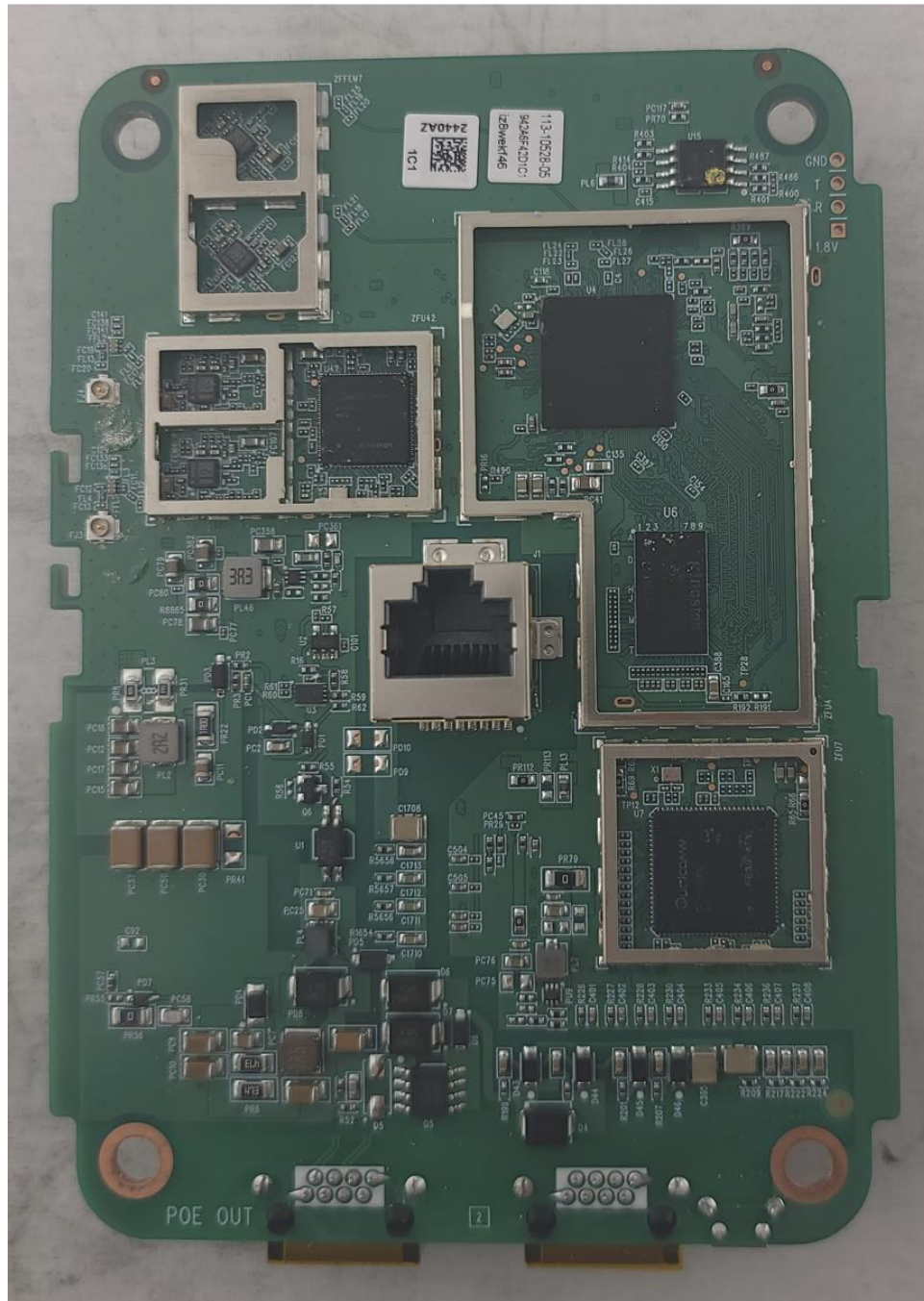
Photograph 5: Back Side of PCB with Can Off
