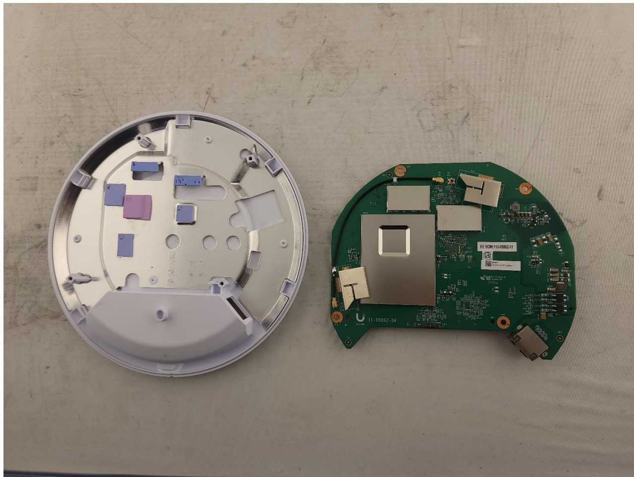
Photograph 3: Internal View of Main PCB Removed From Back Housing
