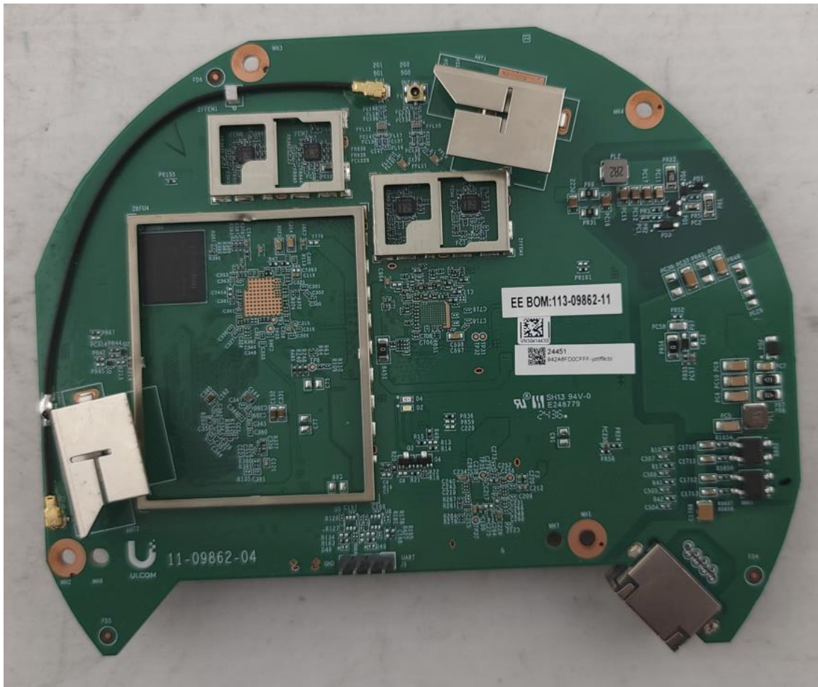
Photograph 5: Top Side of Main PCB w/Cans Off
