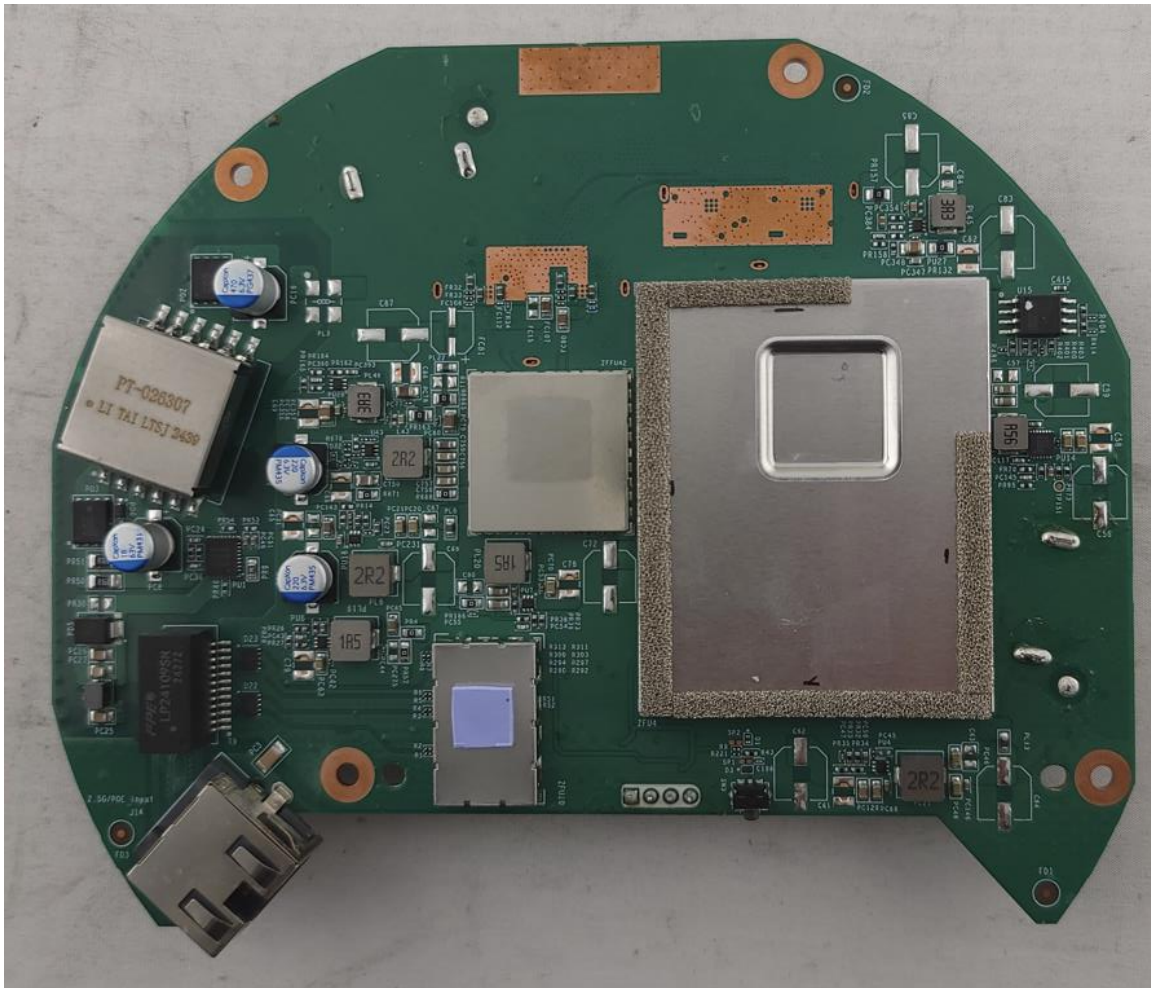
Photograph 6: Bottom Side of Main PCB w/Cans On
