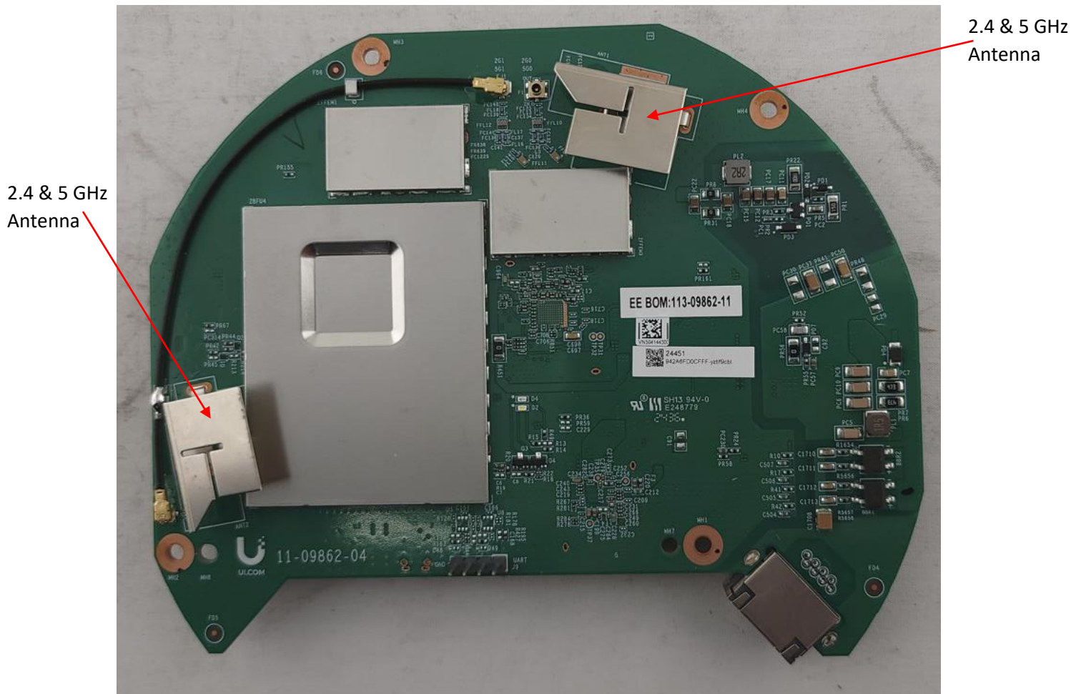
Photograph 4: Top Side of Main PCB w/Cans On
