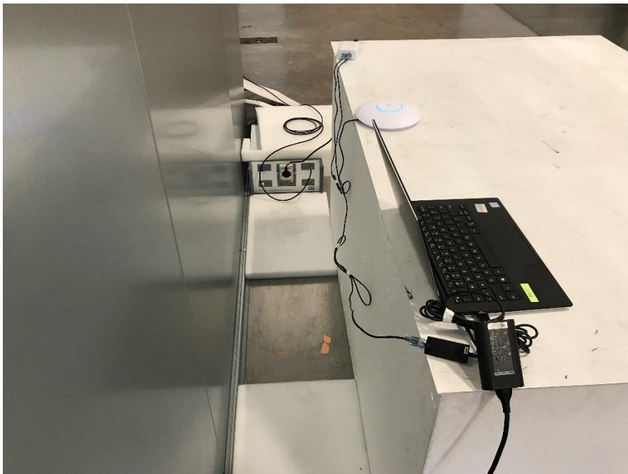
Photograph 8: View Test Set Up Back Conducted Emissions
