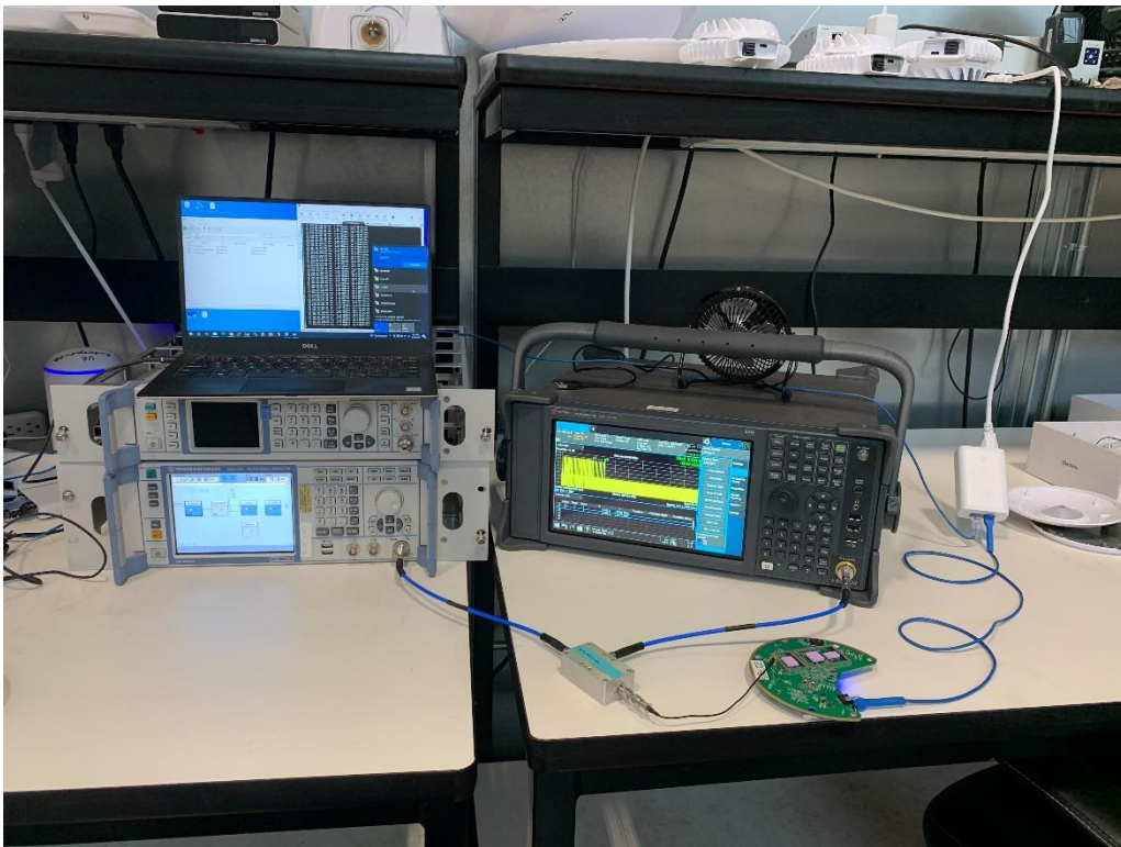
Photograph 6: View Test Set Up DFS
