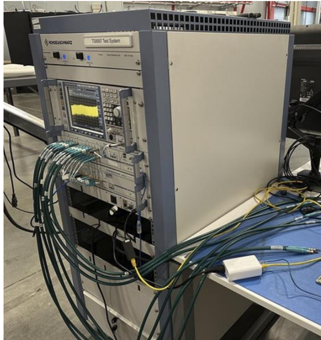
Photograph 5: View Test Set Up RF Conducted Showing Test Rack
