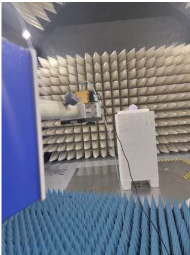
Photograph 3: View Test Set Up Radiated Emissions 17 – 40 GHz
