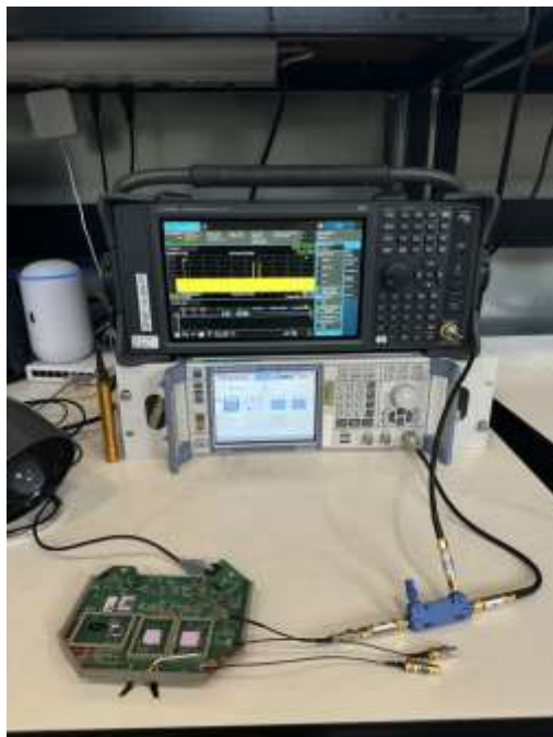
Photograph 5: View Test Set Up DFS
