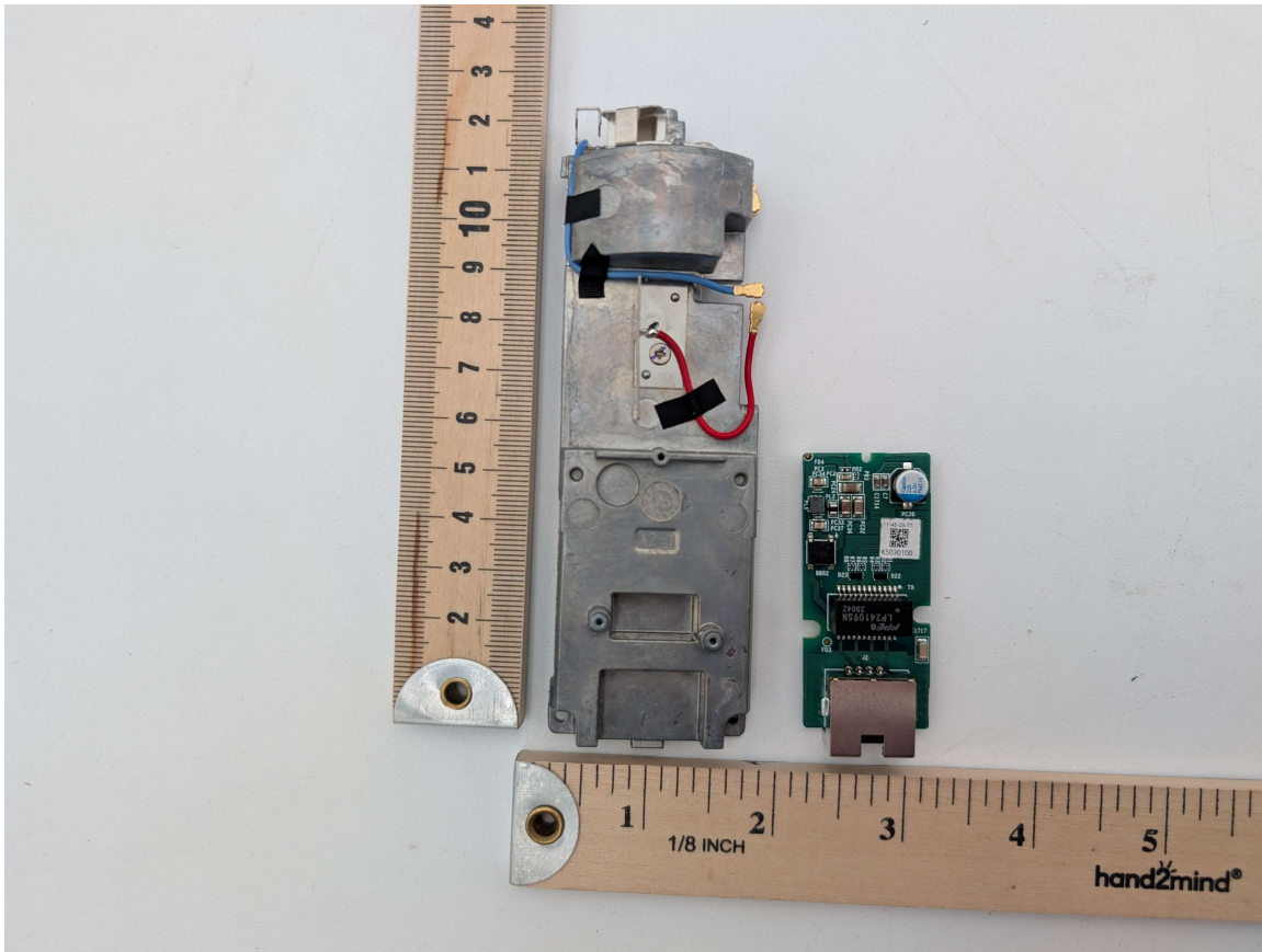
Photograph 13: Back Section w/ PoE PCB Removed
