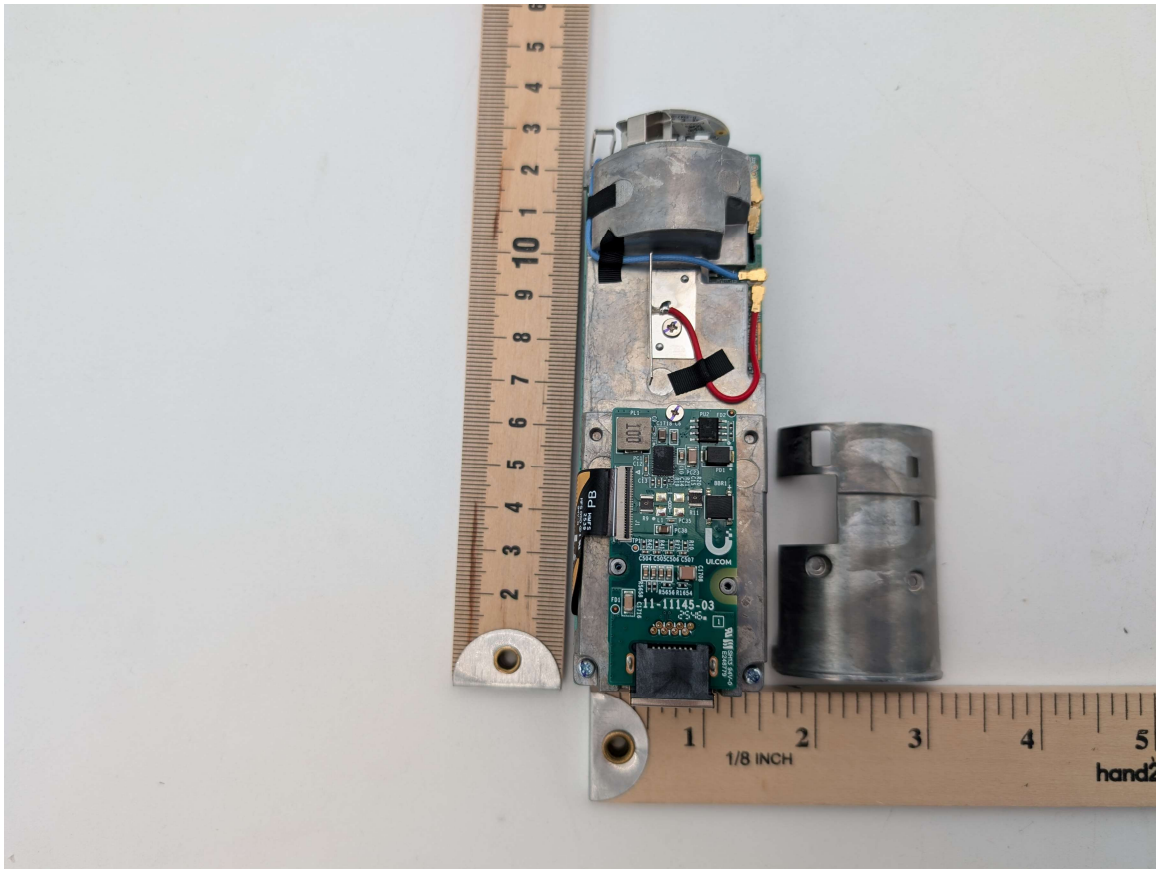
Photograph 9: Internal Assembly Back Cover Off
