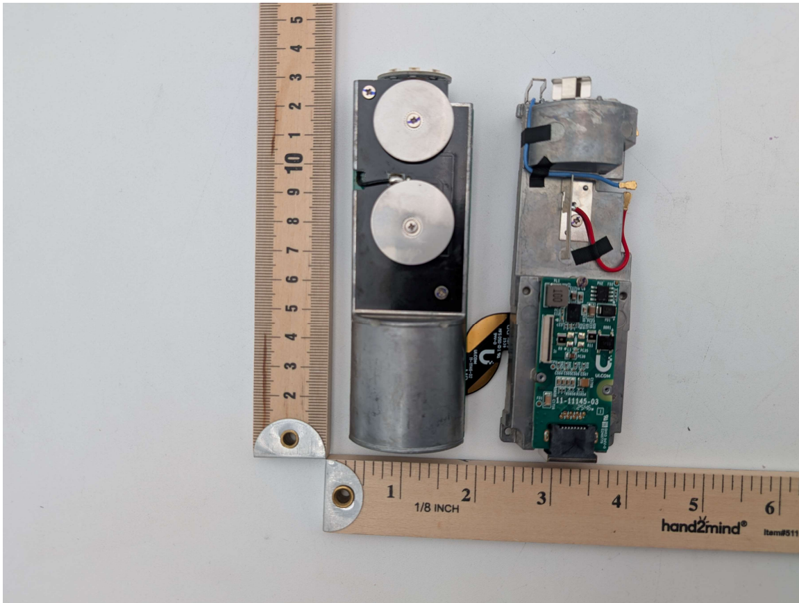
Photograph 12: Internal Assembly Outside Front/Back Sections Removed
