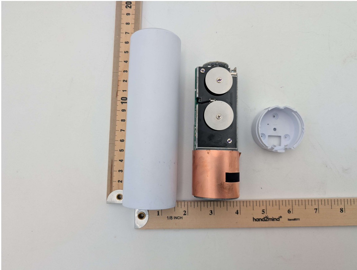
Photograph 1: Internal Assembly Out of Shell w/ Bottom Cap
