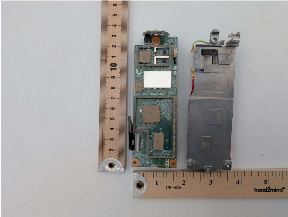
Photograph 11: Internal Assembly Inside Front/Back Sections Removed
