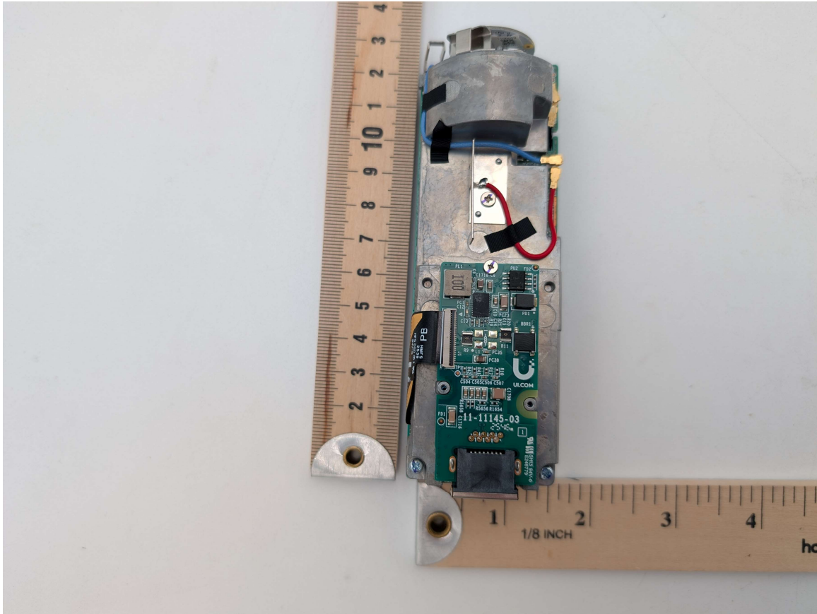
Photograph 10: Internal Assembly Back w/o Cover
