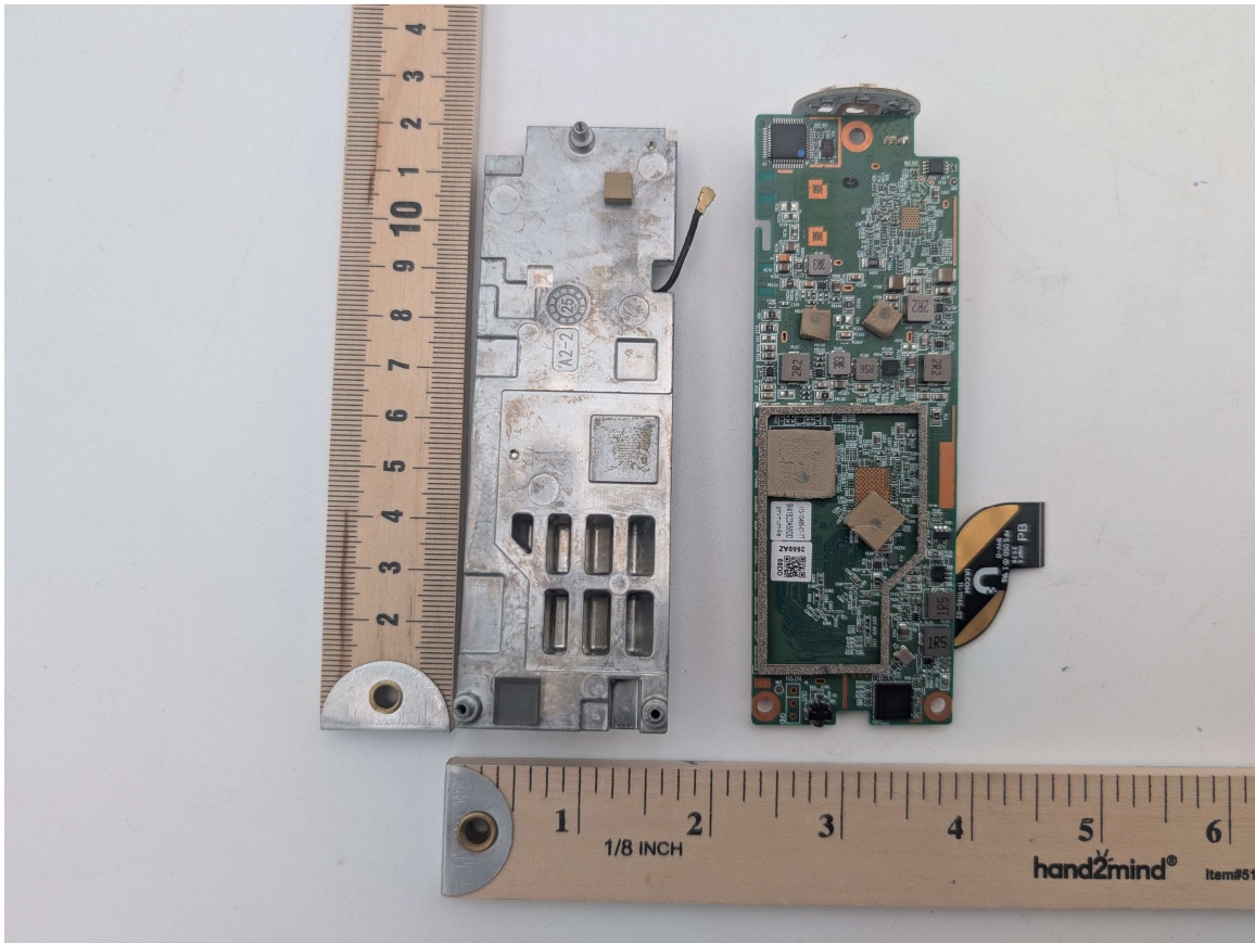
Photograph 3: Main PCB Removed From Front Assembly
