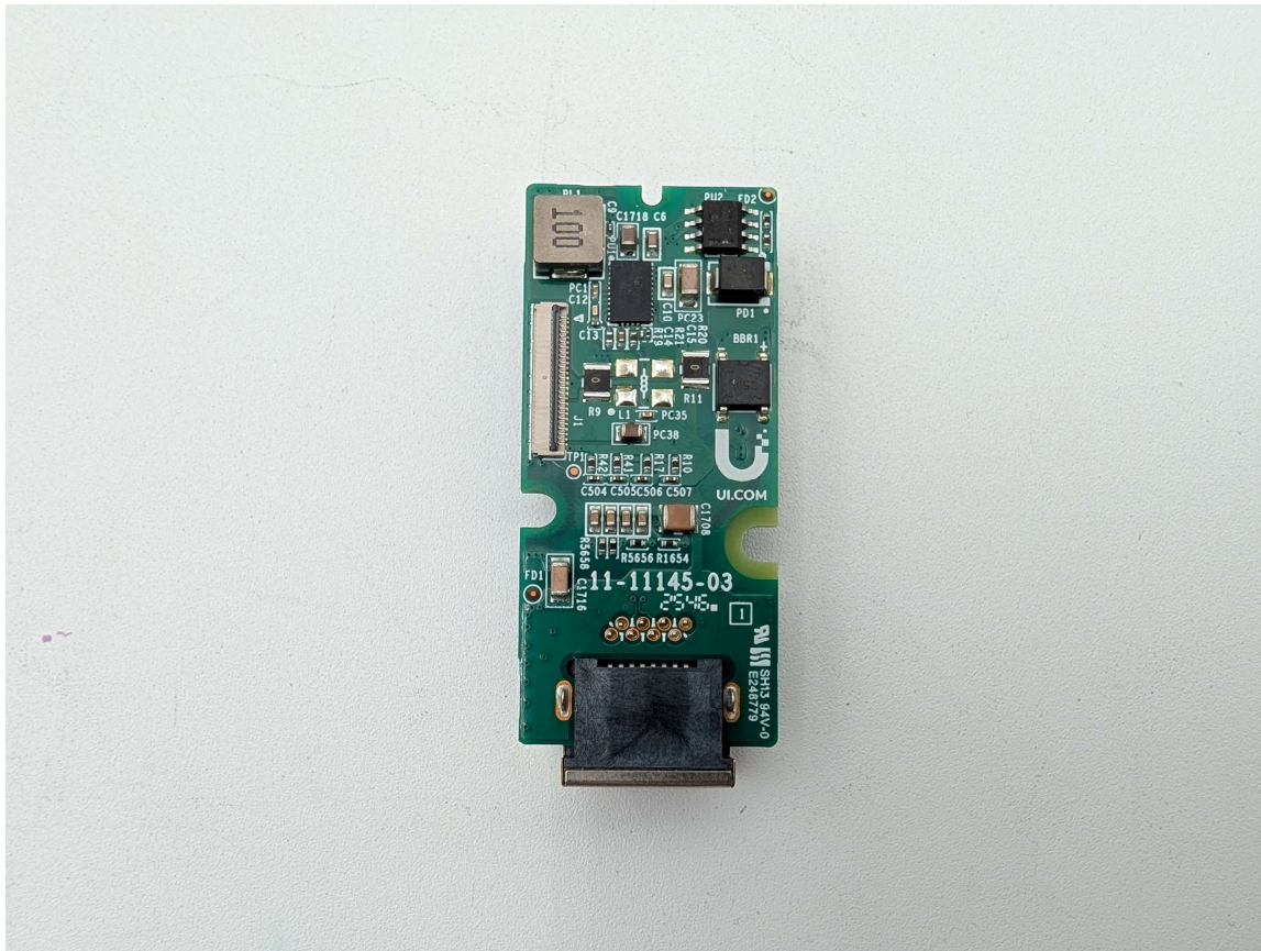
Photograph 2: PoE PCB Back
