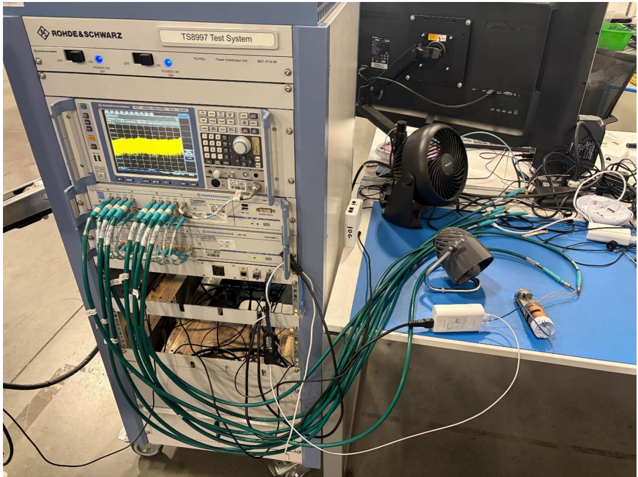
Photograph 4: View Test Set Up RF Conducted
