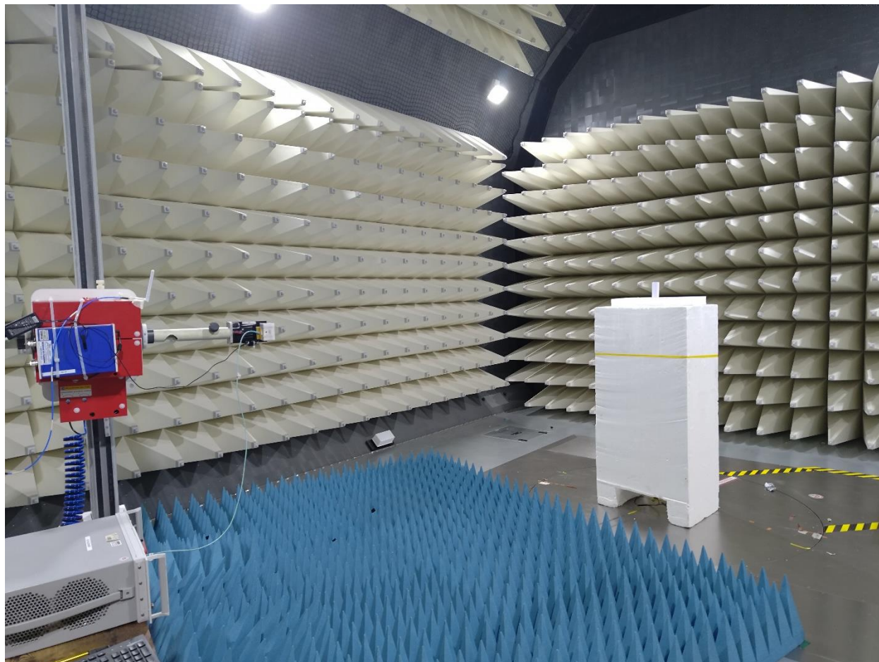
Photograph 3: View Test Set Up Radiated Emissions 17 – 40 GHz
