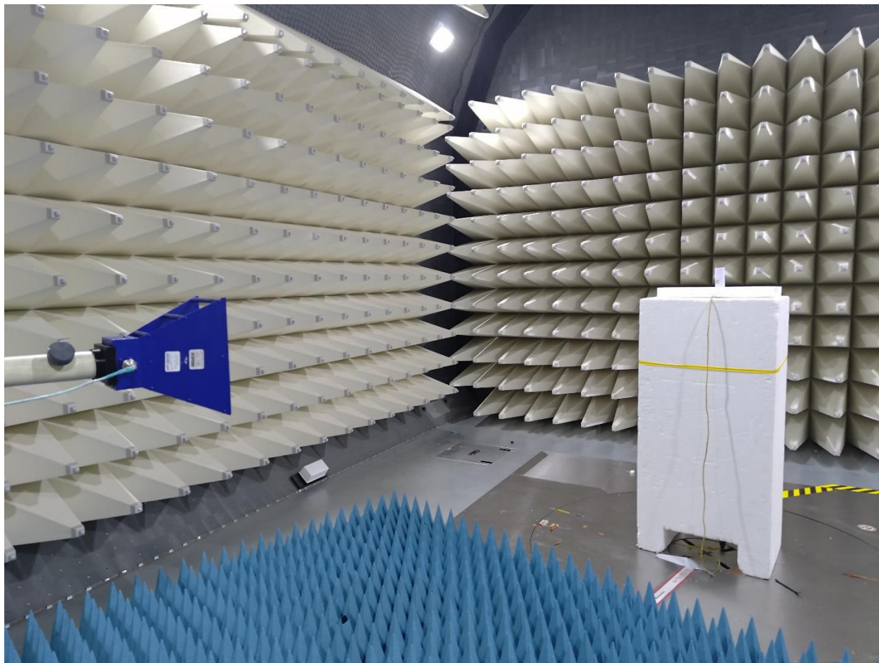
Photograph 2: View Test Set Up Radiated Emissions 1 – 17 GHz
