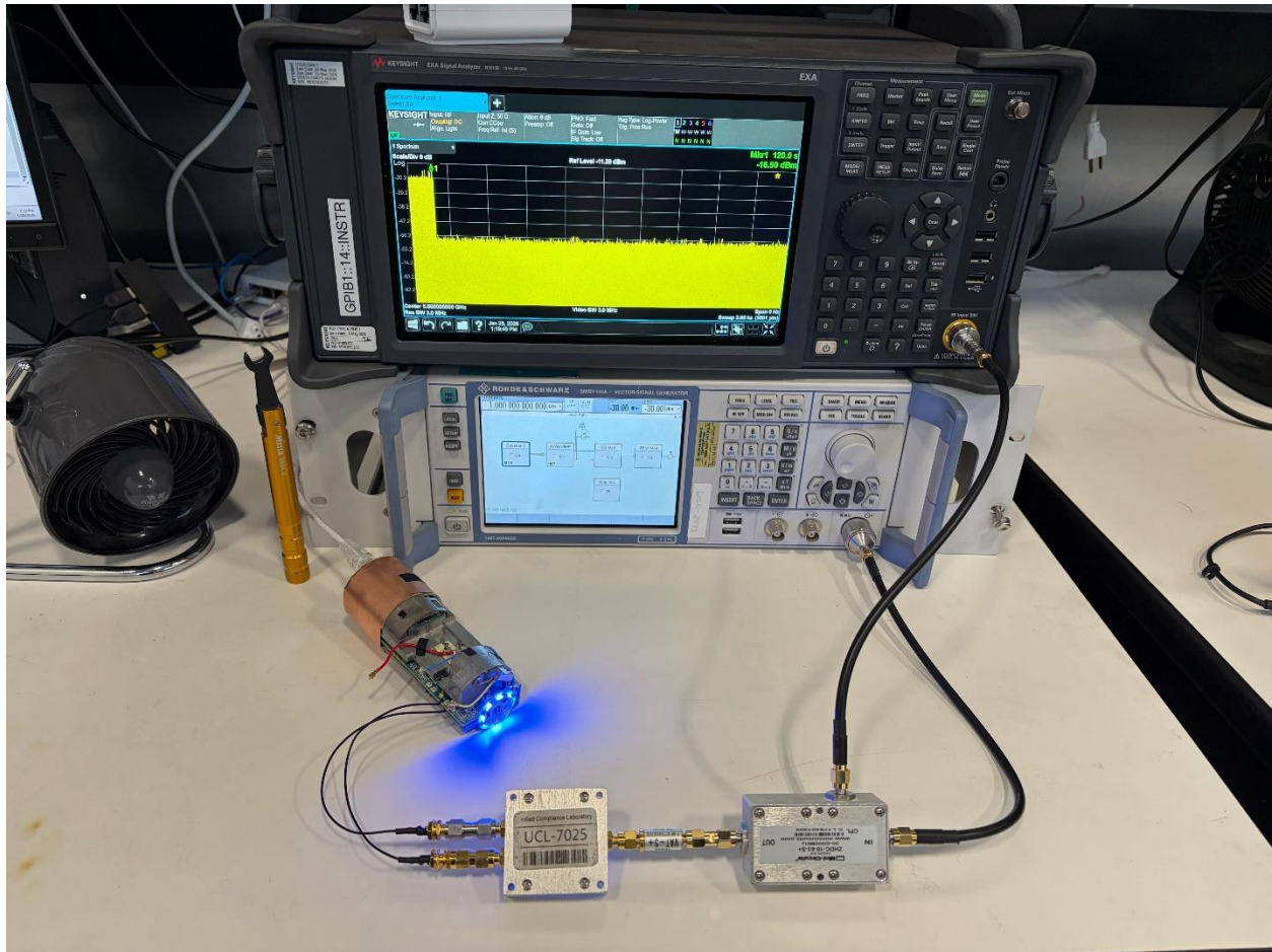
Photograph 5: View Test Set Up DFS
