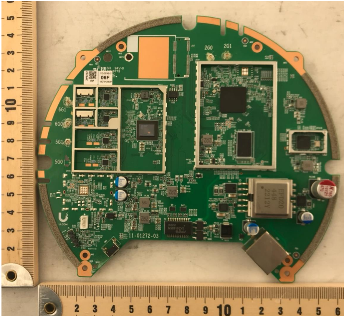
Photograph 5: Top View of the PCB with Cans Off
