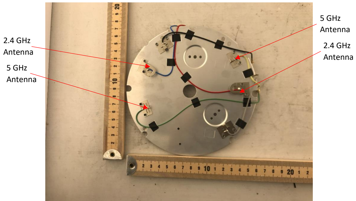
Photograph 7: Top View of the Antenna Configuration
