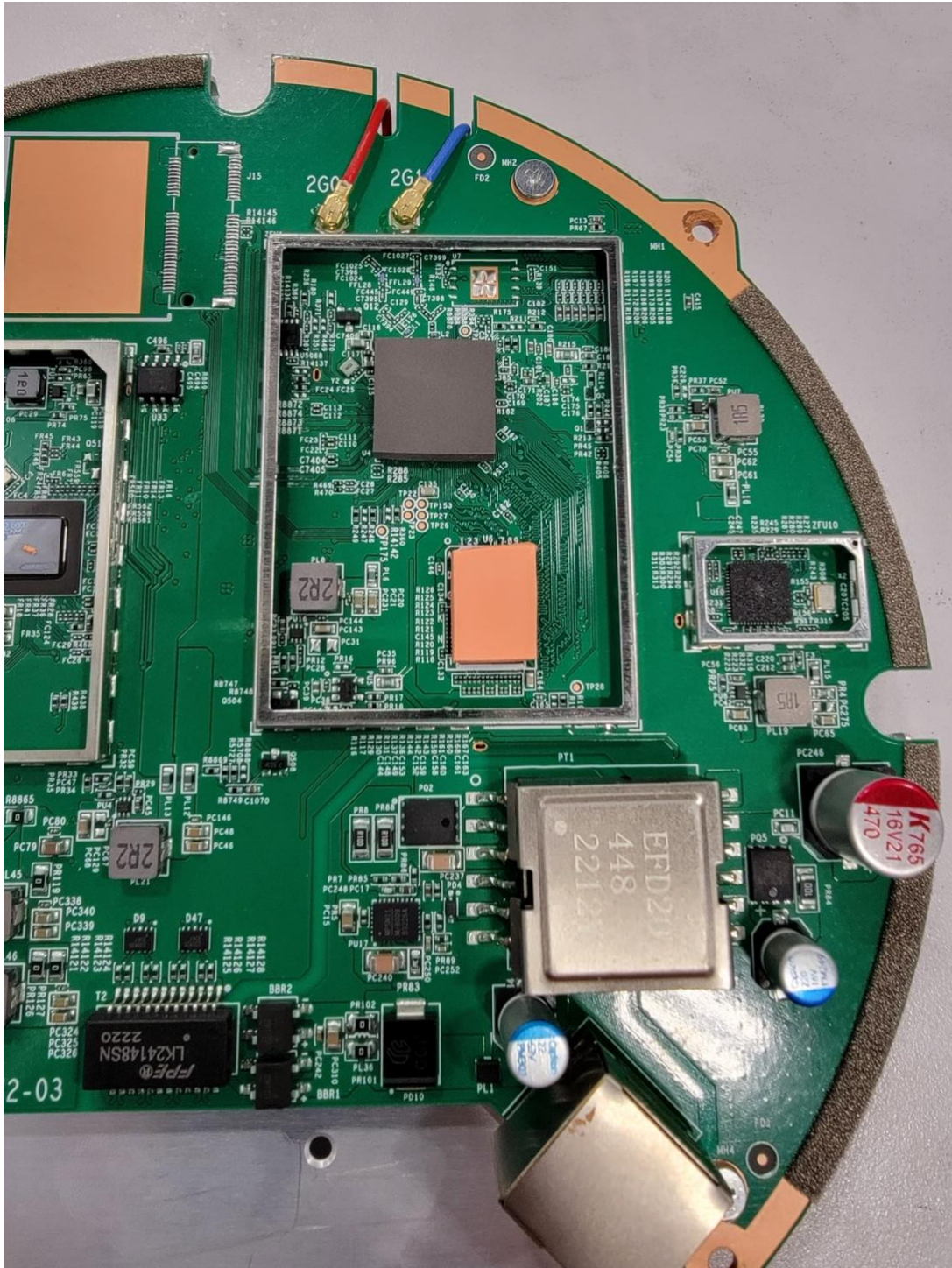
Photograph 10: PCB Closeup left side
