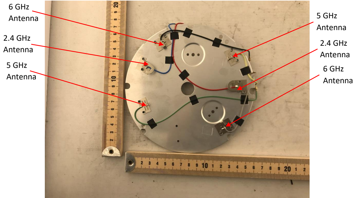
Photograph 7: Top View of the Antenna Configuration
