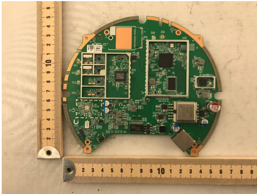
Photograph 5: Top View of the PCB with Cans Off
