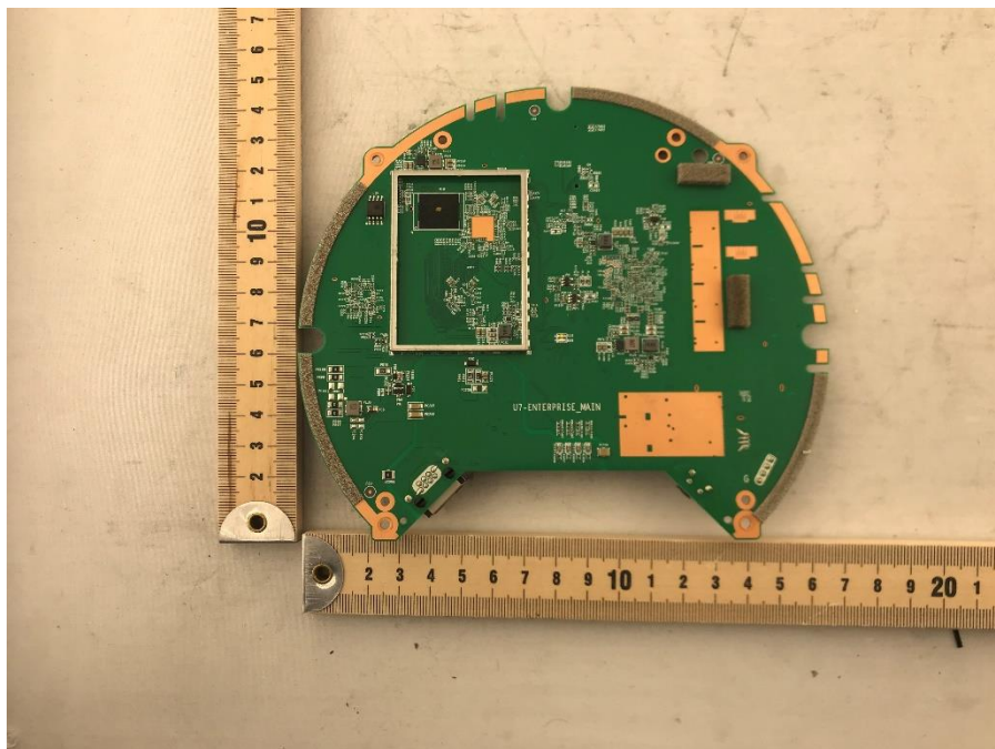
Photograph 6: Bottom View of the PCB
