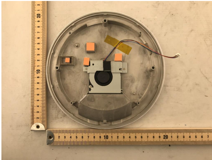
Photograph 3: Bottom Base Internal View of DUT with PCB Off
