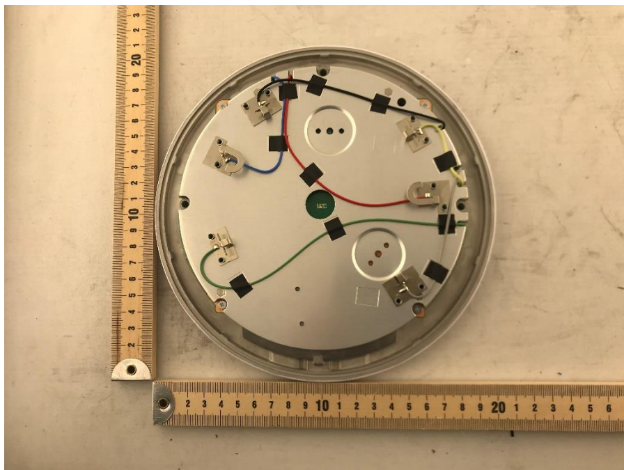
Photograph 2: Internal View of DUT With Front Cover Removed
