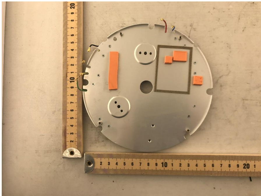
Photograph 8: Bottom View of the Antenna Configuration
