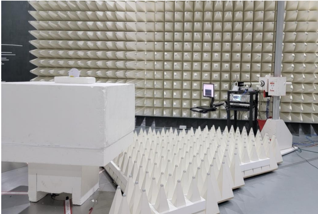
Photograph 3: View Test Set Up Radiated Emissions 17 – 40 GHz
