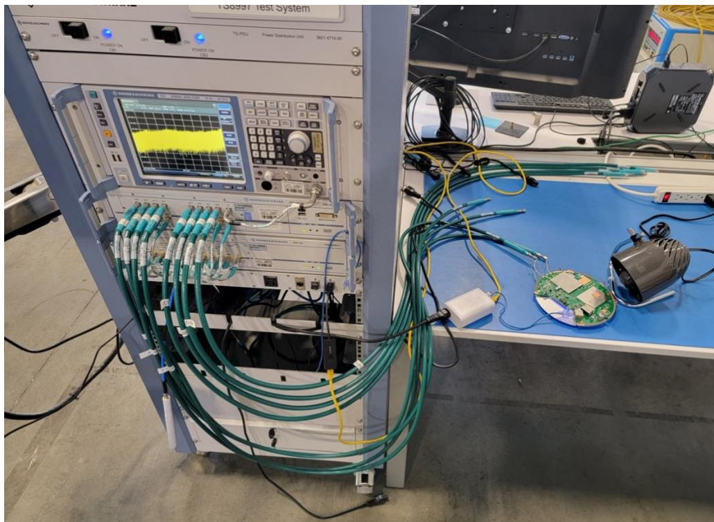
Photograph 4: View Test Set Up RF Conducted
