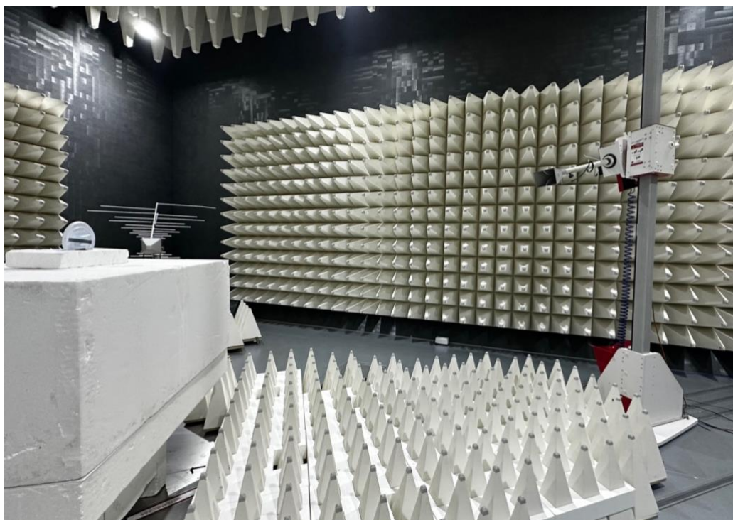
Photograph 2: View Test Set Up Radiated Emissions 1 – 17 GHz
