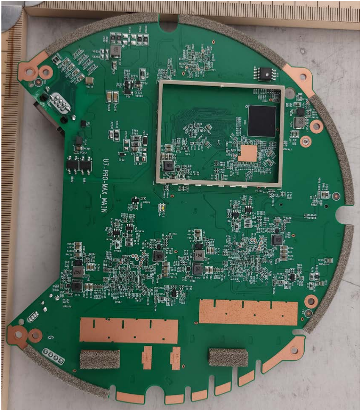
Photograph 5: Internal View Back Main PCB
