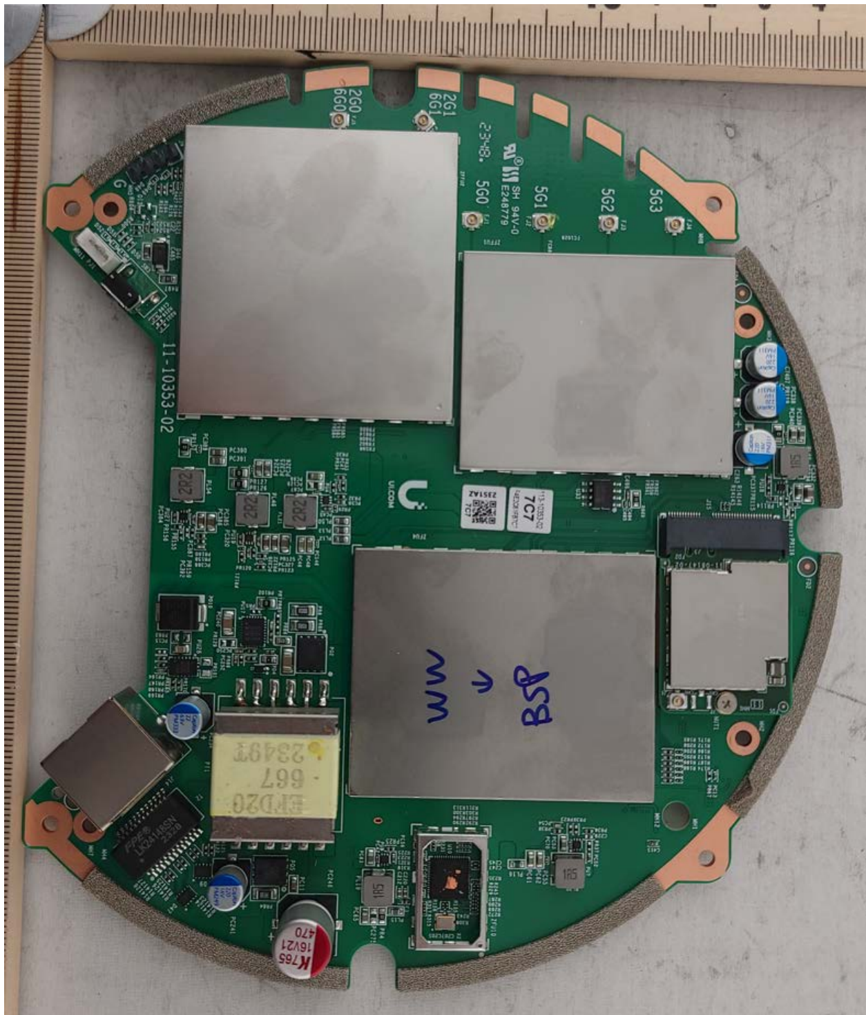
Photograph 3: Internal View Front Main PCB Cans One
