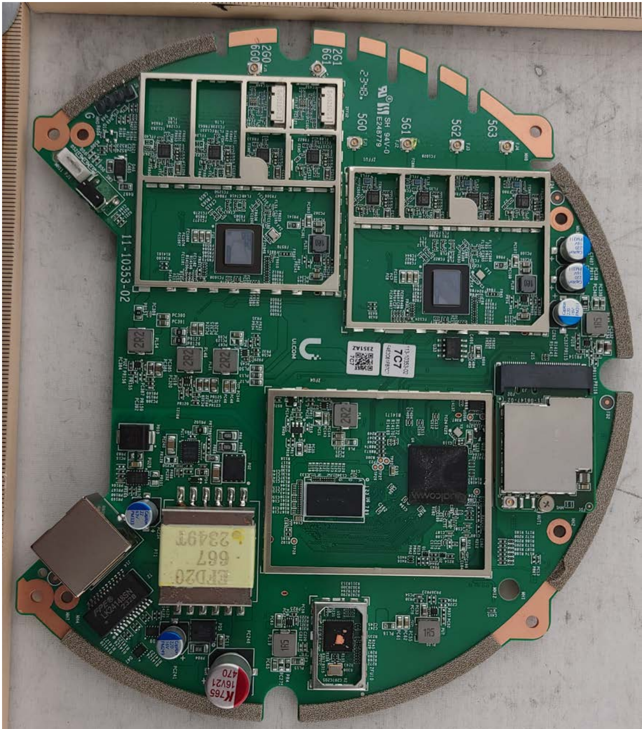
Photograph 4: Internal View Front Main PCB Cans Off
