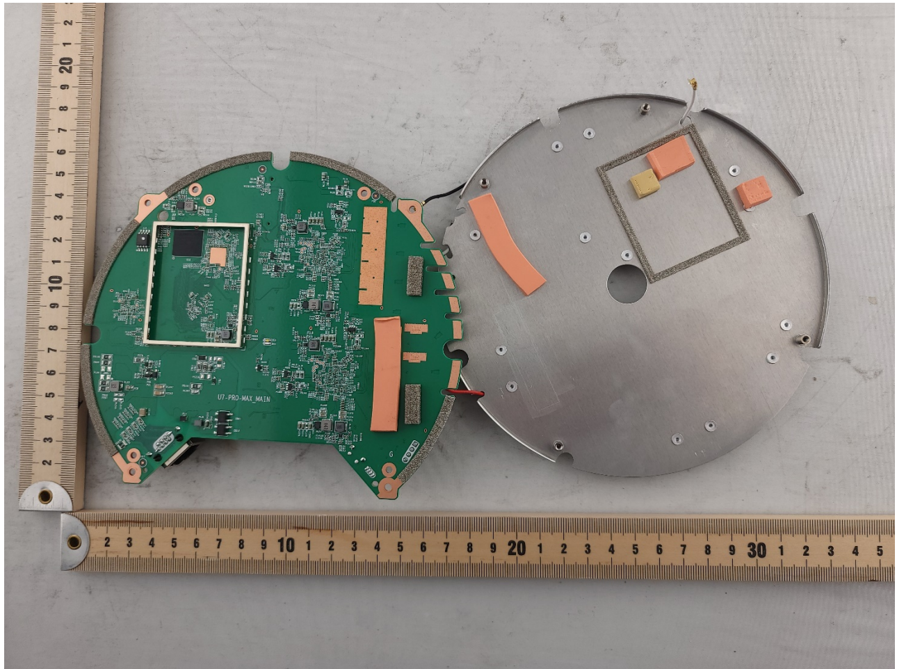
Photograph 2: Internal View Back Antenna/Main PCB Separated
