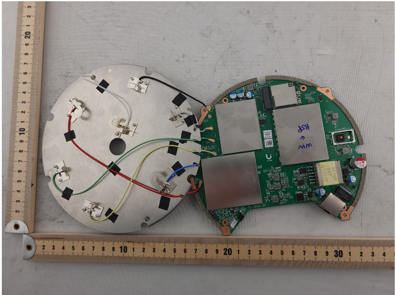
Photograph 1: Internal View Front Antenna/Main PCB Separated
