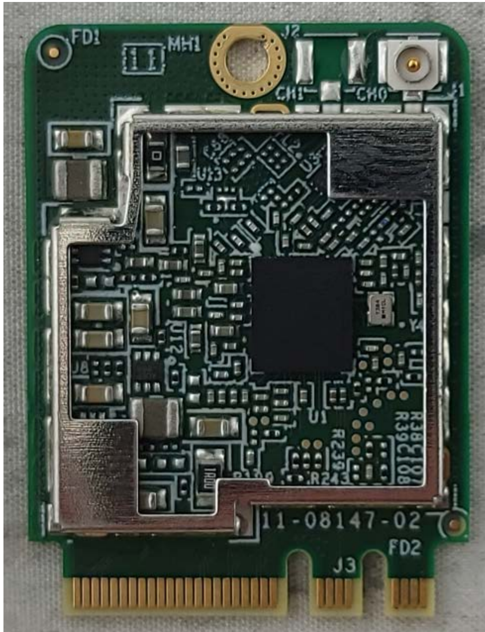
Photograph 3: Internal View Front Scanner PCB Can Off
