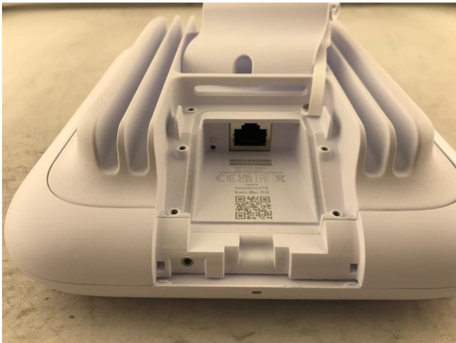
Photograph 8: Close-up of DUT Port
