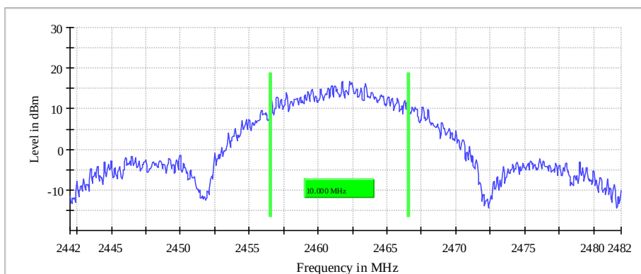
6 dB Bandwidth
