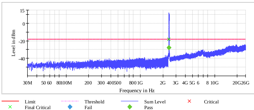
Spurious
