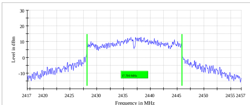
6 dB Bandwidth
