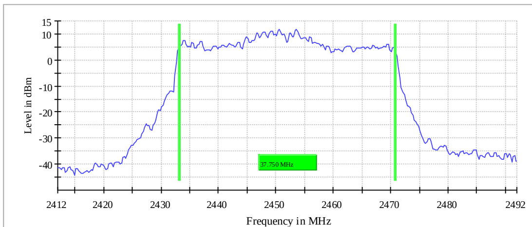
Bandwidth
