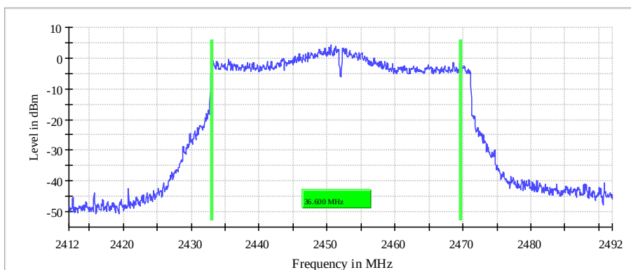
6 dB Bandwidth
